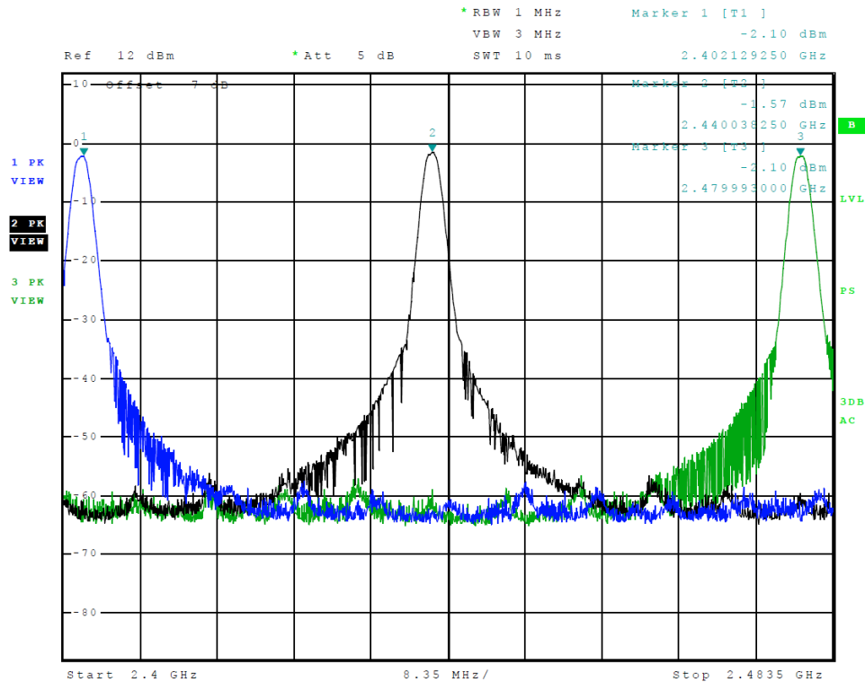
Figure 19 Plot of Transmitter Emissions (Operation in 2402-2480 MHz, BLE 0x55)
