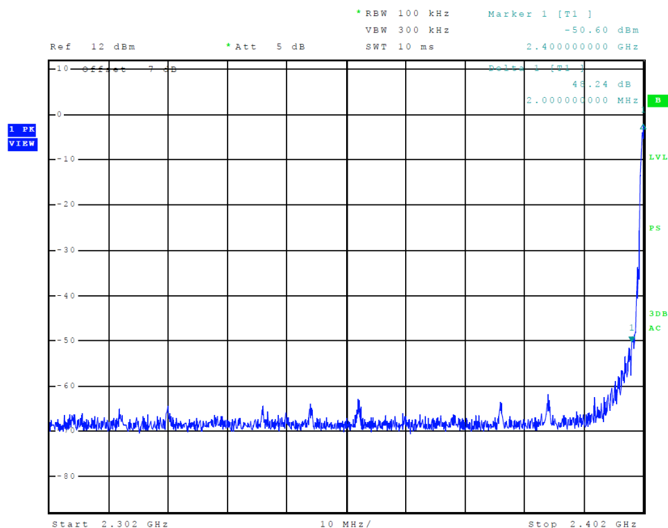
Figure 17 Plot of Transmitter Emissions (Low Band Edge, BLE 0x0F)
