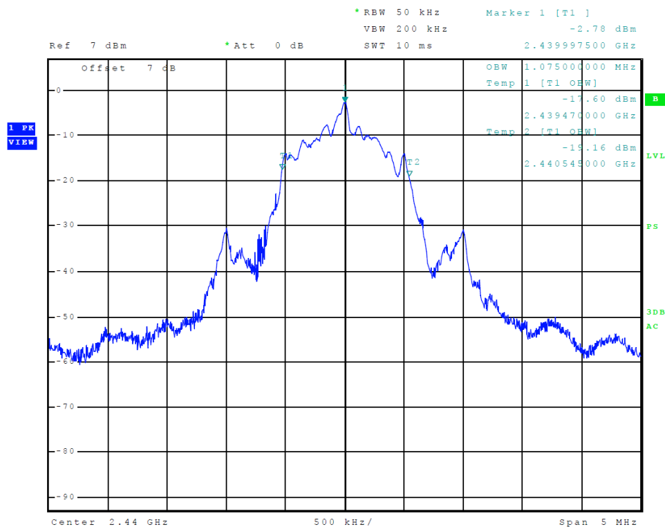
Figure 20 Plot of Transmitter Emissions (99% Occupied Bandwidth, BLE 0x55)
