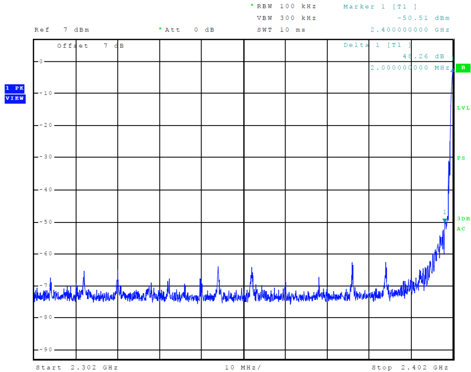
Figure 21 Plot of Transmitter Emissions (Low Band Edge, BLE 0x55)
