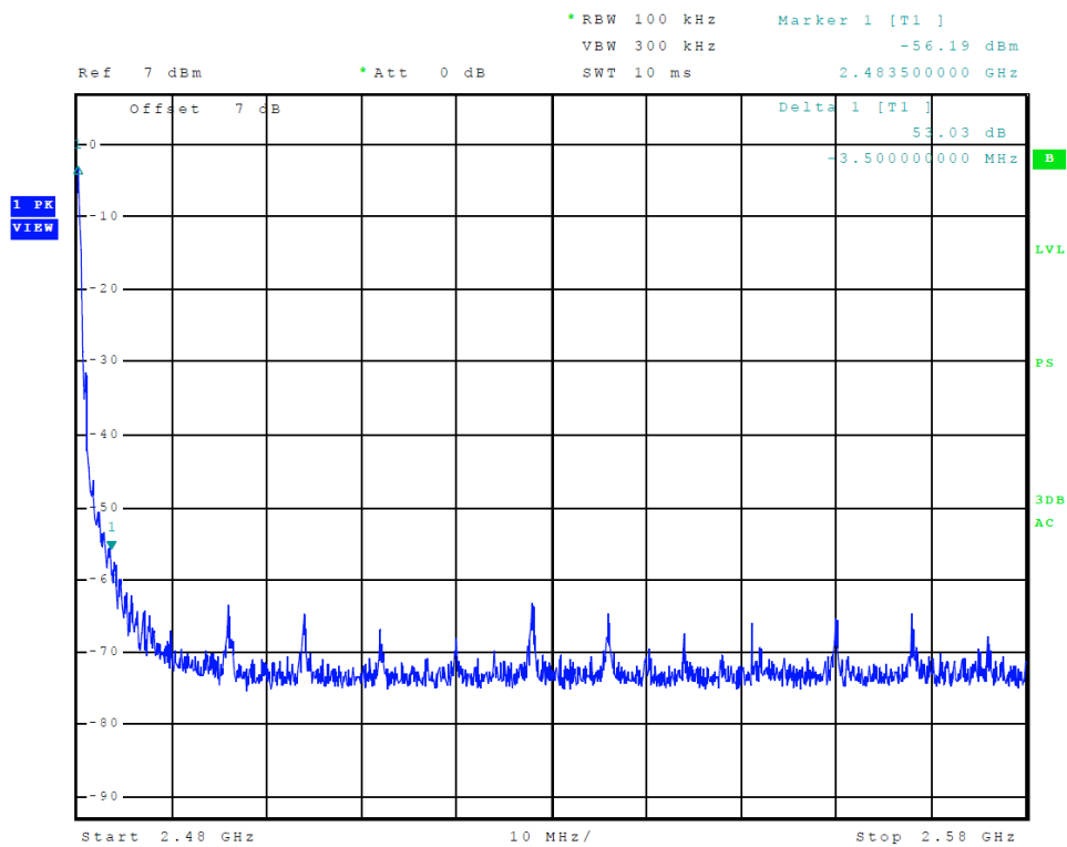
Figure 22 Plot of Transmitter Emissions (High Band Edge, BLE 0x55)
