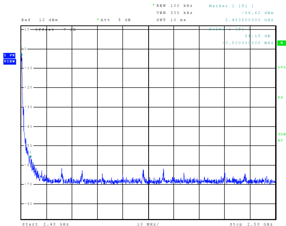
Figure 18 Plot of Transmitter Emissions (High Band Edge, BLE 0x0F)
