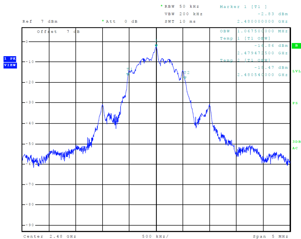
Figure 16 Plot of Transmitter Emissions (99% Occupied Bandwidth, BLE 0x0F)
