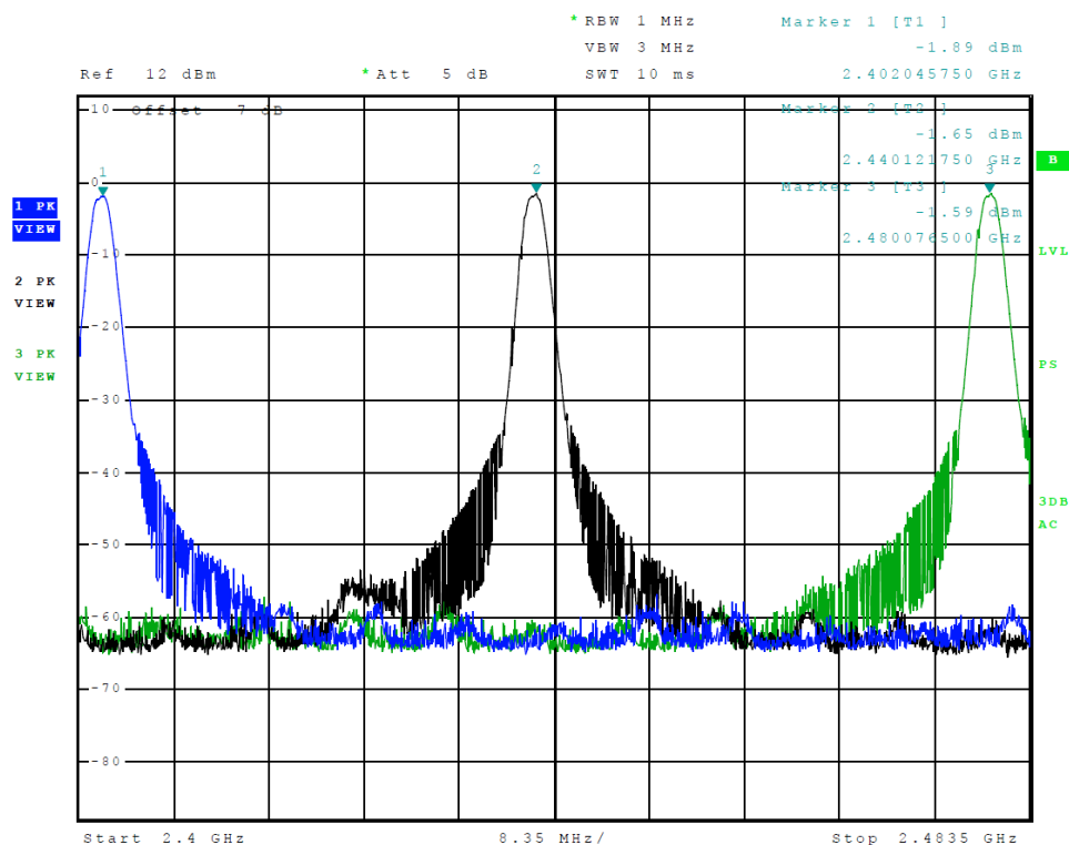
Figure 15 Plot of Transmitter Emissions (Operation in 2402-2480 MHz, BLE 0x0F)
