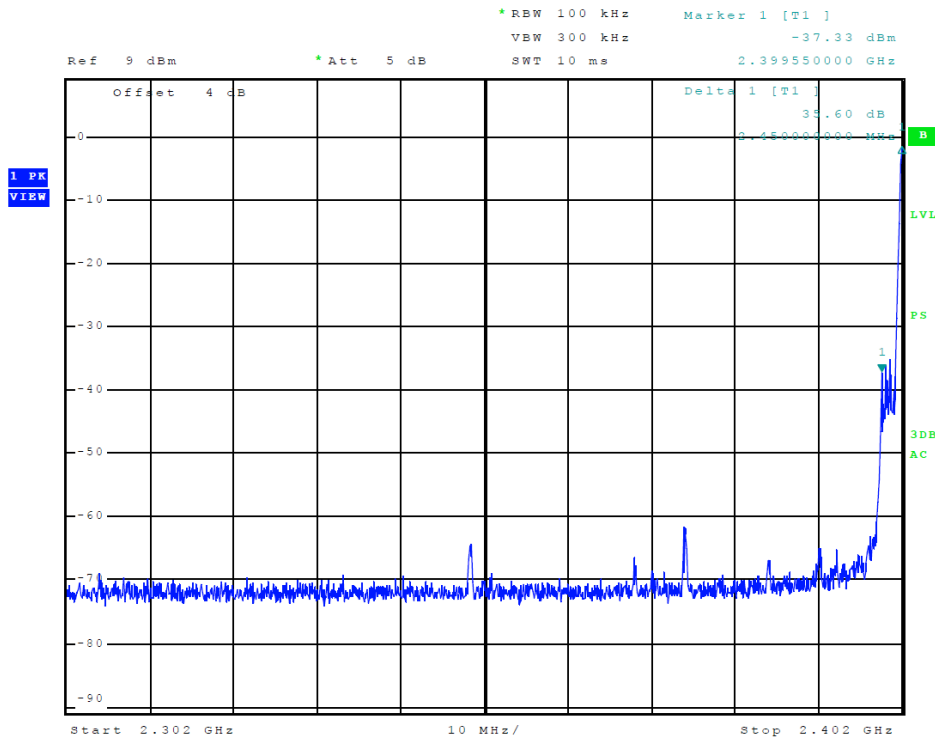
Figure 7 Plot of Transmitter Emissions (Low Band Edge, 3EDR)
