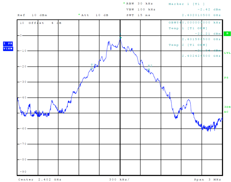
Figure 2 Plot of Transmitter Emissions (99% Occupied Bandwidth, 2EDR)
