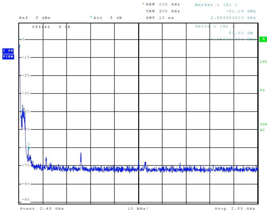
Figure 8 Plot of Transmitter Emissions (High Band Edge, 3EDR)
