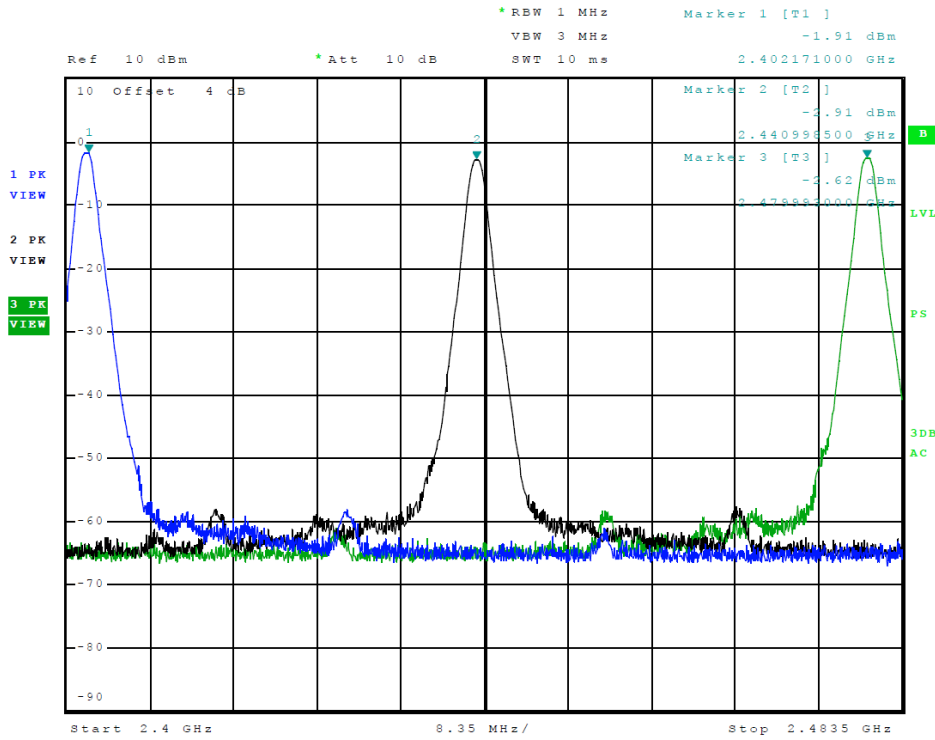
Figure 5 Plot of Transmitter Emissions (Operation in 2402-2480 MHz, 3EDR)
