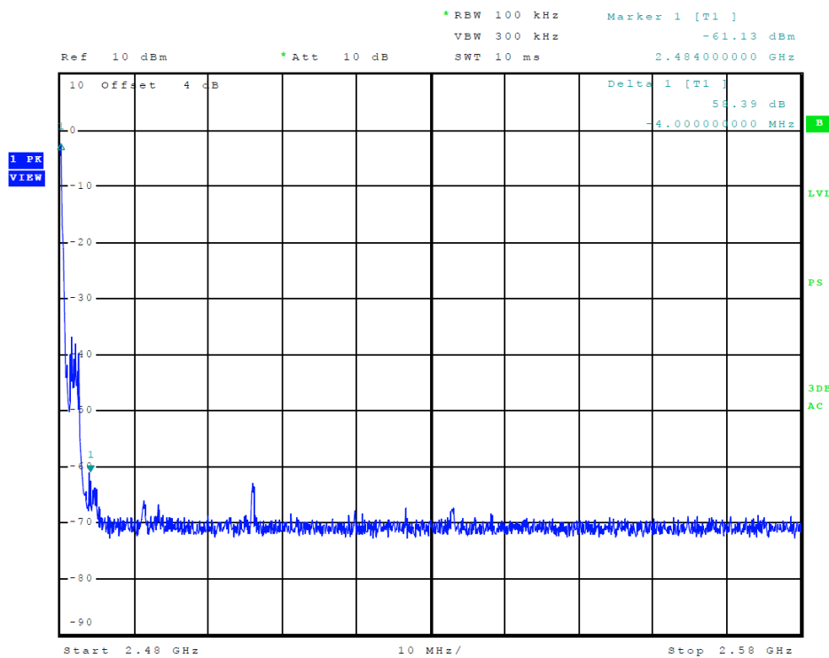
Figure 4 Plot of Transmitter Emissions (High Band Edge, 2EDR)
