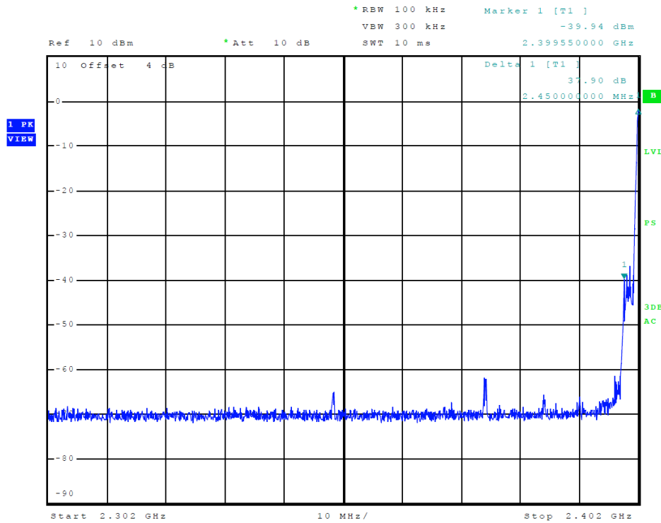
Figure 3 Plot of Transmitter Emissions (Low Band Edge, 2EDR)
