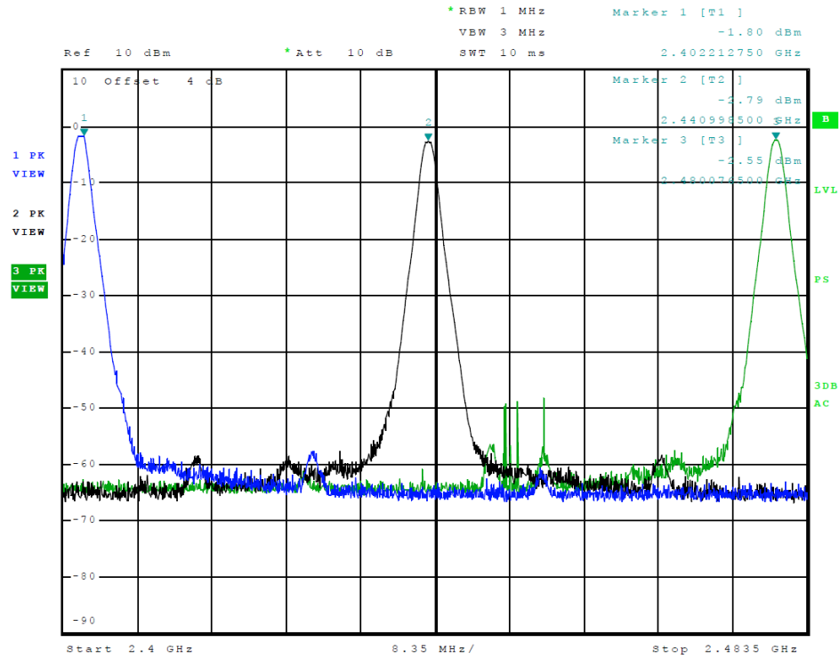
Figure 1 Plot of Transmitter Emissions (Operation in 2402-2480 MHz, 2EDR)
