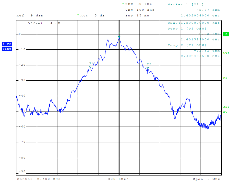
Figure 6 Plot of Transmitter Emissions (99% Occupied Bandwidth, 3EDR)
