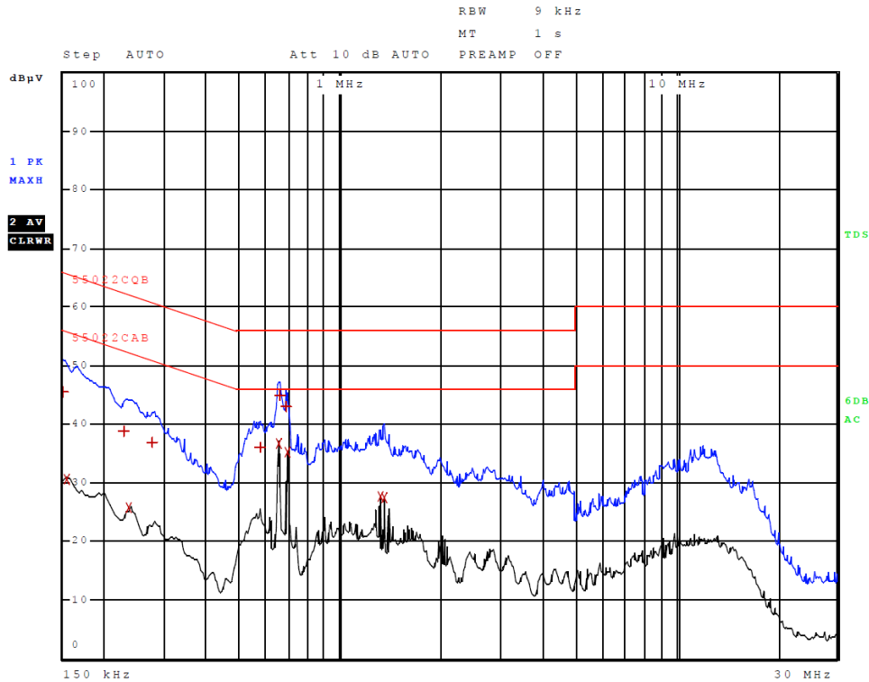
Figure 2 AC Line Conducted emissions of EUT line 2 (#3, EUT – 320-00096-00)
