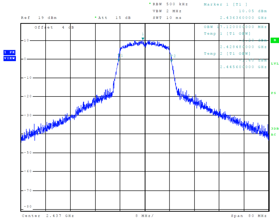
Figure 17 Plot of Transmitter 99% Occupied Bandwidth (802.11 g-mode)
