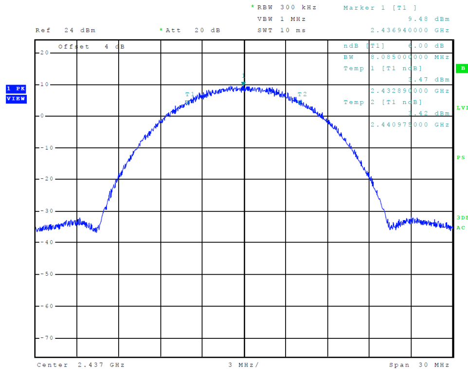
Figure 14 Plot of Transmitter 6-dB Occupied Bandwidth (802.11 b-mode)
