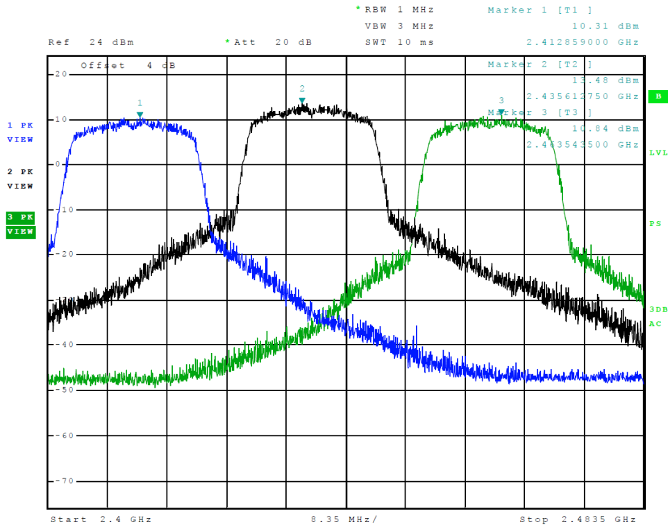
Figure 7 Plot of Transmitter Emissions in Operational Frequency (802.11 n-Mode)
