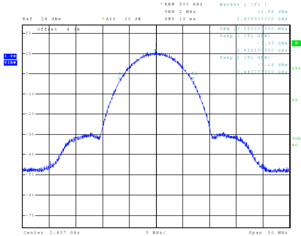
Figure 15 Plot of Transmitter 99% Occupied Bandwidth (802.11 b-mode)
