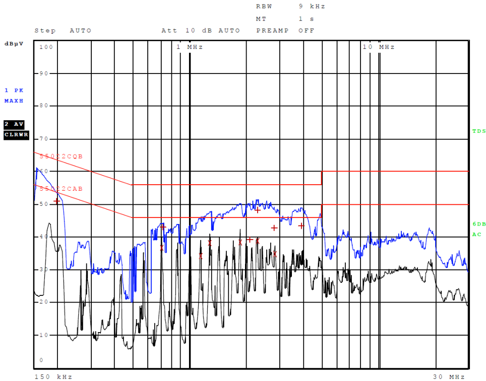
Figure 3 AC Line Conducted emissions of EUT line 1 (#4, EUT – CPU)
