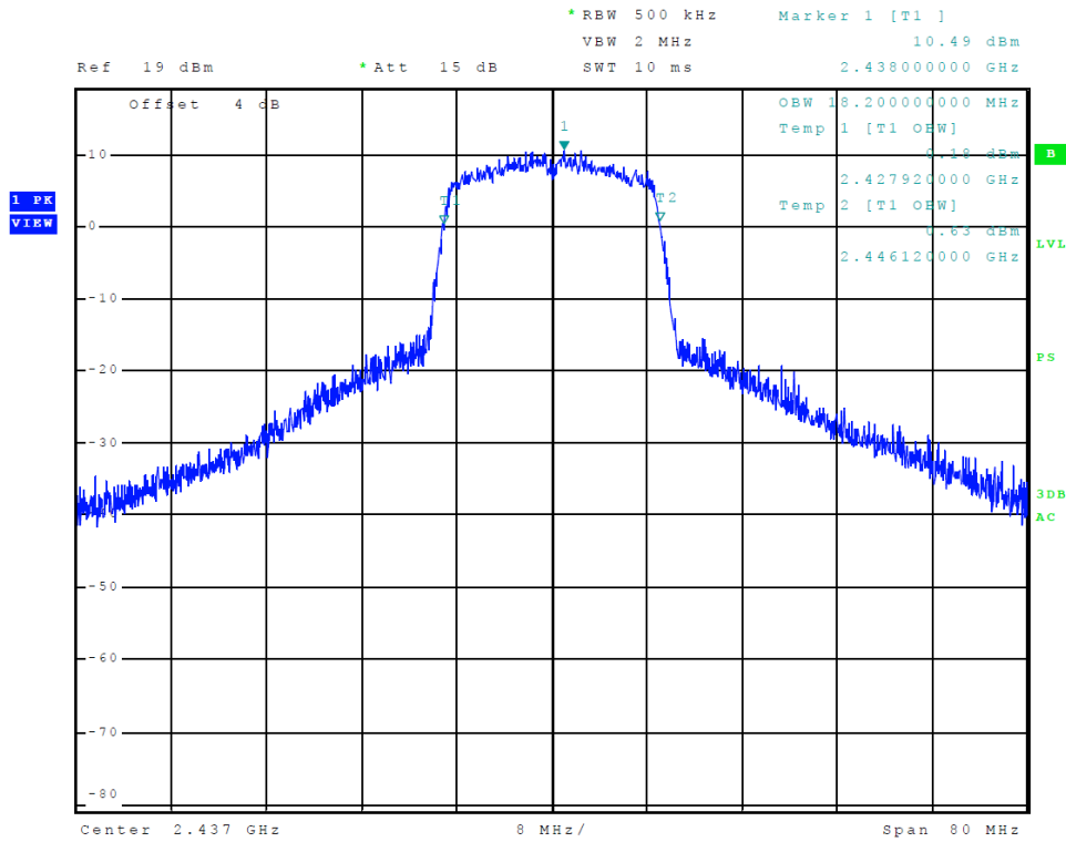
Figure 19 Plot of Transmitter 99% Occupied Bandwidth (802.11 n-mode)
