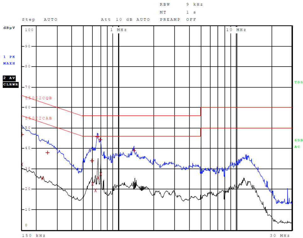
Figure 1 AC Line Conducted emissions of EUT line 1 (#3, EUT – 320-00096-00)
