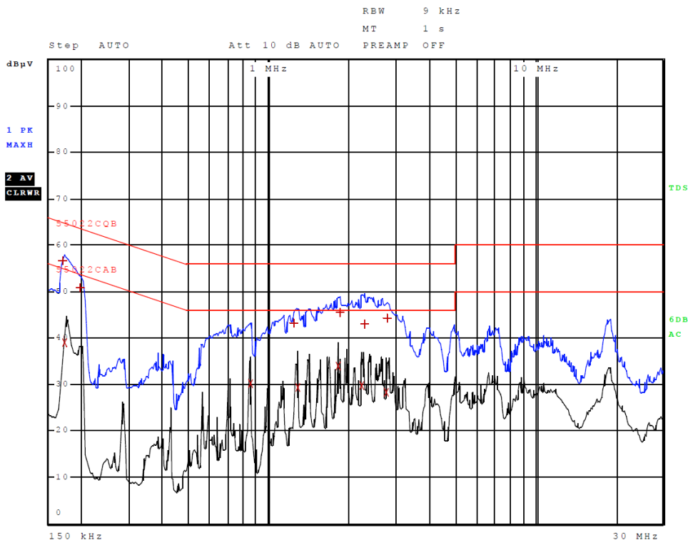
Figure 4 AC Line Conducted emissions of EUT line 2 (#4, EUT – CPU)
