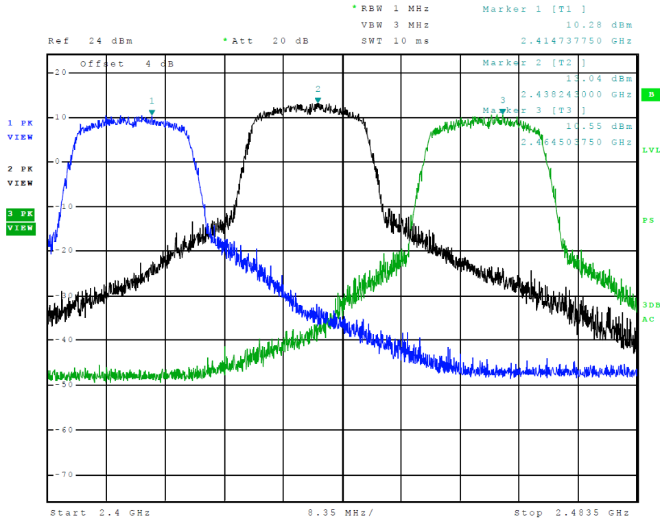
Figure 6 Plot of Transmitter Emissions in Operational Frequency (802.11 g-Mode)
