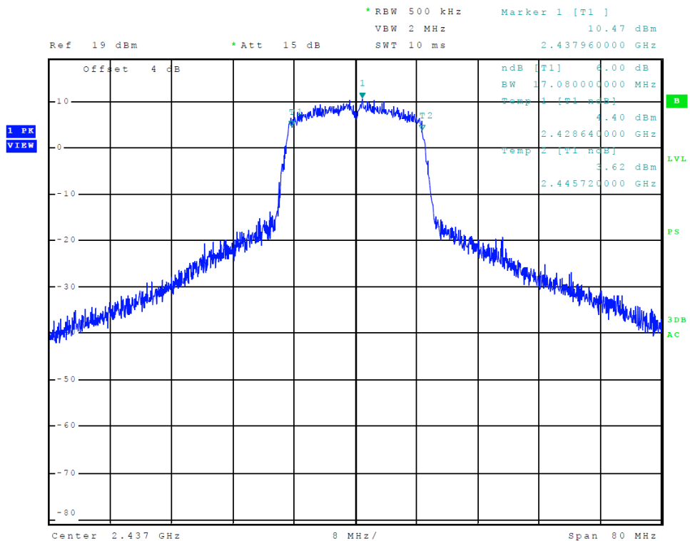
Figure 18 Plot of Transmitter 6-dB Occupied Bandwidth (802.11 n-mode)
