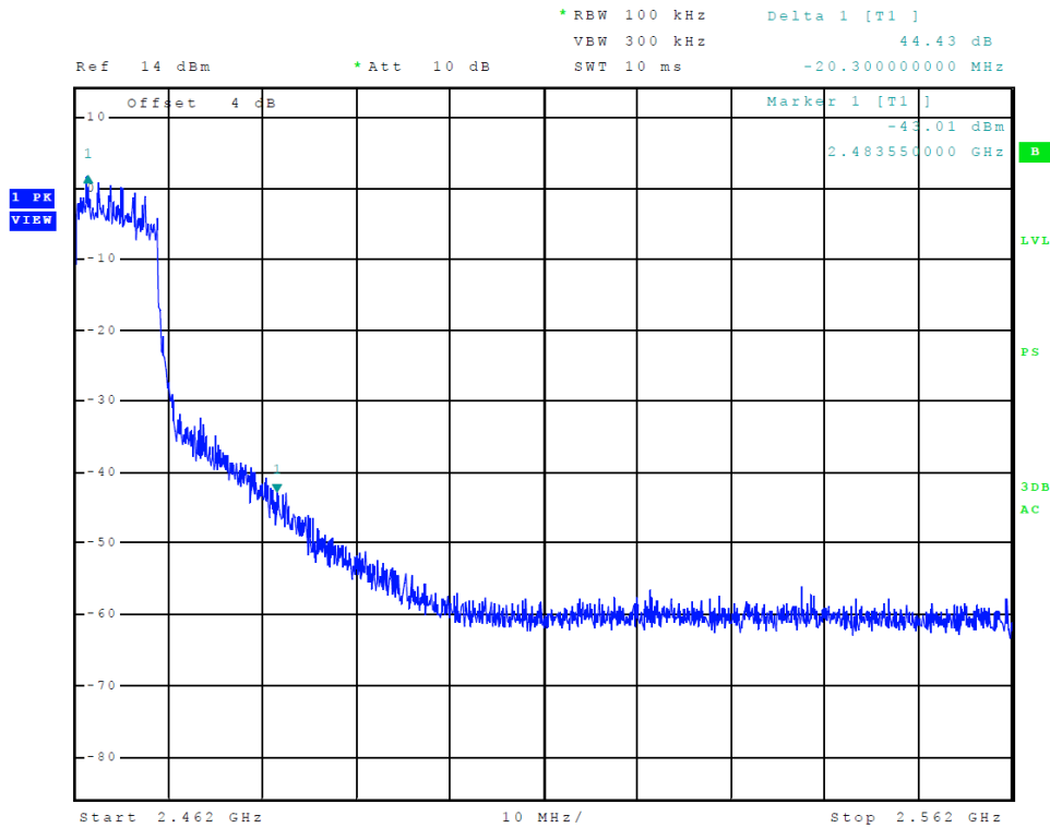
Figure 13 Plot of Upper Band Edge (802.11 n-mode)
