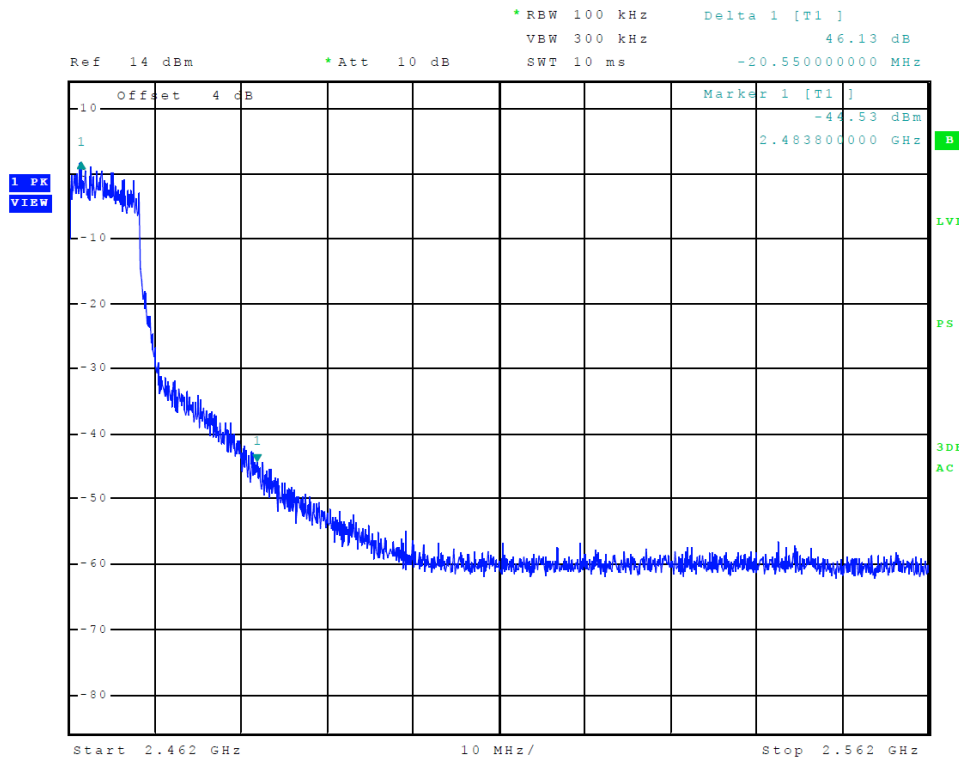
Figure 12 Plot of Upper Band Edge (802.11 g-mode)
