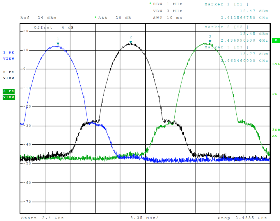
Figure 5 Plot of Transmitter Emissions in Operational Frequency (802.11 b-Mode)
