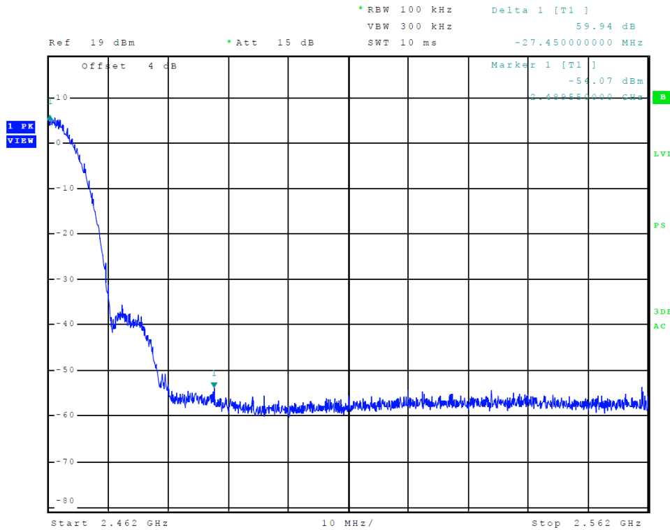
Figure 11 Plot of Upper Band Edge (802.11 b-mode)
