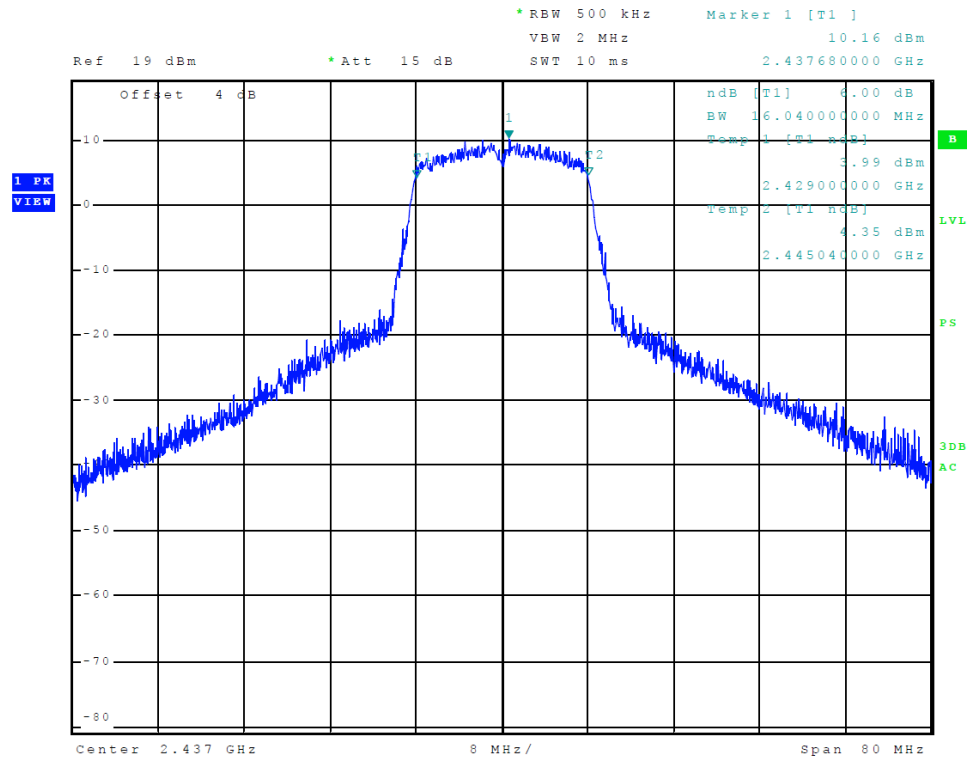
Figure 16 Plot of Transmitter 6-dB Occupied Bandwidth (802.11 g-mode)
