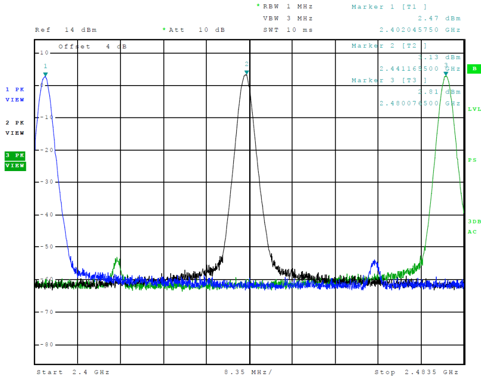
Figure 17 Plot of Transmitter Emissions (Operation in 2402-2480 MHz, 3EDR)
