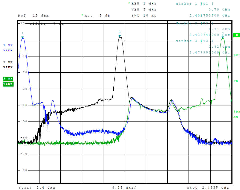
Figure 5 Plot of Transmitter Emissions (Operation in 2402-2479 MHz, BLE)
