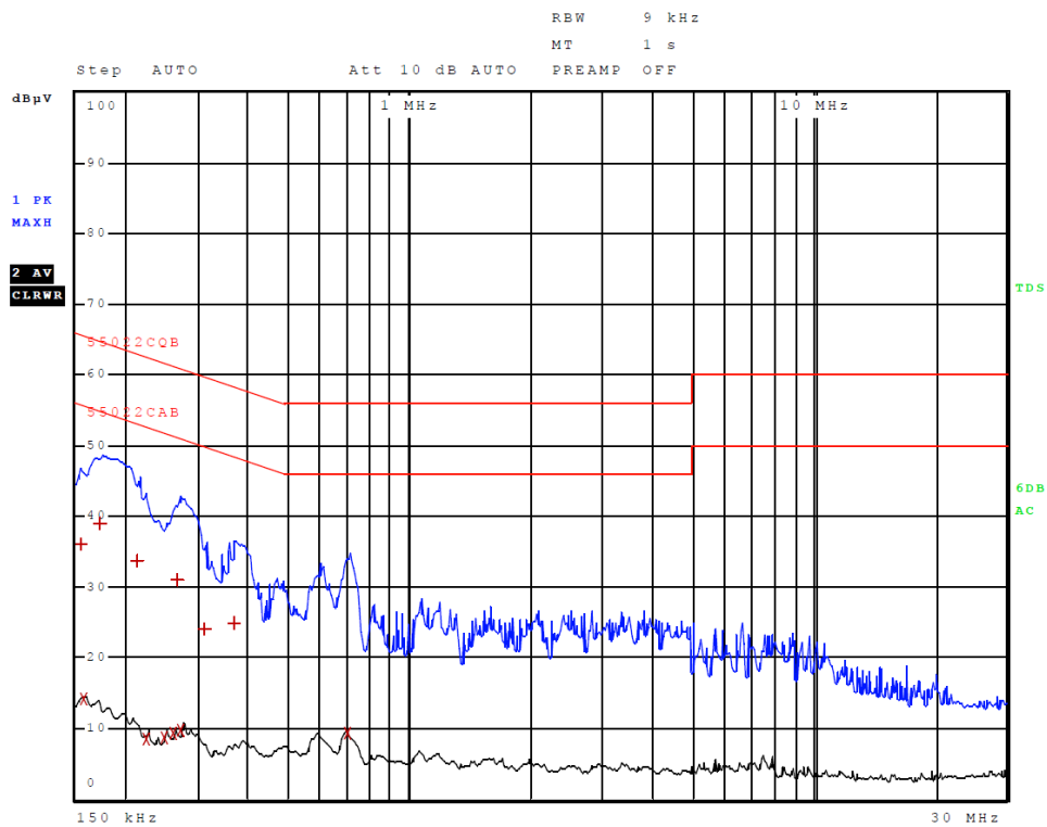
Figure 4 AC Line Conducted emissions of EUT line 2 (#3, EUT – 320-00087-00)
