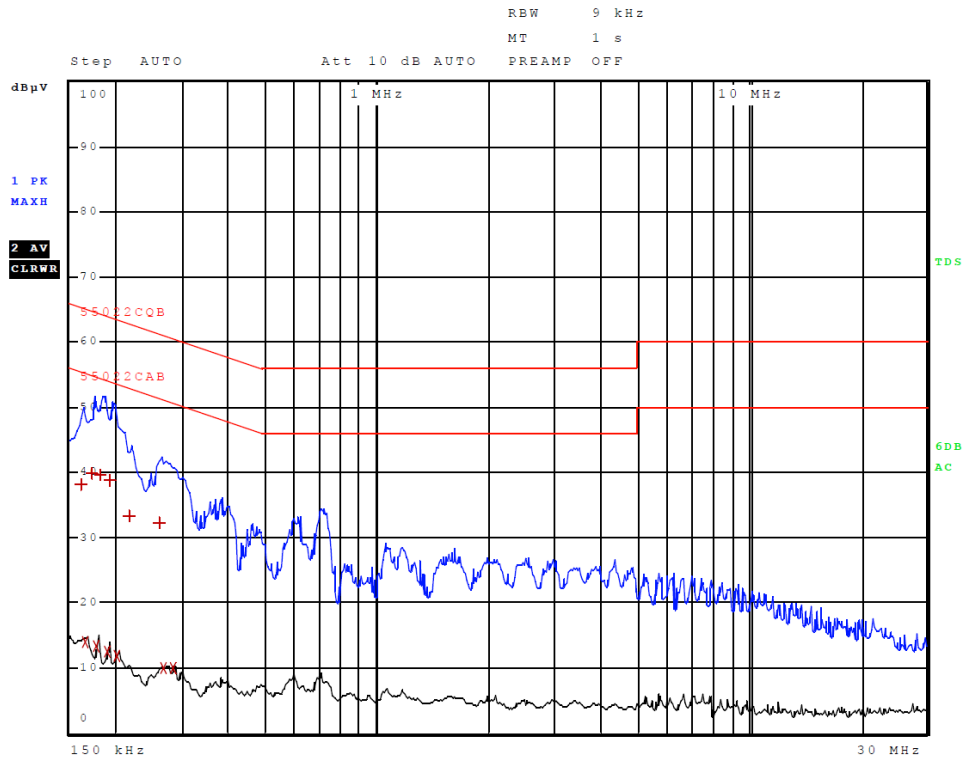
Figure 3 AC Line Conducted emissions of EUT line 1 (#3, EUT – 320-00087-00)
