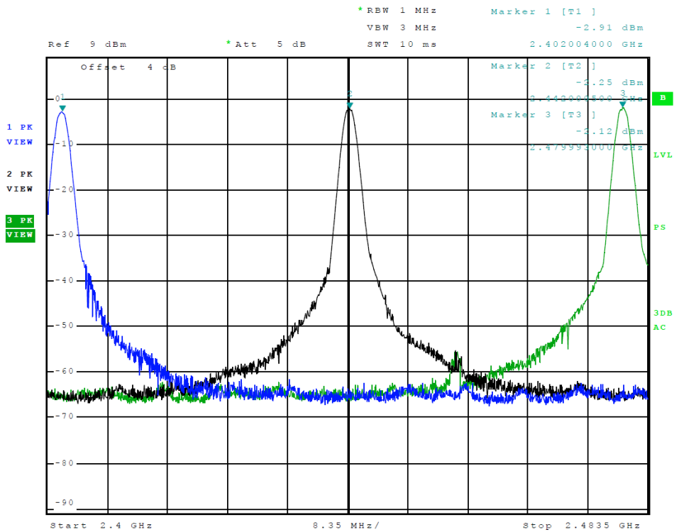
Figure 8 Plot of Transmitter Emissions (Operation in 2402-2480 MHz, mode 2)
