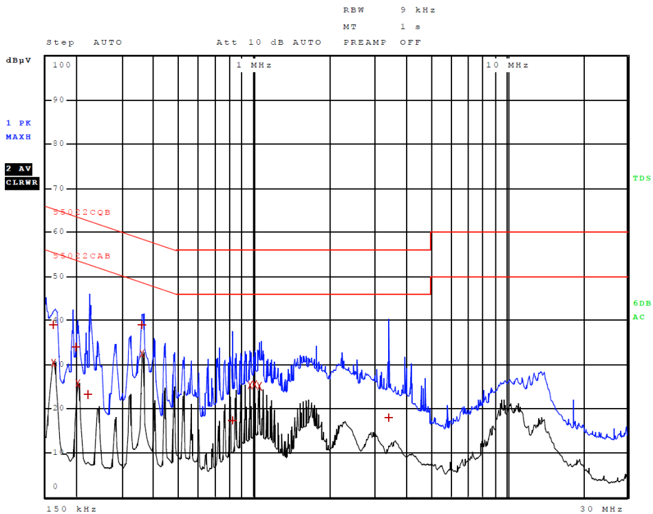
Figure 4 AC Line Conducted emissions of EUT line 2 (#3, EUT -AC Adapter, 362-00072-00)
