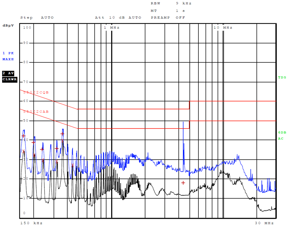
Figure 3 AC Line Conducted emissions of EUT line 1 (#3, EUT -AC Adapter, 362-00072-00)
