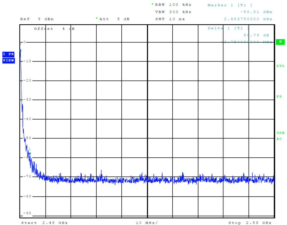
Figure 14 Plot of Transmitter Emissions (High Band Edge, mode 2)
