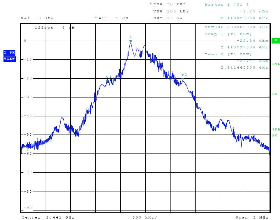
Figure 9 Plot of Transmitter Emissions (99% Occupied Bandwidth, mode 1)
