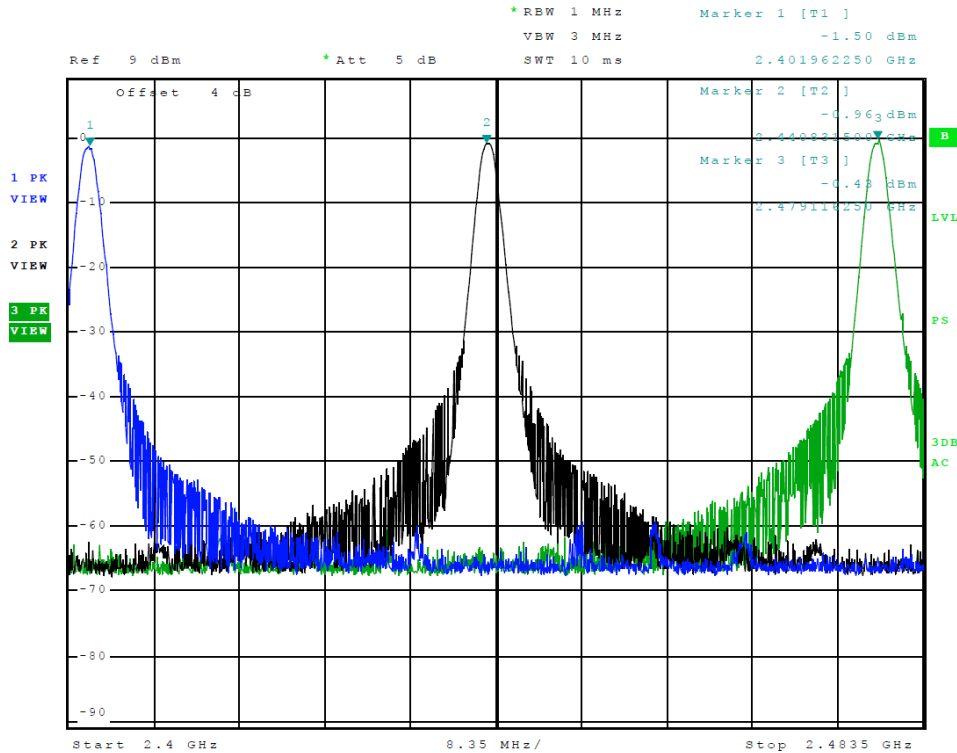
Figure 7 Plot of Transmitter Emissions (Operation in 2402-2479 MHz, node 1)
