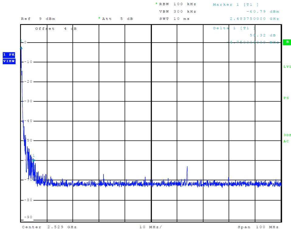
Figure 13 Plot of Transmitter Emissions (High Band Edge, mode 1)
