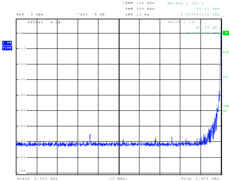
Figure 11 Plot of Transmitter Emissions (Low Band Edge, mode 1)
