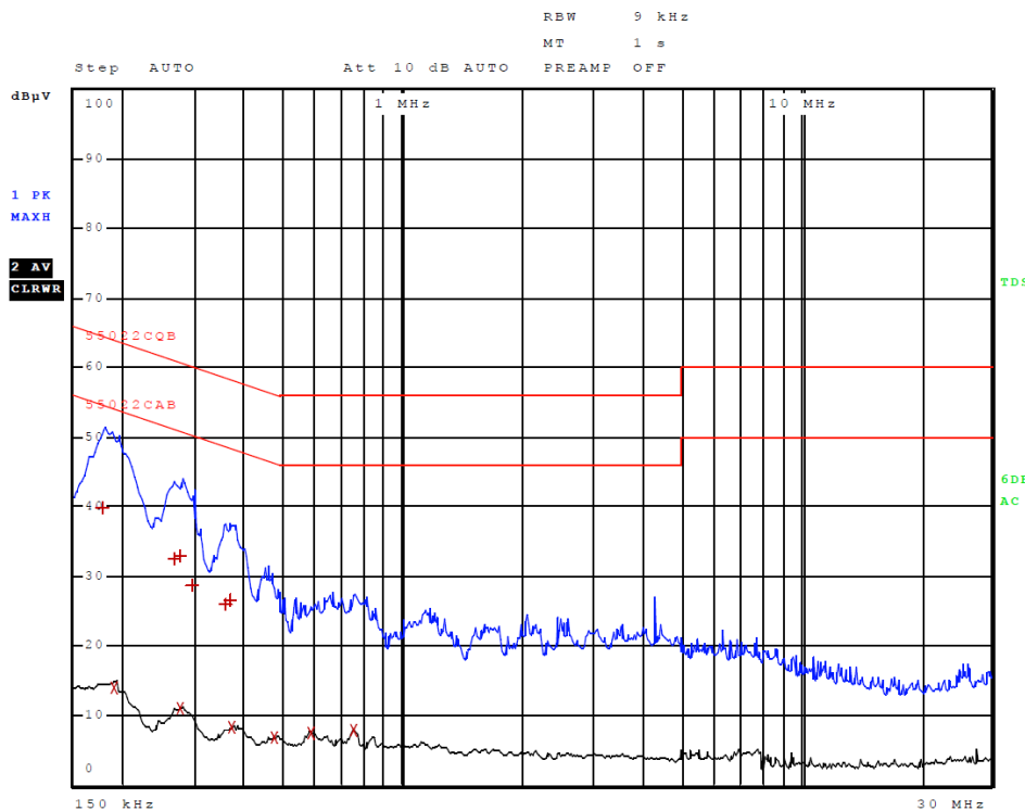
Figure 6 AC Line Conducted emissions of EUT line 2 (#4, EUT -AC Adapter, 362-00087-00)
