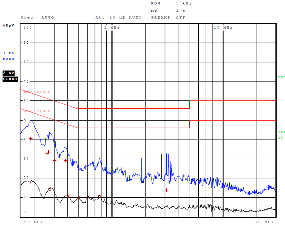
Figure 5 AC Line Conducted emissions of EUT line 1 (#4, EUT -AC Adapter, 362-00087-00)
