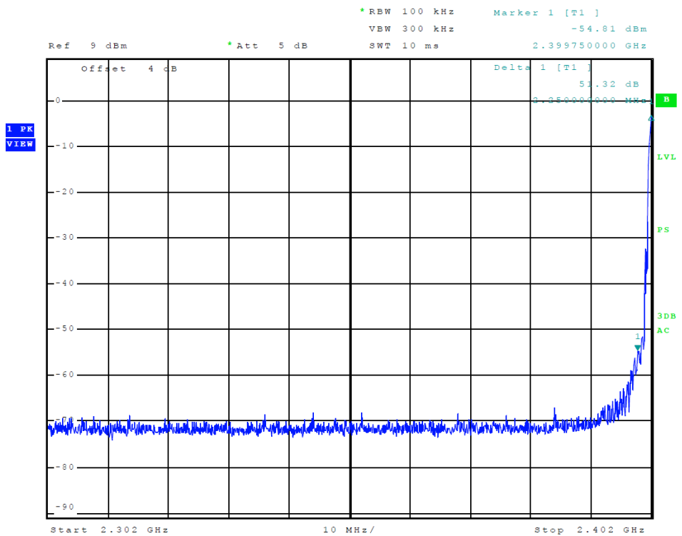
Figure 12 Plot of Transmitter Emissions (Low Band Edge, mode 2)
