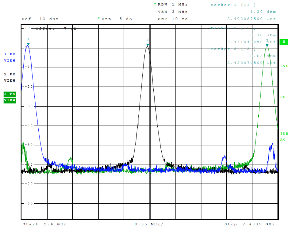
Figure 11 Plot of Transmitter Emissions (Operation in 2402-2480 MHz, BT EDR2)
