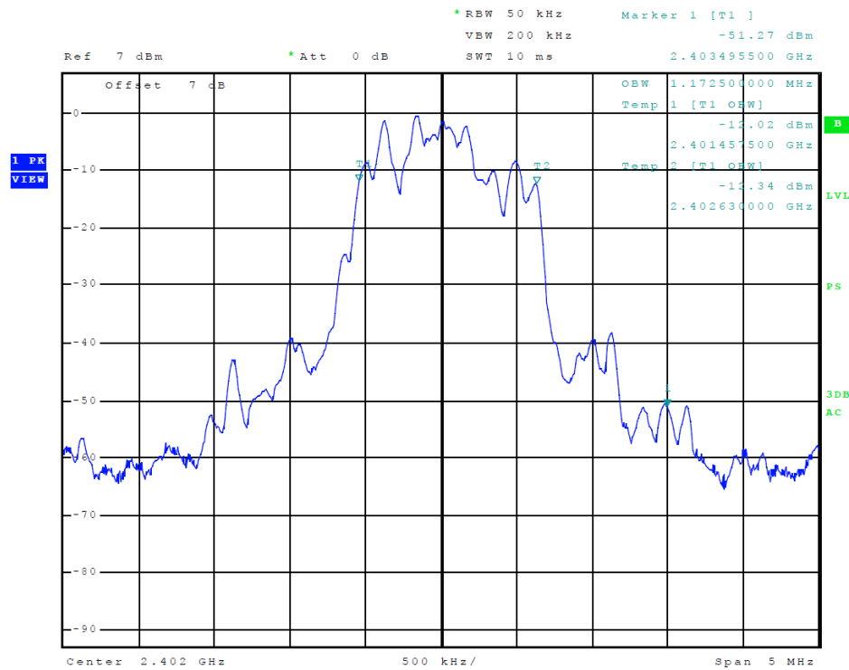
Figure 12 Plot of Transmitter Emissions (99% Occupied Bandwidth, BT EDR2)
