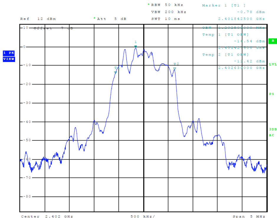
Figure 16 Plot of Transmitter Emissions (99% Occupied Bandwidth, BT EDR3)
