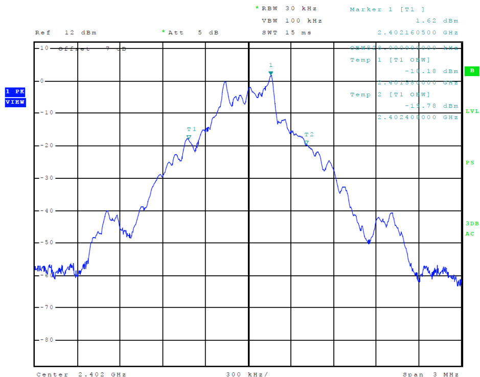
Figure 6 Plot of Transmitter Emissions (99% Occupied Bandwidth, ANT)
