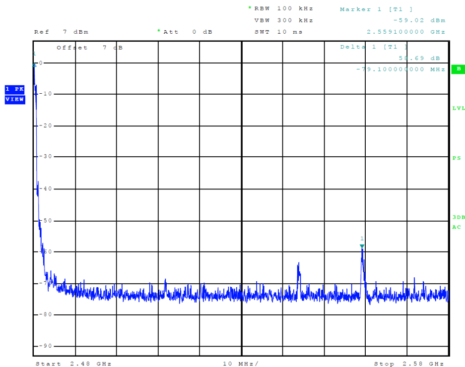
Figure 14 Plot of Transmitter Emissions (High Band Edge, BT EDR2)
