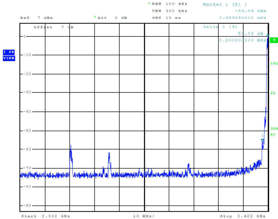
Figure 13 Plot of Transmitter Emissions (Low Band Edge, BT EDR2)
