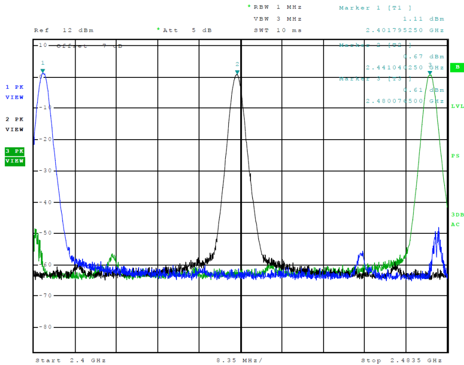
Figure 15 Plot of Transmitter Emissions (Operation in 2402-2480 MHz, BT EDR3)
