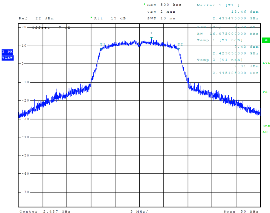
Figure 18 Plot of Transmitter 6-dB Occupied Bandwidth (802.11 g-mode)
