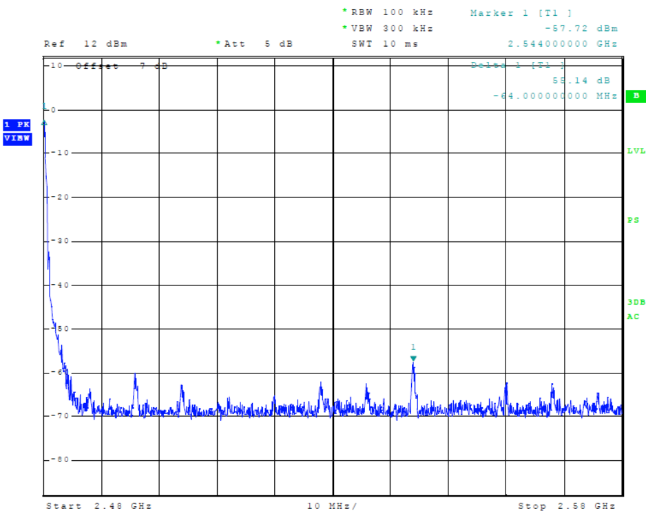
Figure 20 Plot of Transmitter Emissions (High Band Edge, BLE 0x55)
