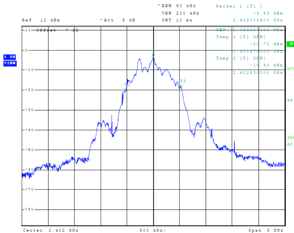
Figure 18 Plot of Transmitter Emissions (99% Occupied Bandwidth, BLE 0x55)
