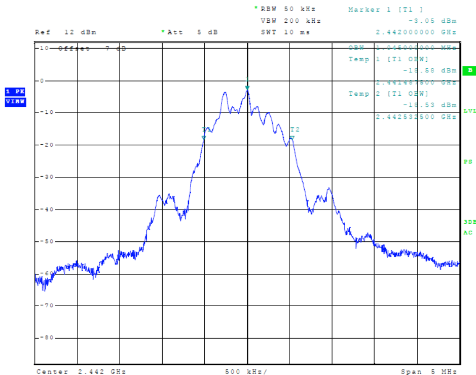
Figure 10 Plot of Transmitter Emissions (99% Occupied Bandwidth, PRB29)
