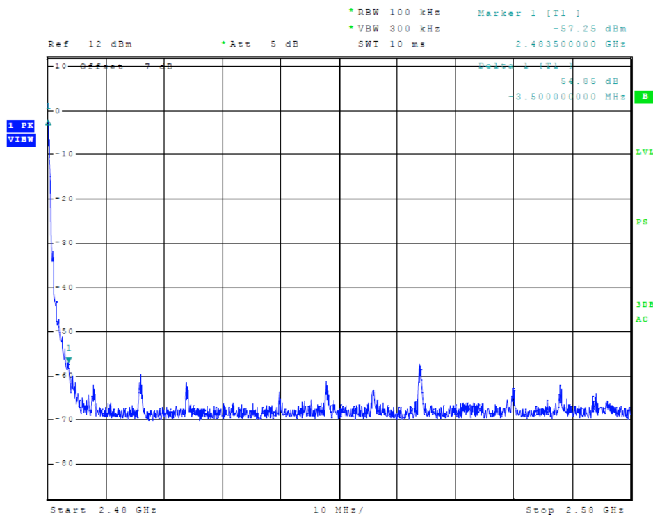
Figure 12 Plot of Transmitter Emissions (High Band Edge, PRB29)
