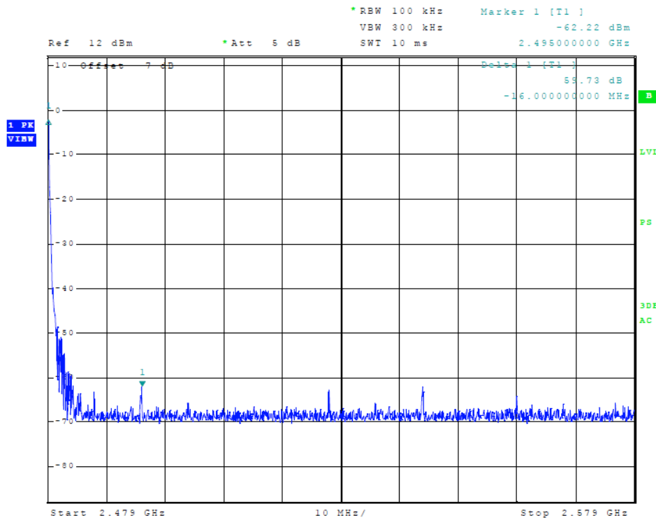
Figure 8 Plot of Transmitter Emissions (High Band Edge, GFSK)
