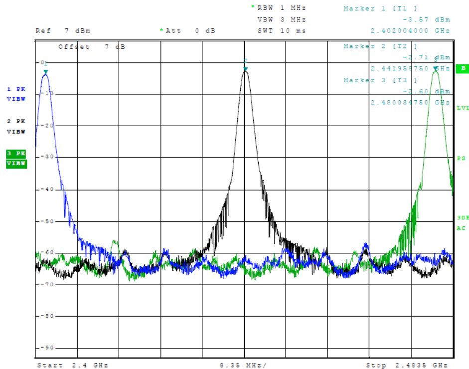
Figure 13 Plot of Transmitter Emissions (Operation in 2402-2480 MHz, BLE 0x0F)
