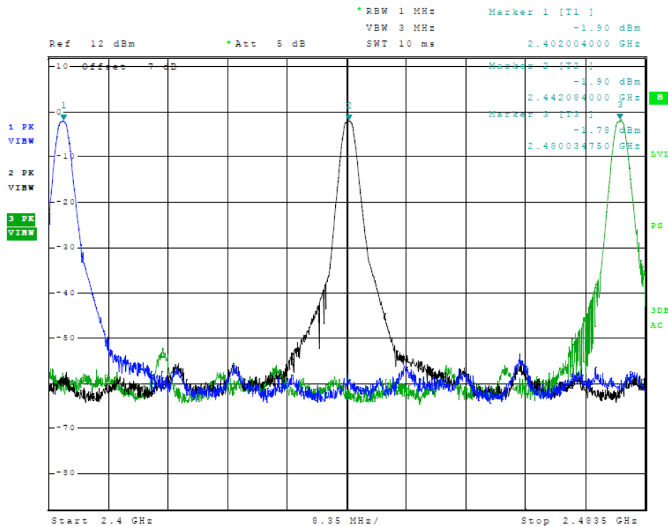
Figure 9 Plot of Transmitter Emissions (Operation in 2402-2480 MHz, PRB29)
