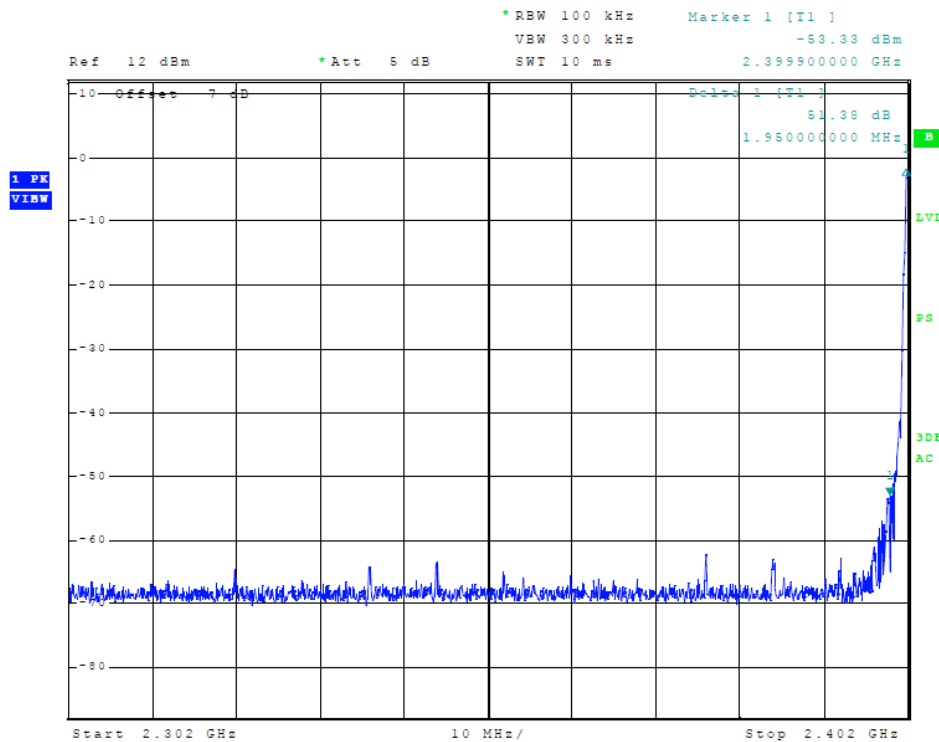
Figure 7 Plot of Transmitter Emissions (Low Band Edge, GFSK)
