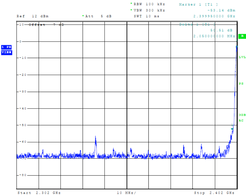
Figure 19 Plot of Transmitter Emissions (Low Band Edge, BLE 0x55)
