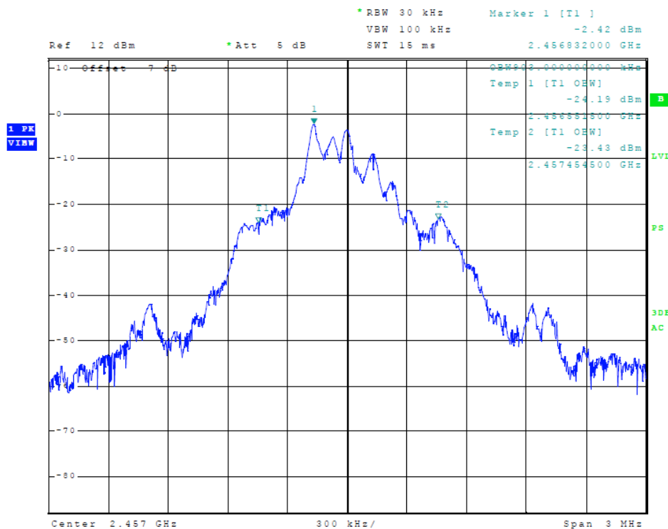
Figure 6 Plot of Transmitter Emissions (99% Occupied Bandwidth, GFSK)
