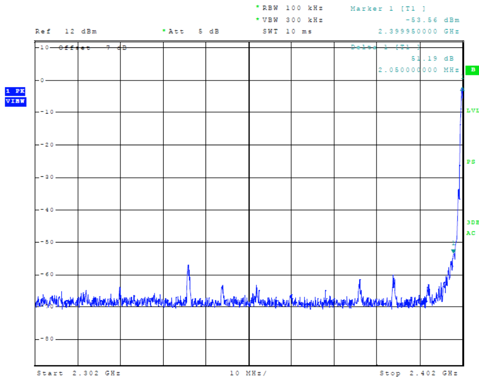
Figure 11 Plot of Transmitter Emissions (Low Band Edge, PRB29)
