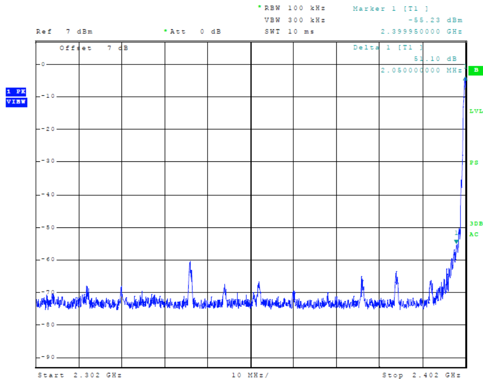
Figure 15 Plot of Transmitter Emissions (Low Band Edge, BLE 0x0F)
