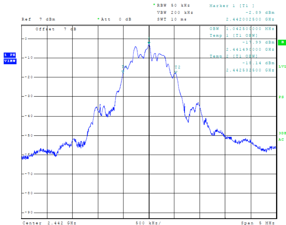
Figure 14 Plot of Transmitter Emissions (99% Occupied Bandwidth, BLE 0x0F)
