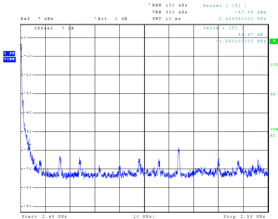
Figure 16 Plot of Transmitter Emissions (High Band Edge, BLE 0x0F)
