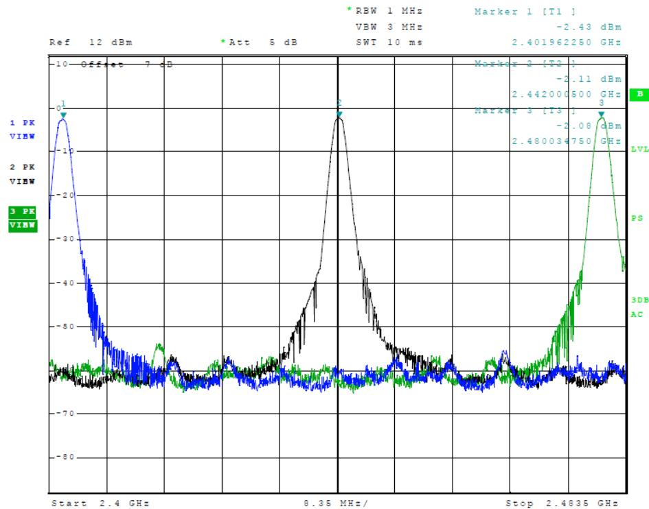
Figure 17 Plot of Transmitter Emissions (Operation in 2402-2480 MHz, BLE 0x55)
