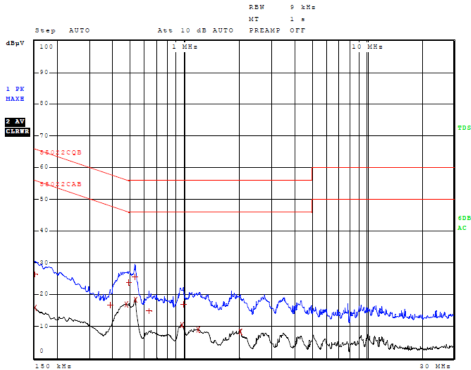
Figure 2 AC Line Conducted emissions of EUT line 2 (#3, EUT – AC Adapter)
