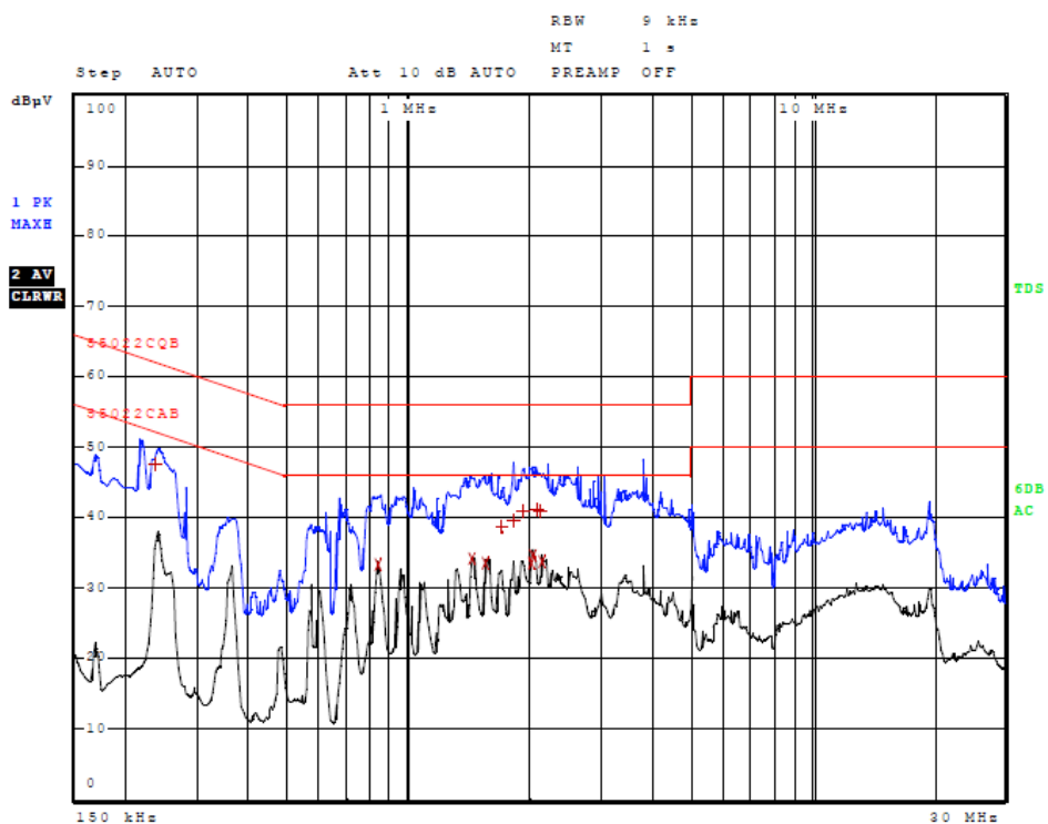
Figure 3 AC Line Conducted emissions of EUT line 1 (#2, EUT - CPU)
