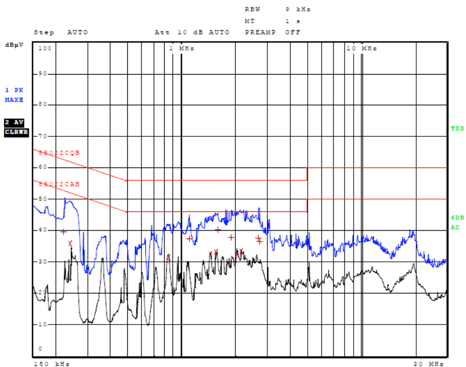
Figure 4 AC Line Conducted emissions of EUT line 2 (#2, EUT - CPU)
