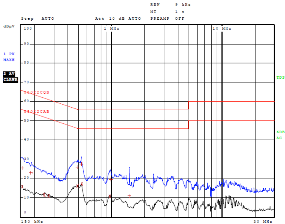
Figure 1 AC Line Conducted emissions of EUT line 1 (#3, EUT – AC Adapter)
