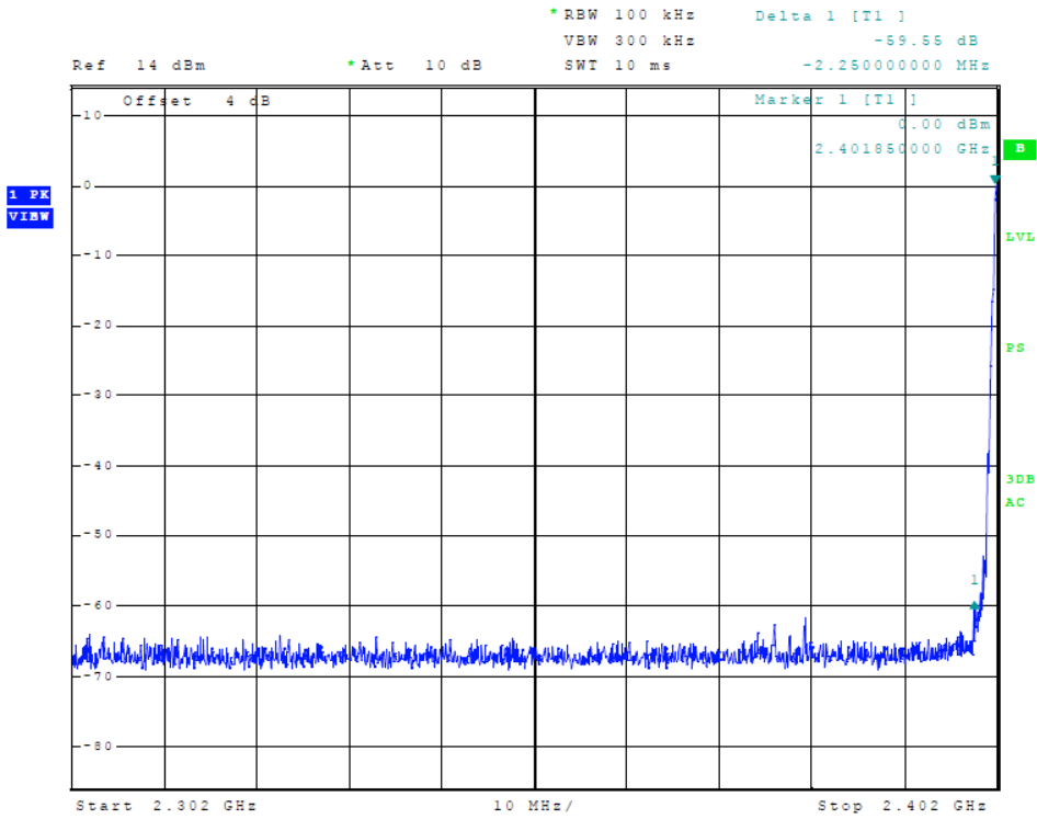
Figure 15 Plot of Transmitter Emissions (Low Band Edge, GFSK)
