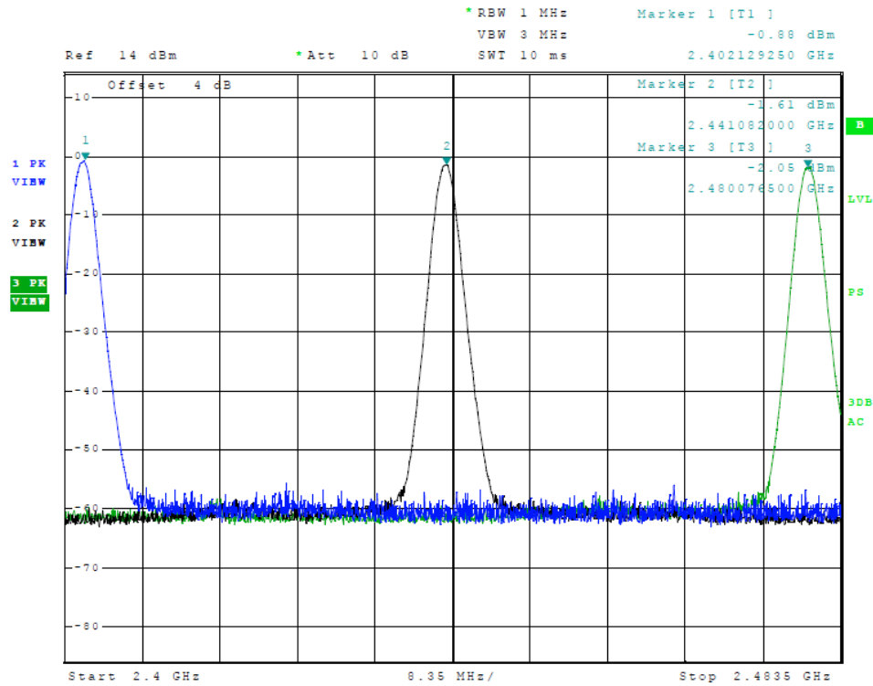
Figure 21 Plot of Transmitter Emissions (Operation in 2402-2480 MHz, 8-DPSK)
