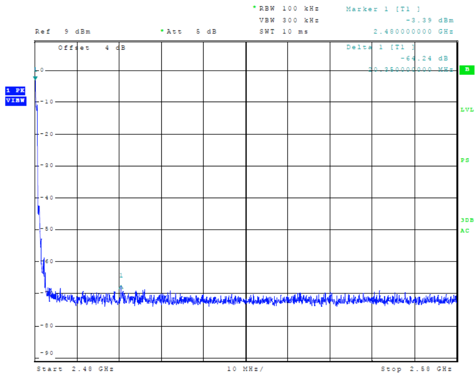
Figure 20 Plot of Transmitter Emissions (High Band Edge, \pi/4 DQPSK)
