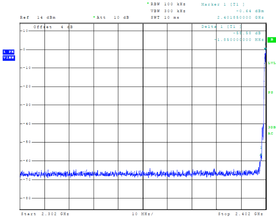
Figure 23 Plot of Transmitter Emissions (Low Band Edge, 8-DPSK)
