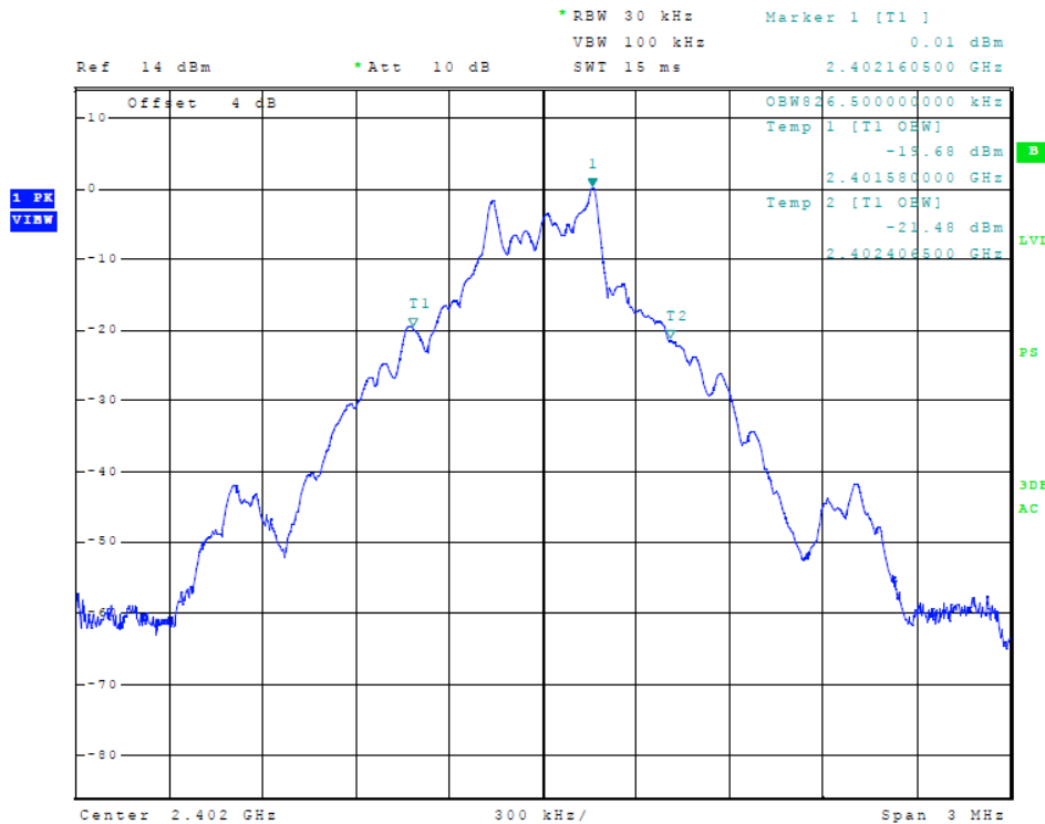
Figure 14 Plot of Transmitter Emissions (99% Occupied Bandwidth, GFSK)
