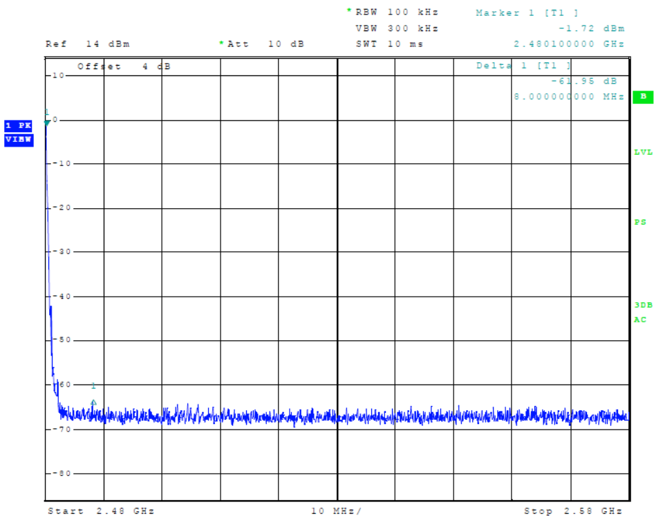
Figure 16 Plot of Transmitter Emissions (High Band Edge, GFSK)
