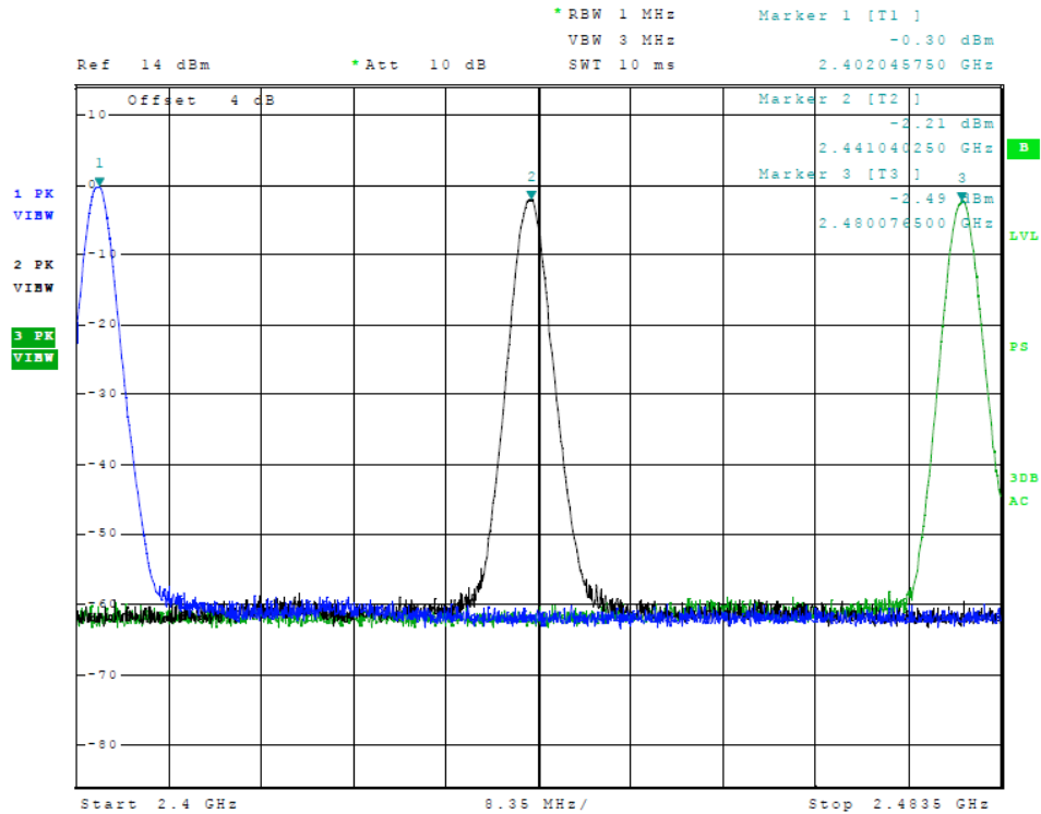
Figure 17 Plot of Transmitter Emissions (Operation in 2402-2480 MHz, \pi/4 DQPSK)
