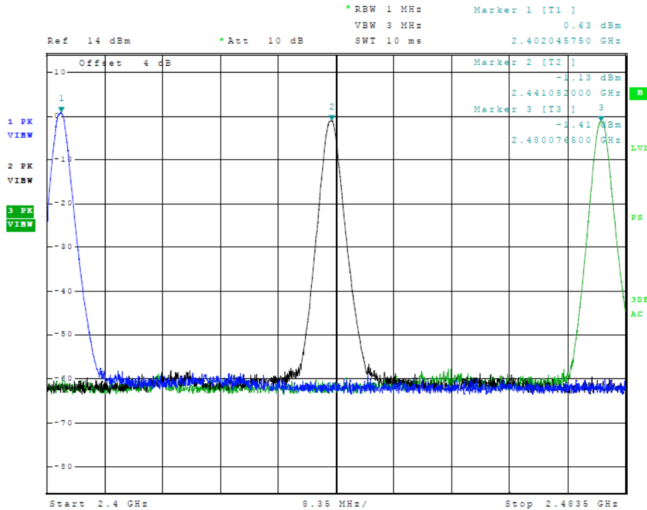
Figure 13 Plot of Transmitter Emissions (Operation in 2402-2480 MHz. GFSK)
