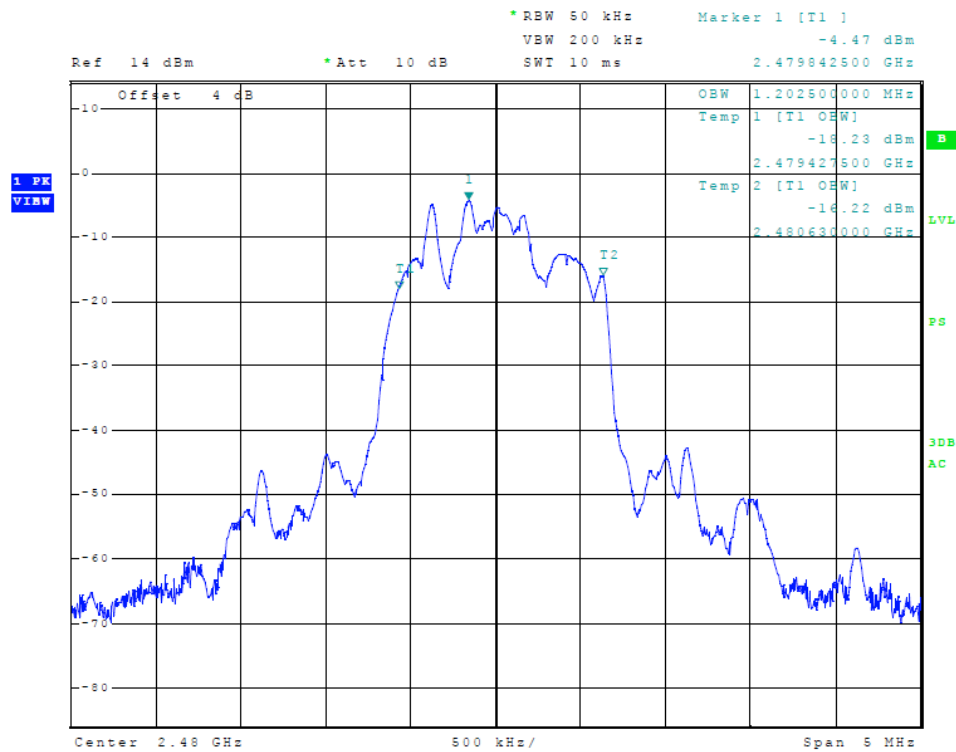
Figure 22 Plot of Transmitter Emissions (99% Occupied Bandwidth, 8-DPSK)
