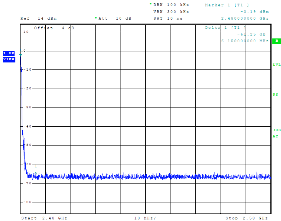
Figure 24 Plot of Transmitter Emissions (High Band Edge, 8-DPSK)
