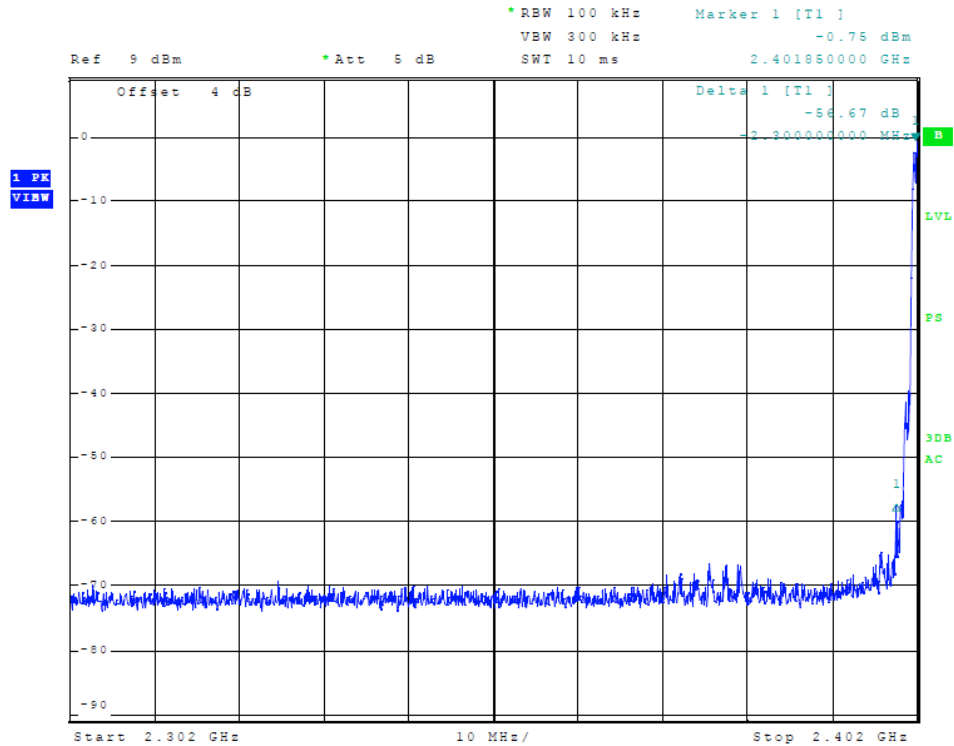
Figure 19 Plot of Transmitter Emissions (Low Band Edge, \pi/4 DQPSK)
