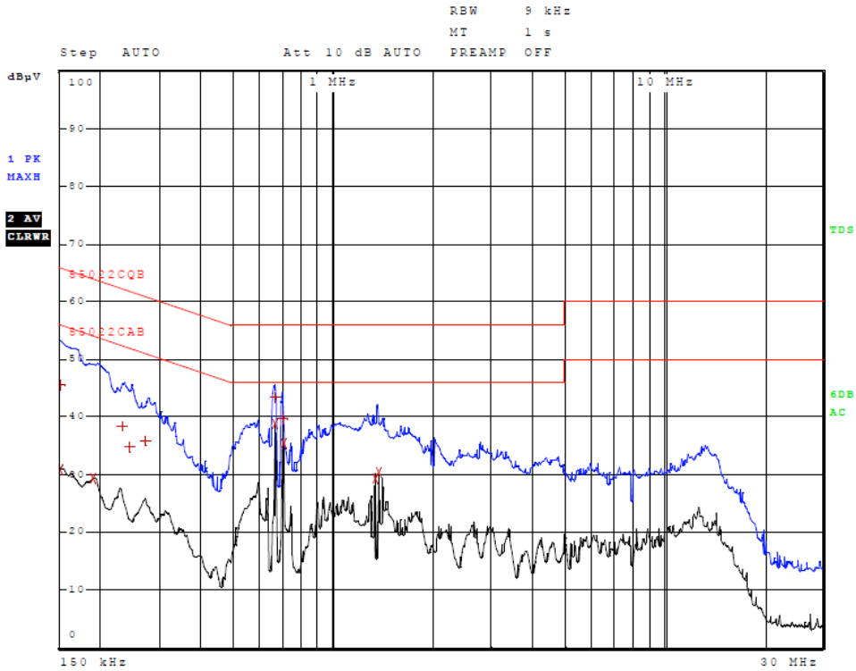
Figure 1 AC Line Conducted emissions of EUT line 1 (#2, EUT, Mount, 96 Adapter)
