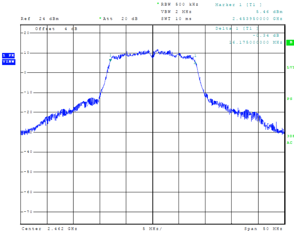
Figure 26 Plot of Transmitter 6-dB Occupied Bandwidth (802.11 g-mode)
