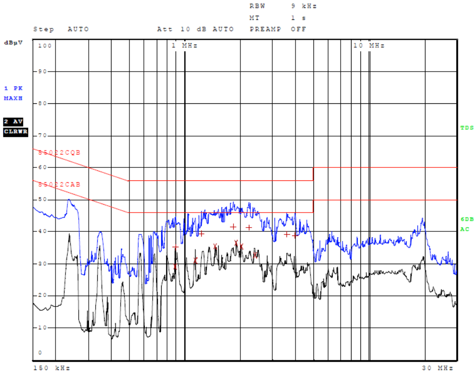
Figure 9 AC Line Conducted emissions of EUT line 1 (#6, EUT, USB CPU Adapter)
