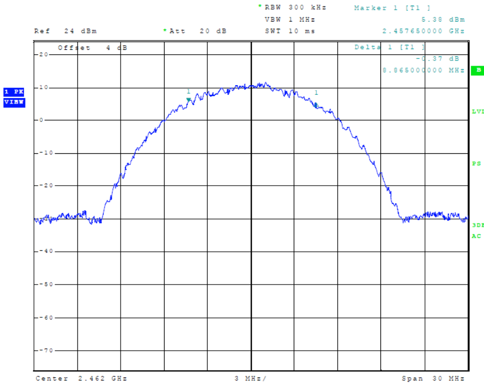
Figure 25 Plot of Transmitter 6-dB Occupied Bandwidth (802.11 b-mode)
