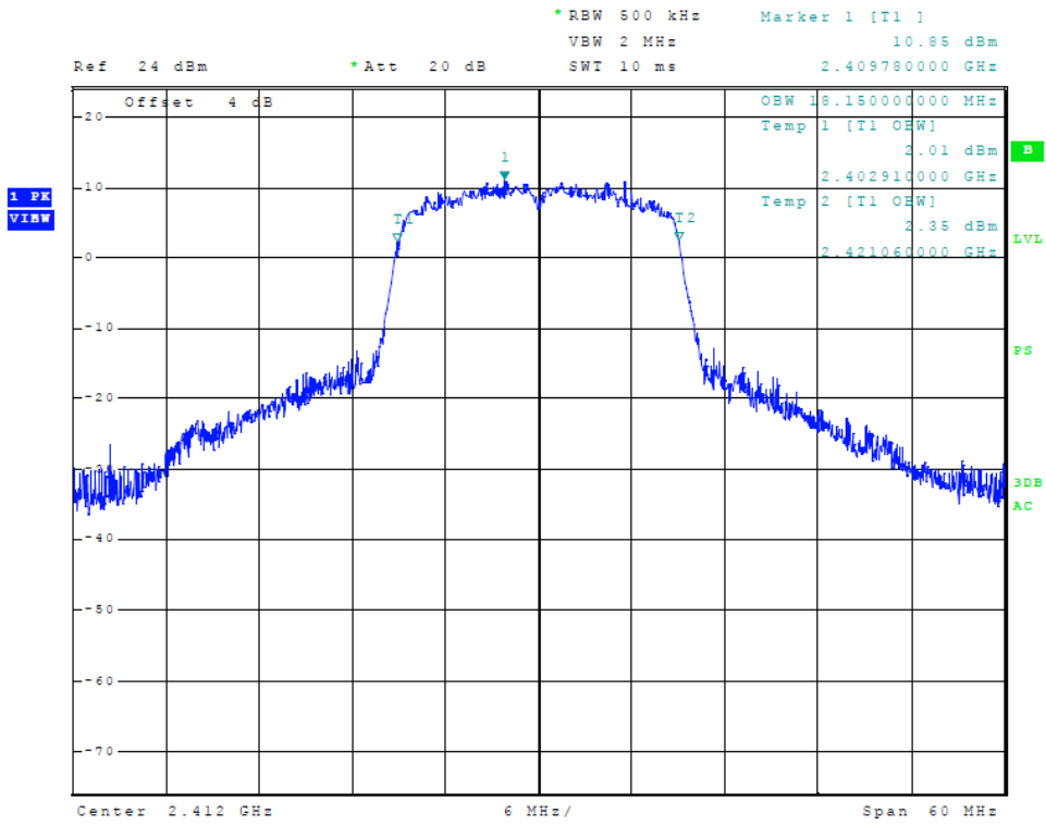
Figure 31 Plot of Transmitter 99% Occupied Bandwidth (802.11 n-mode)
