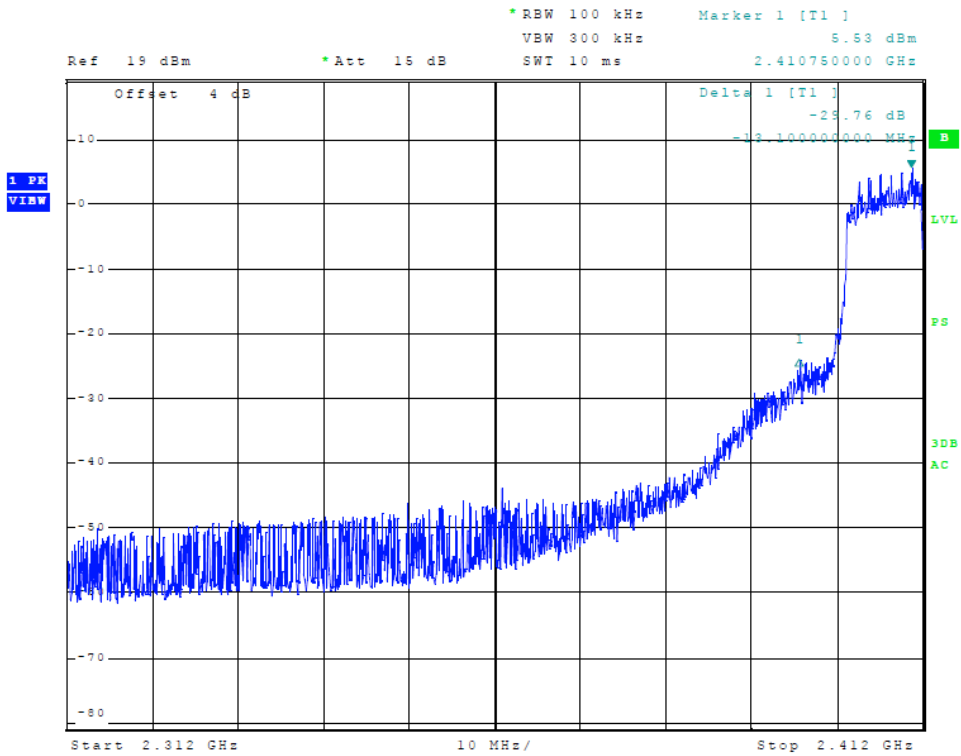
Figure 19 Plot of Lower Band Edge (802.11 n-mode)
