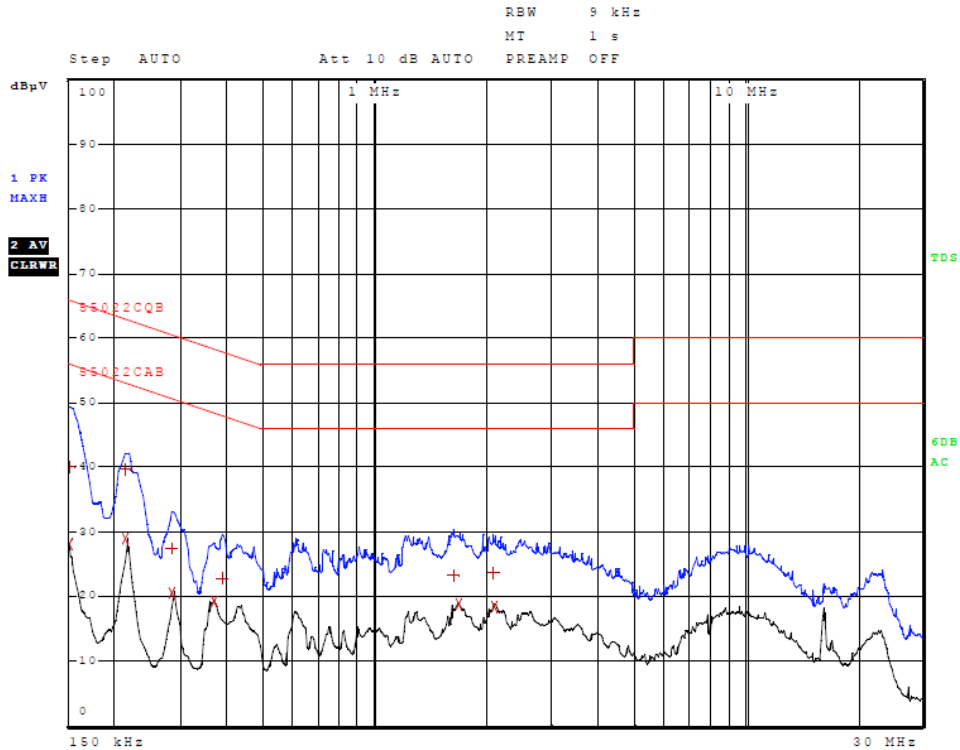
Figure 8 AC Line Conducted emissions of EUT line 2 (#5, EUT, 86 Adapter)
