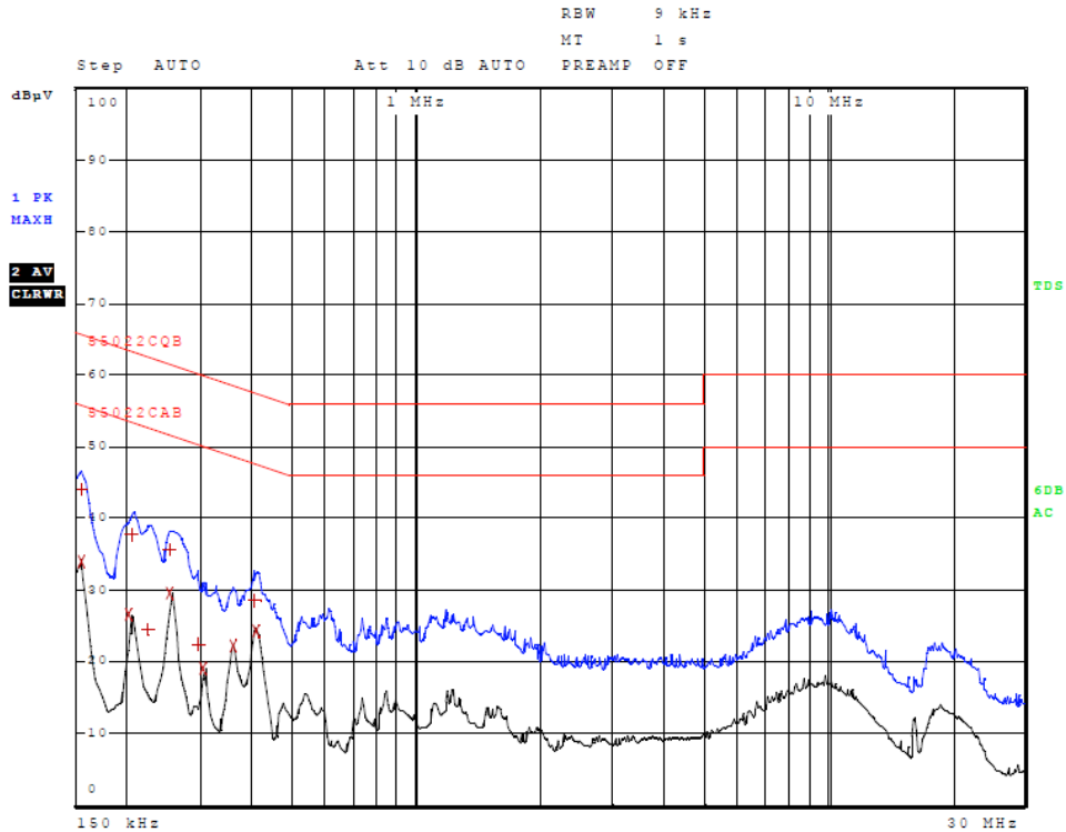
Figure 3 AC Line Conducted emissions of EUT line 1 (#2, EUT, Mount, 86 Adapter)
