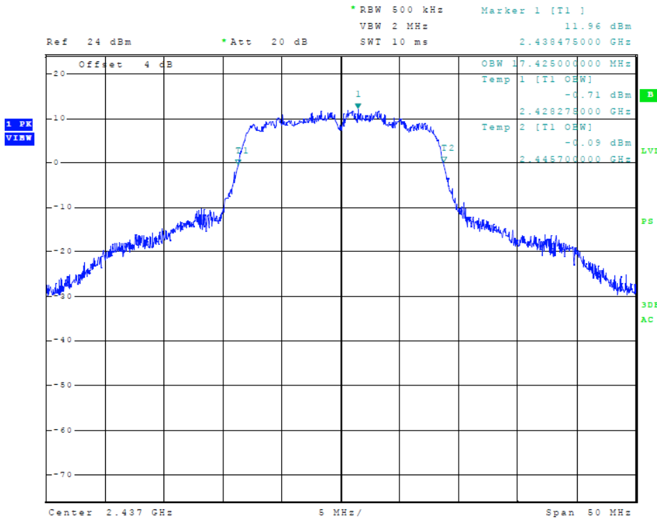
Figure 30 Plot of Transmitter 99% Occupied Bandwidth (802.11 g-mode)
