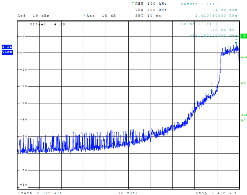
Figure 18 Plot of Lower Band Edge (802.11 g-mode)
