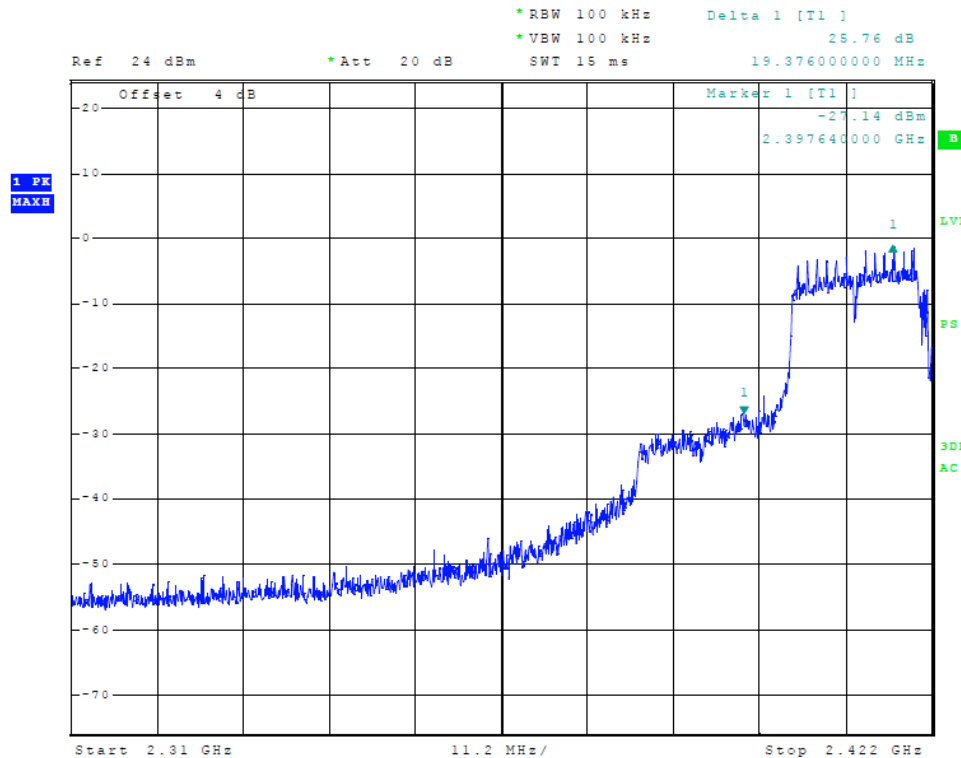
Figure 20 Plot of Lower Band Edge (802.11 n40-mode)
