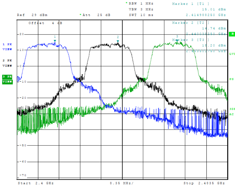
Figure 14 Plot of Transmitter Emissions in Operational Frequency (802.11 g-Mode)
