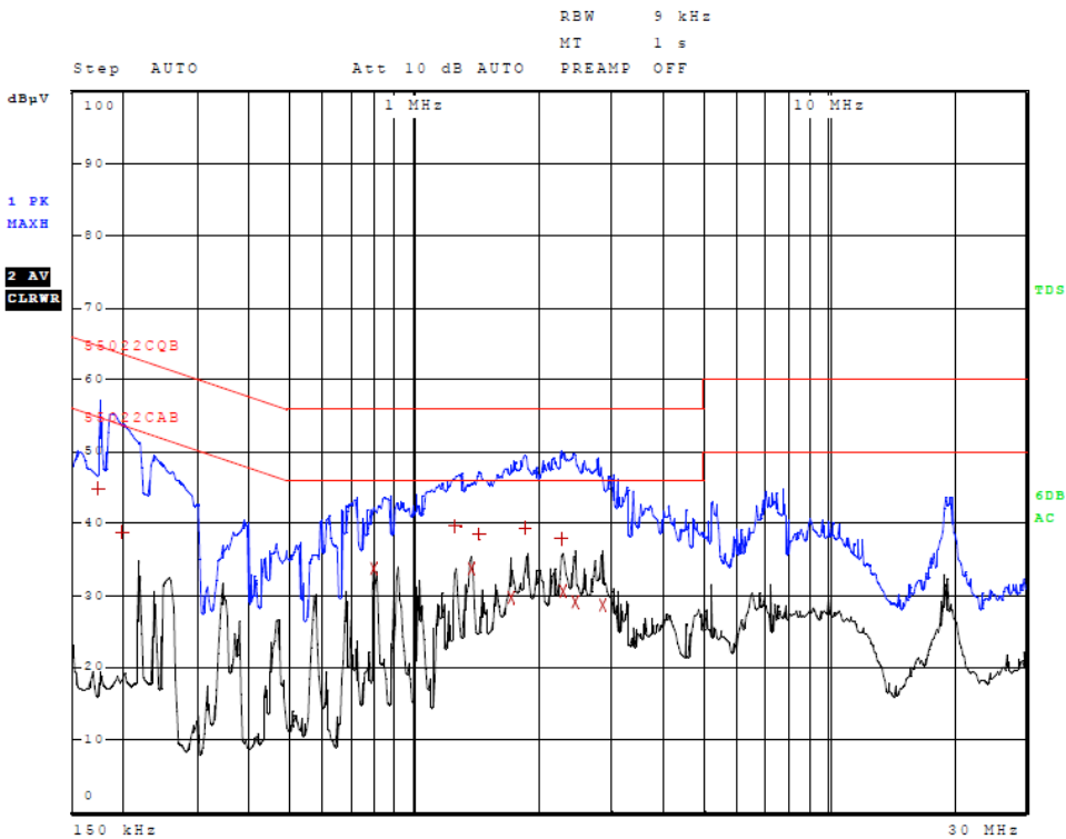
Figure 12 AC Line Conducted emissions of EUT line 2 (#6, EUT, Mount, USB CPU)
