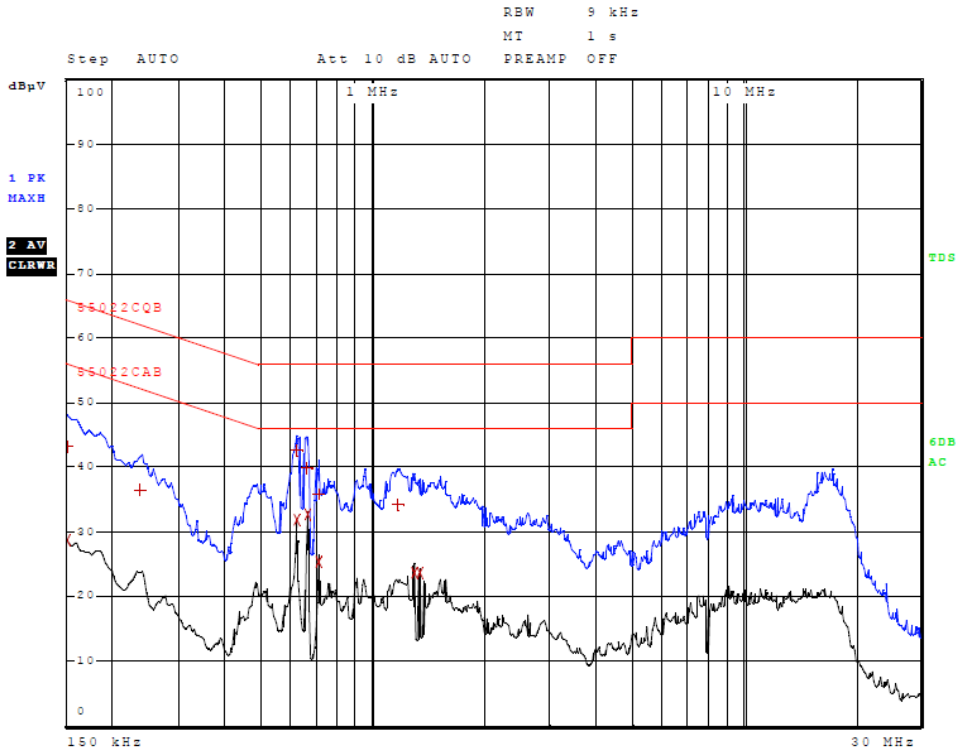
Figure 6 AC Line Conducted emissions of EUT line 2 (#5, EUT, 96 Adapter)
