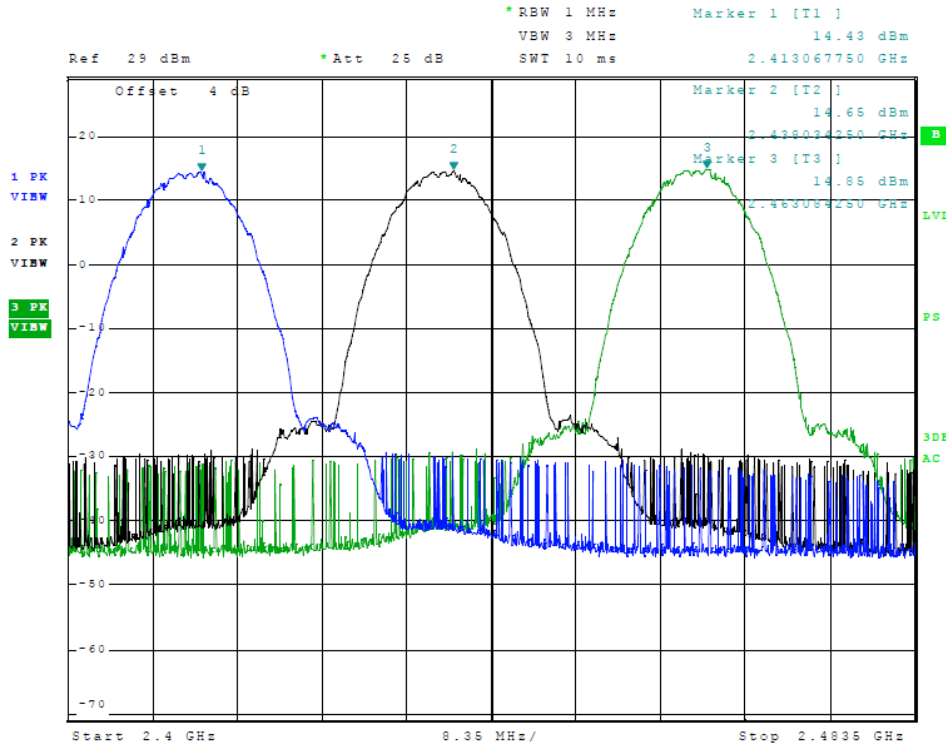
Figure 13 Plot of Transmitter Emissions in Operational Frequency (802.11 b-Mode)
