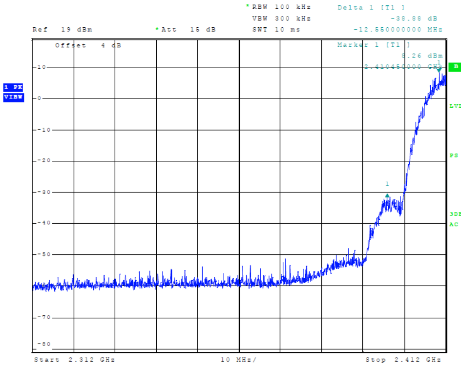
Figure 17 Plot of Lower Band Edge (802.11 b-mode)
