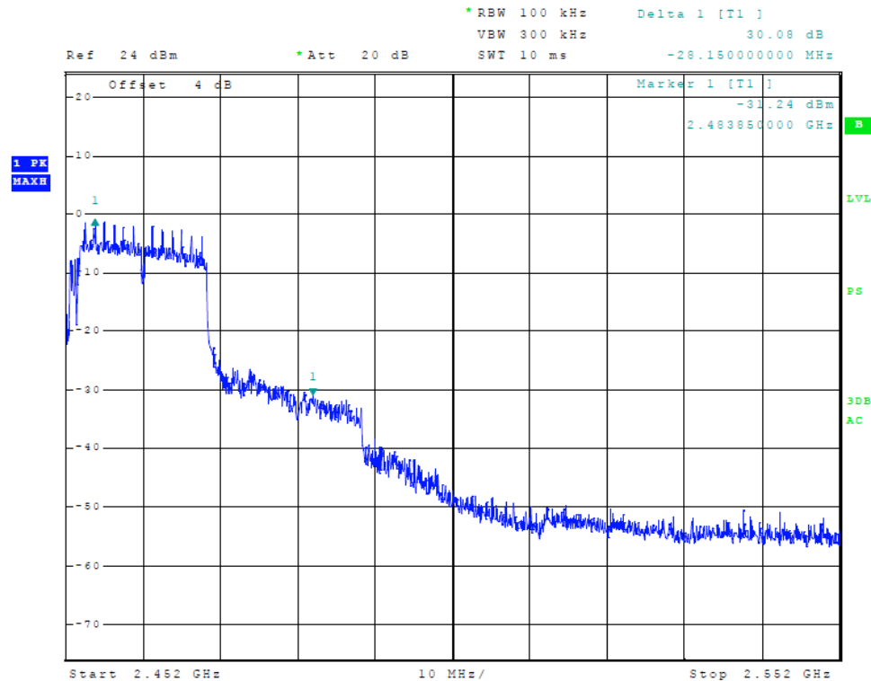
Figure 24 Plot of Upper Band Edge (802.11 n40-mode)
