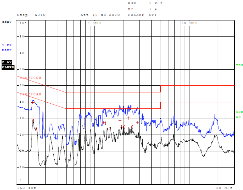
Figure 10 AC Line Conducted emissions of EUT line 2 (#6, EUT, USB CPU Adapter)
