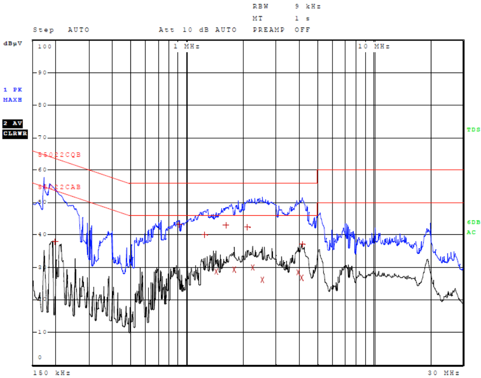
Figure 11 AC Line Conducted emissions of EUT line 1 (#6, EUT, Mount, USB CPU)
