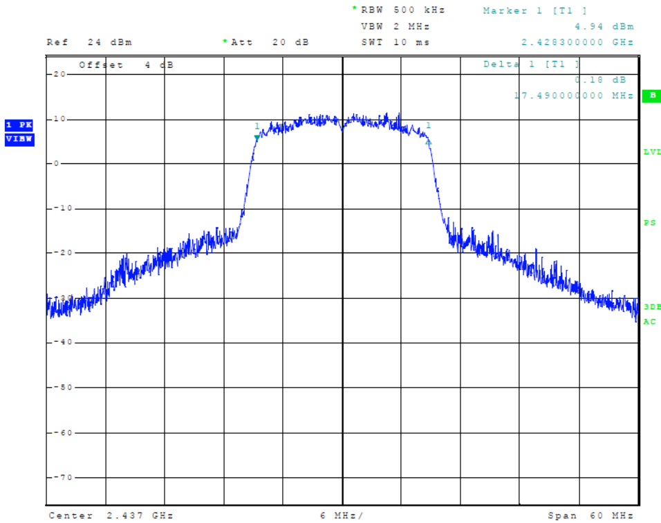
Figure 27 Plot of Transmitter 6-dB Occupied Bandwidth (802.11 n-mode)
