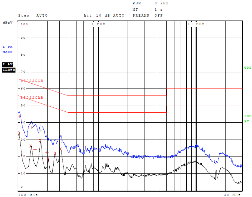
Figure 4 AC Line Conducted emissions of EUT line 2 (#2, EUT, Mount, 86 Adapter)
