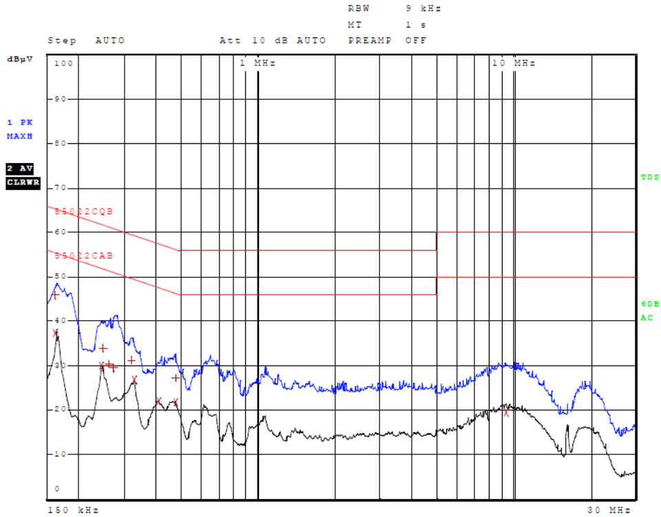
Figure 7 AC Line Conducted emissions of EUT line 1 (#5, EUT, 86 Adapter)
