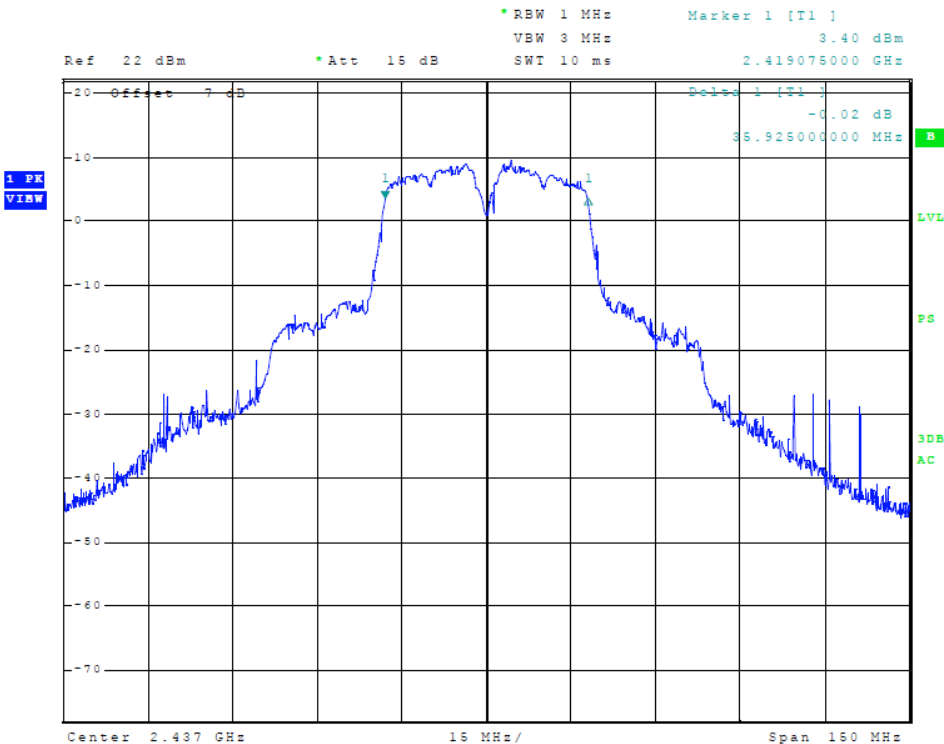
Figure 28 Plot of Transmitter 6-dB Occupied Bandwidth (802.11 n40-mode)
