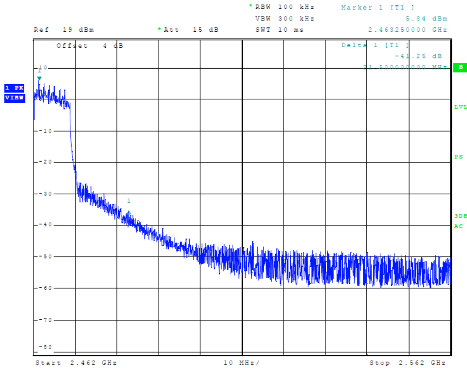
Figure 23 Plot of Upper Band Edge (802.11 n-mode)
