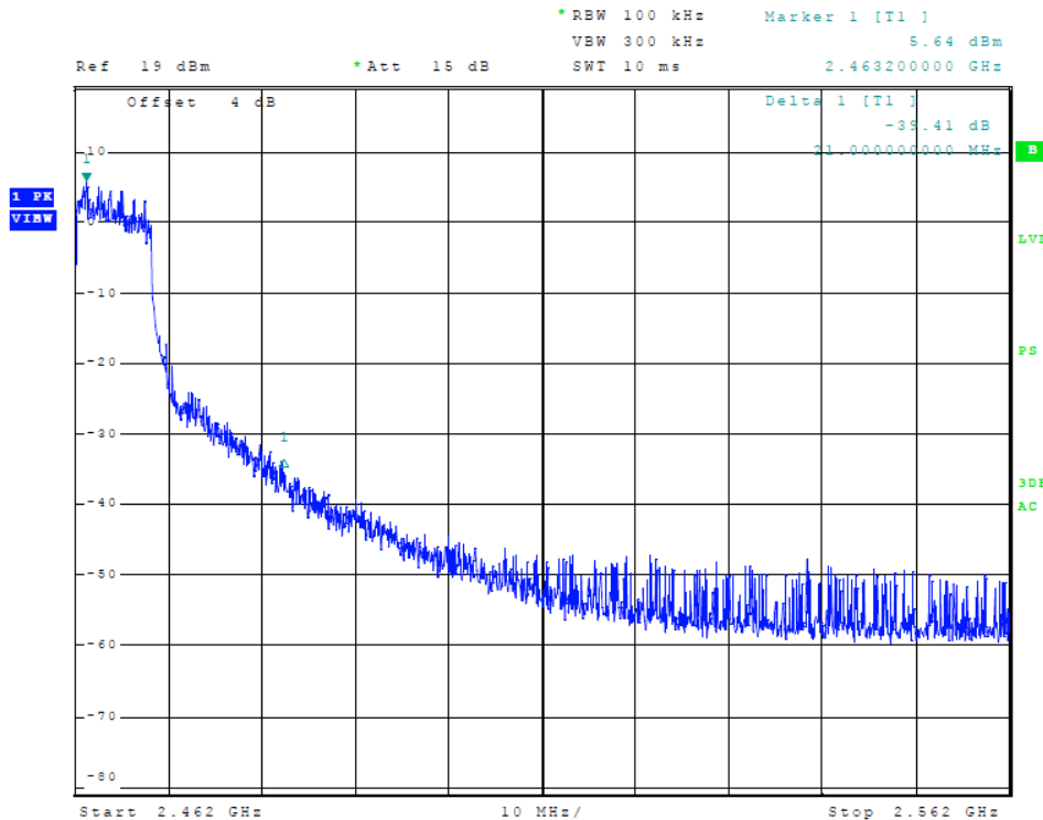
Figure 22 Plot of Upper Band Edge (802.11 g-mode)
