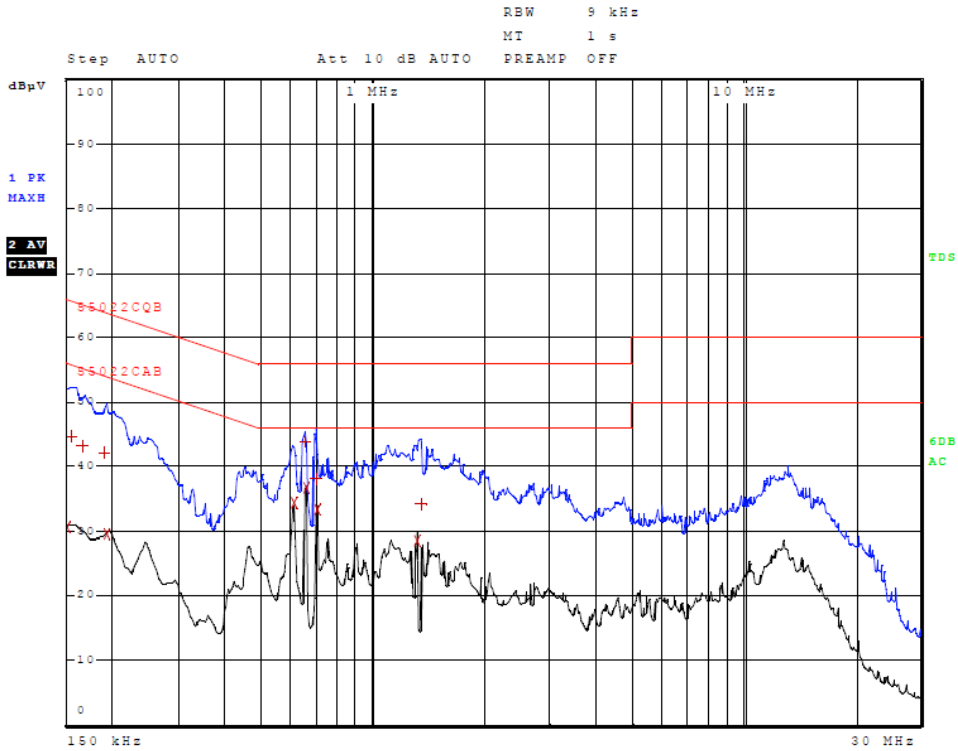
Figure 5 AC Line Conducted emissions of EUT line 1 (#5, EUT, 96 Adapter)
