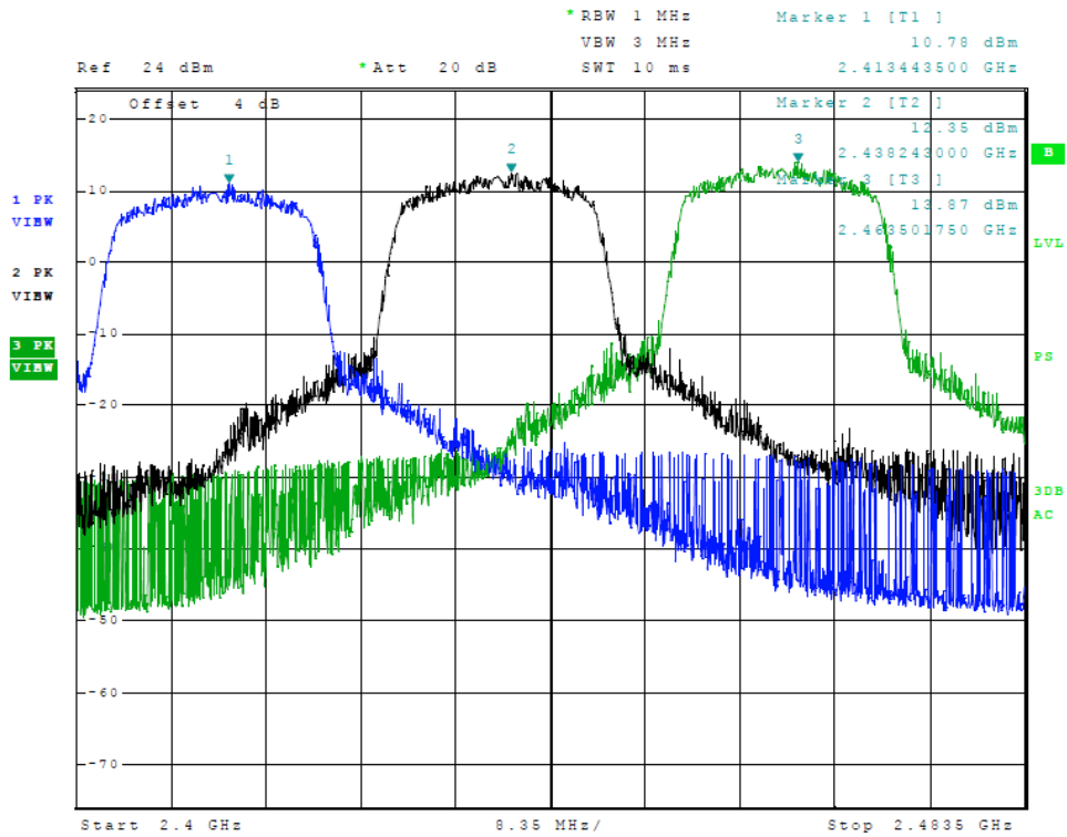
Figure 15 Plot of Transmitter Emissions in Operational Frequency (802.11 n-Mode)
