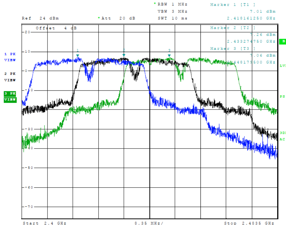
Figure 16 Plot of Transmitter Emissions in Operational Frequency (802.11 n40-Mode)
