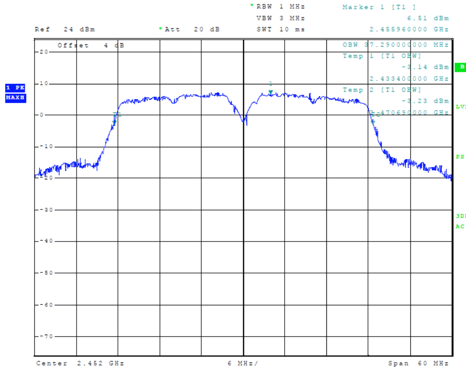
Figure 32 Plot of Transmitter 99% Occupied Bandwidth (802.11 n40-mode)
