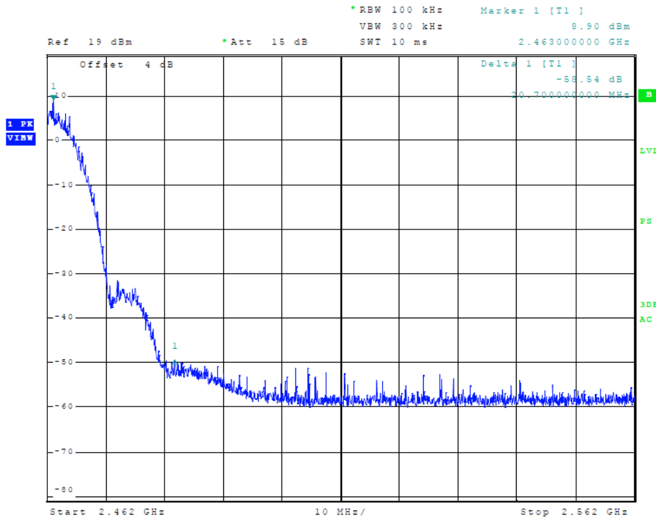
Figure 21 Plot of Upper Band Edge (802.11 b-mode)
