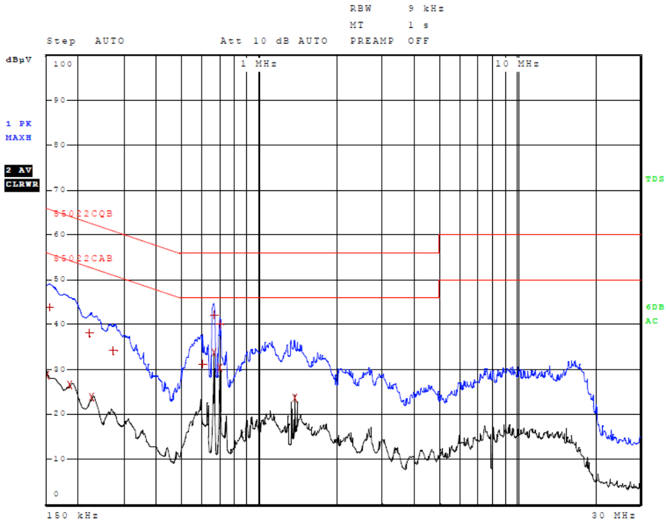
Figure 2 AC Line Conducted emissions of EUT line 2 (#2, EUT, Mount, 96 Adapter)
