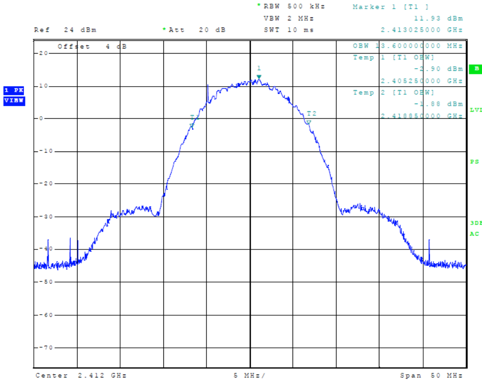
Figure 29 Plot of Transmitter 99% Occupied Bandwidth (802.11 b-mode)
