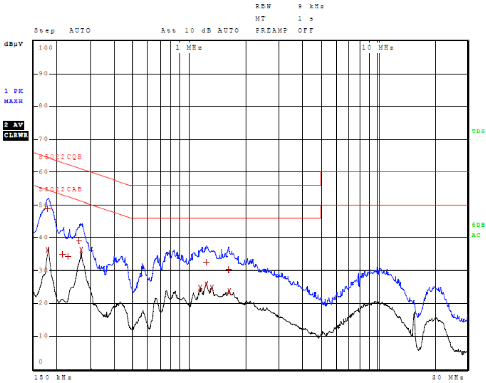
Figure 3 AC Line Conducted emissions of EUT line 1 (#5, EUT AC Adapter 362-00086-01)
