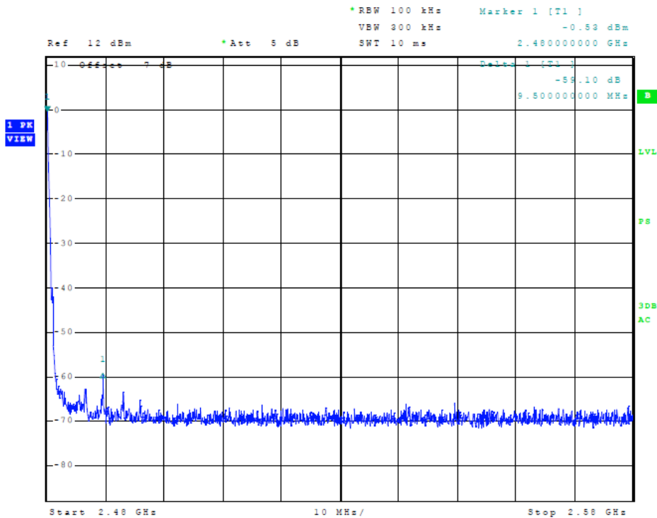
Figure 10 Plot of Transmitter Emissions (Mode 1, High Band Edge)
