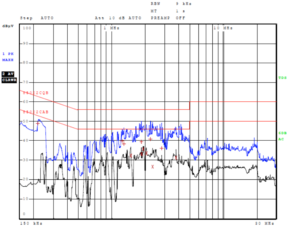
Figure 1 AC Line Conducted emissions of EUT line 1 (#4, EUT USB CPU Adapter)
