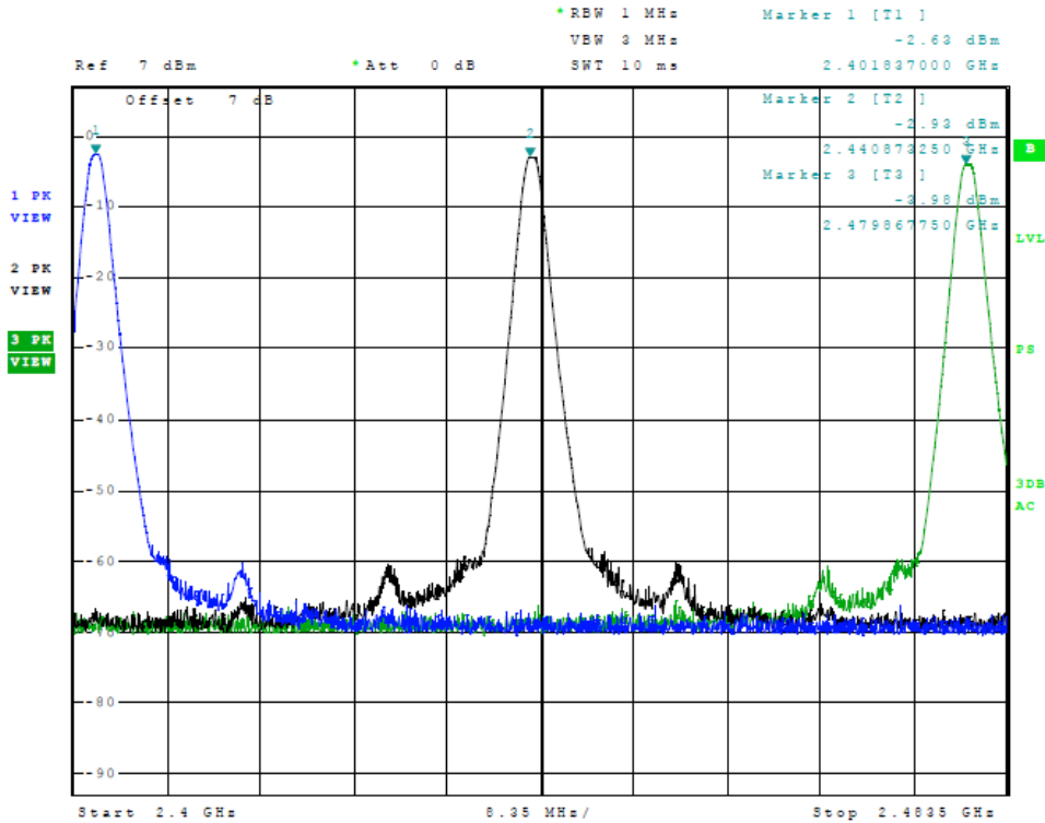
Figure 11 Plot of Transmitter Emissions (Mode 2 Operation in 2402-2480 MHz)
