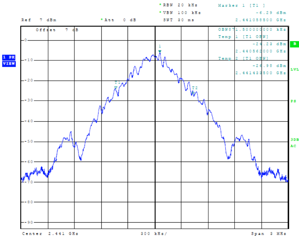
Figure 12 Plot of Transmitter Emissions (Mode 2, 99% Occupied Bandwidth)
