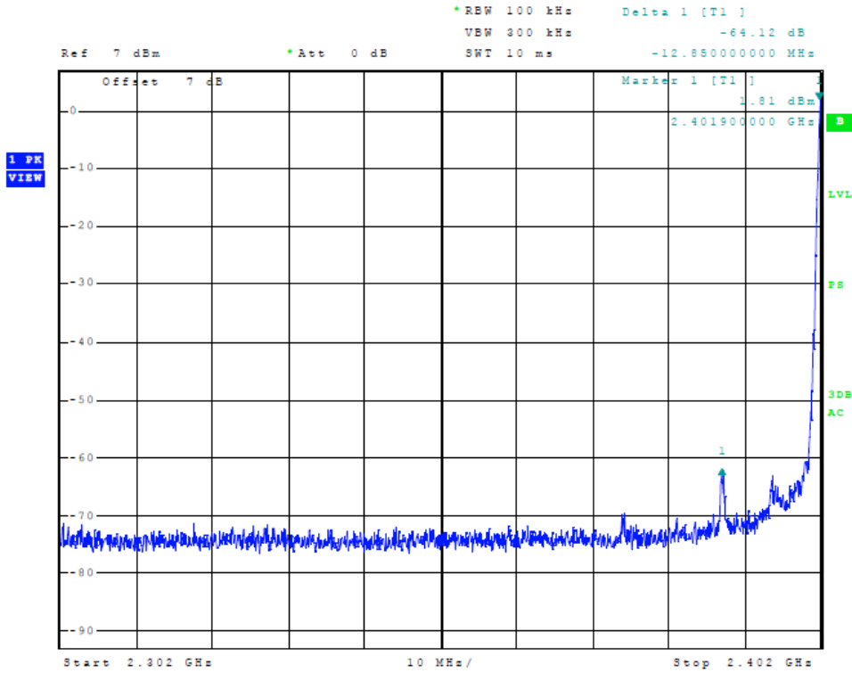
Figure 13 Plot of Transmitter Emissions (Mode 2, Low Band Edge)
