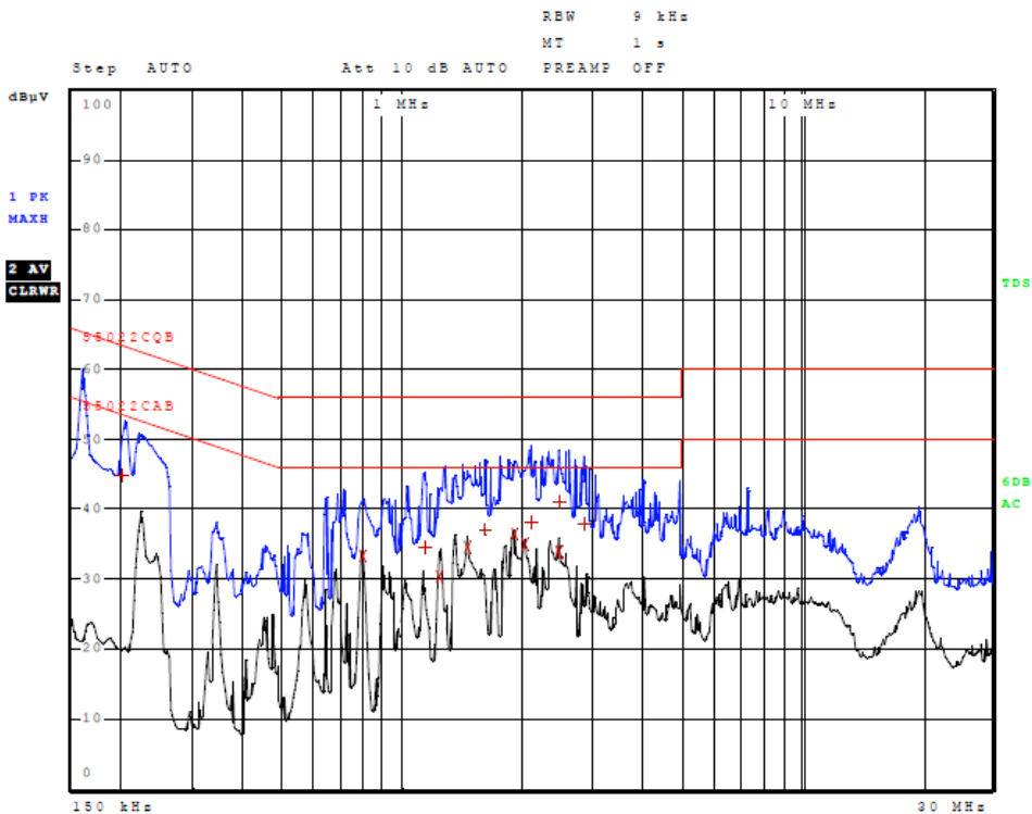
Figure 2 AC Line Conducted emissions of EUT line 2 (#4, EUT USB CPU Adapter)
