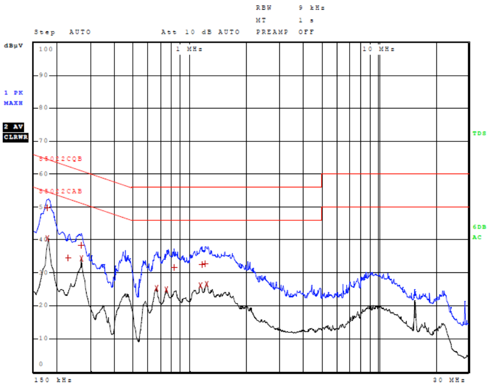
Figure 4 AC Line Conducted emissions of EUT line 2 (#5, EUT AC Adapter 362-00086-01)
