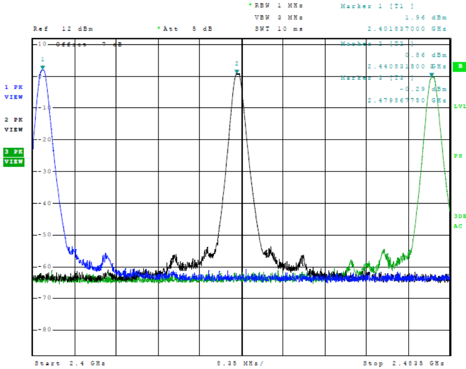
Figure 7 Plot of Transmitter Emissions (Mode 1, Operation in 2402-2480 MHz)
