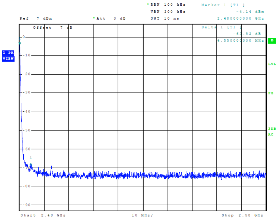
Figure 14 Plot of Transmitter Emissions (Mode 2, High Band Edge)
