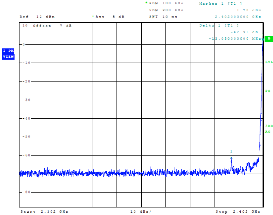
Figure 9 Plot of Transmitter Emissions (Mode 1, Low Band Edge)
