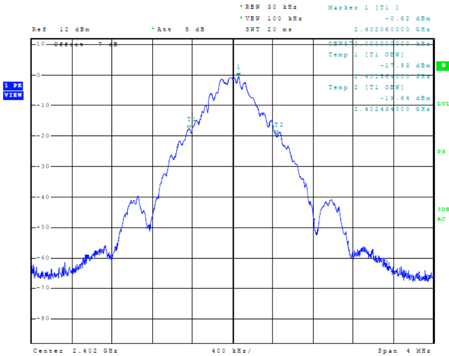
Figure 8 Plot of Transmitter Emissions (Mode 1, 99% Occupied Bandwidth)
