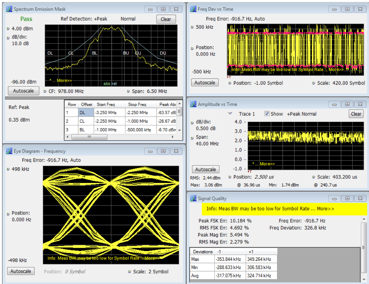
Figure 2 Modulation Characteristics
