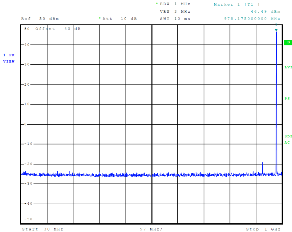
Figure 1 Power Output Across Frequency Band 978 MHz
