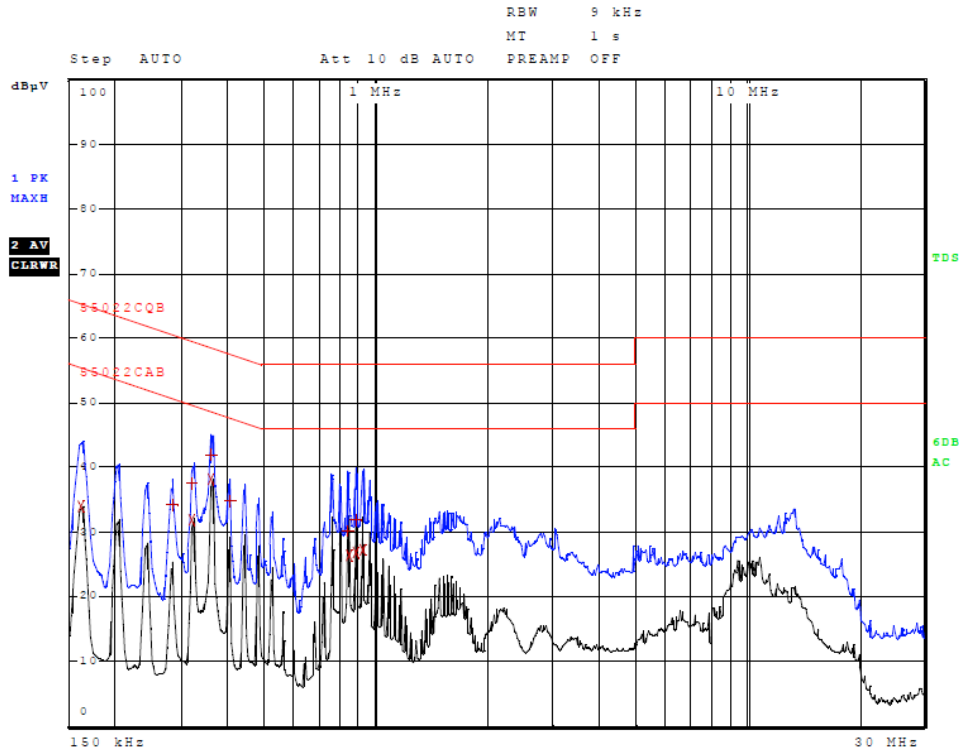
Figure 5 AC Line Conducted emissions of EUT line 1 (EUT AC Adapter 326-00072-00)
