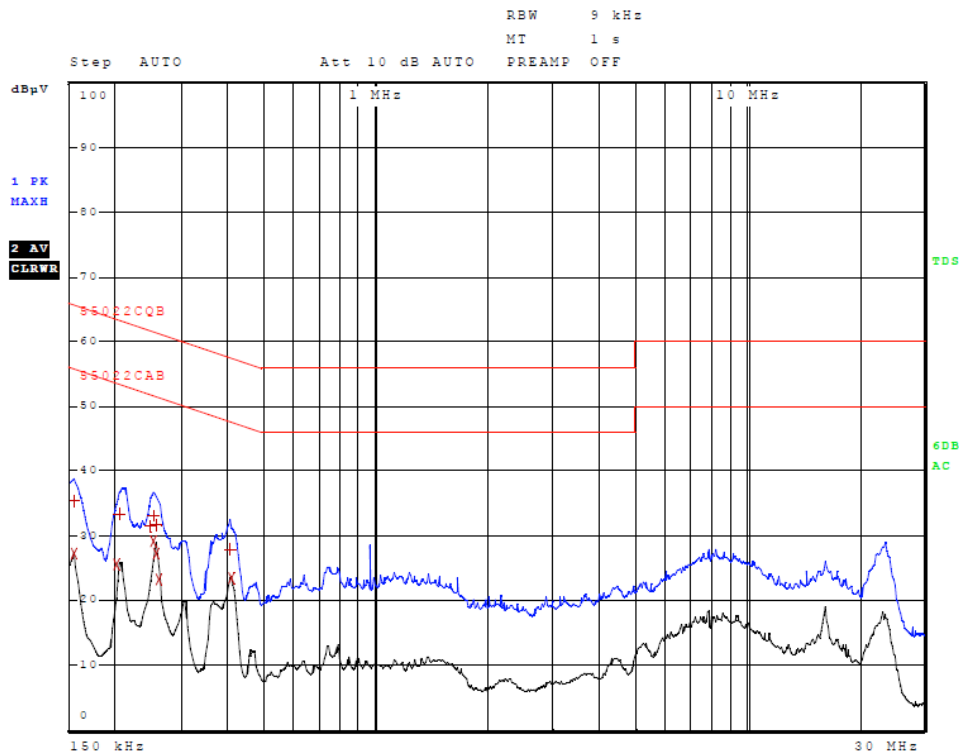
Figure 8 AC Line Conducted emissions of EUT line 2 (EUT AC Adapter 326-00086-01)
