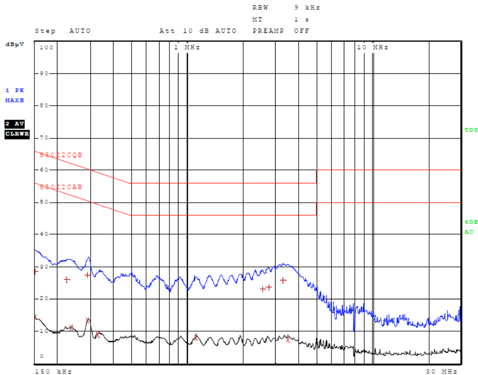
Figure 4 AC Line Conducted emissions of EUT line 2 (EUT AC Adapter SCB055600P)
