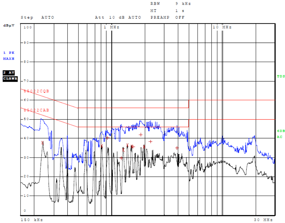
Figure 1 AC Line Conducted emissions of EUT line 1 (EUT-USB-CPU AC Adapter)
