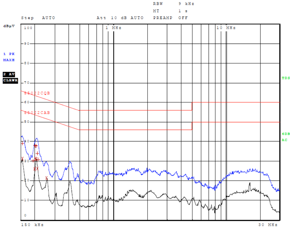
Figure 7 AC Line Conducted emissions of EUT line 1 (EUT AC Adapter 326-00086-01)
