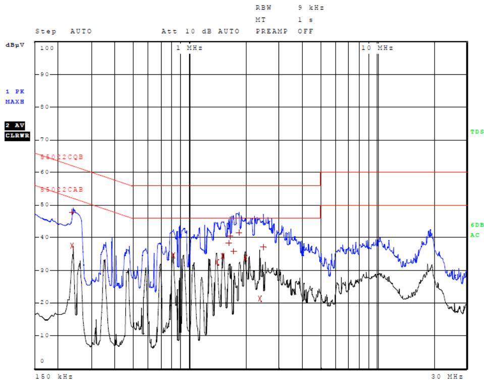
Figure 2 AC Line Conducted emissions of EUT line 2 (EUT-USB-CPU AC Adapter)
