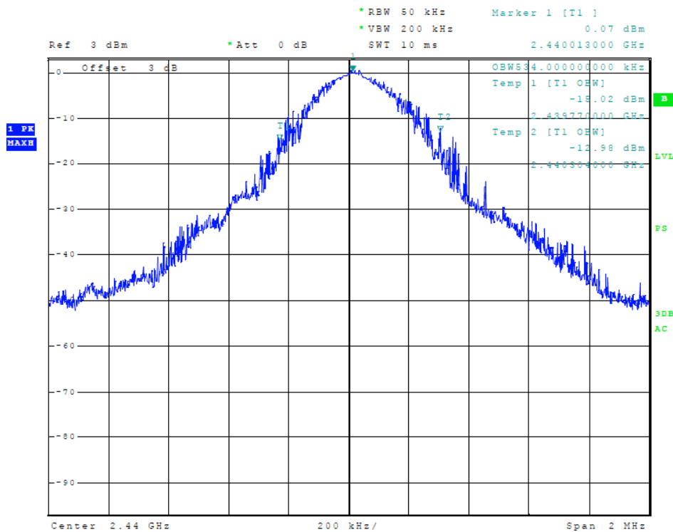
Figure 16 Plot of Transmitter Emissions (99% Occupied Bandwidth, Mode 2)
