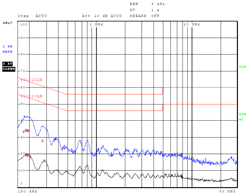
Figure 10 AC Line Conducted emissions of EUT line 2 (EUT AC Adapter 326-00087-00)
