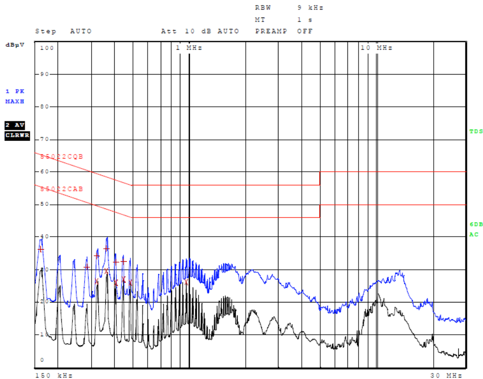
Figure 6 AC Line Conducted emissions of EUT line 2 (EUT AC Adapter 326-00072-00)
