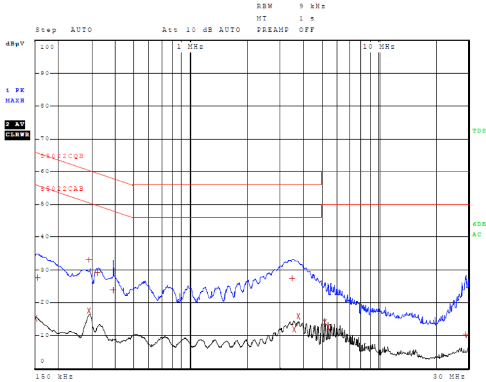
Figure 3 AC Line Conducted emissions of EUT line 1 (EUT AC Adapter SCB055600P)
