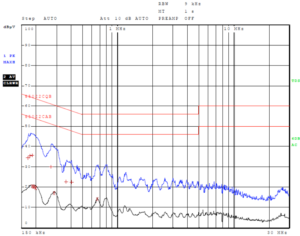
Figure 9 AC Line Conducted emissions of EUT line 1 (EUT AC Adapter 326-00087-00)
