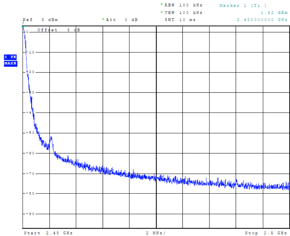
Figure 18 Plot of Transmitter Emissions (High Band Edge, Mode 21)
