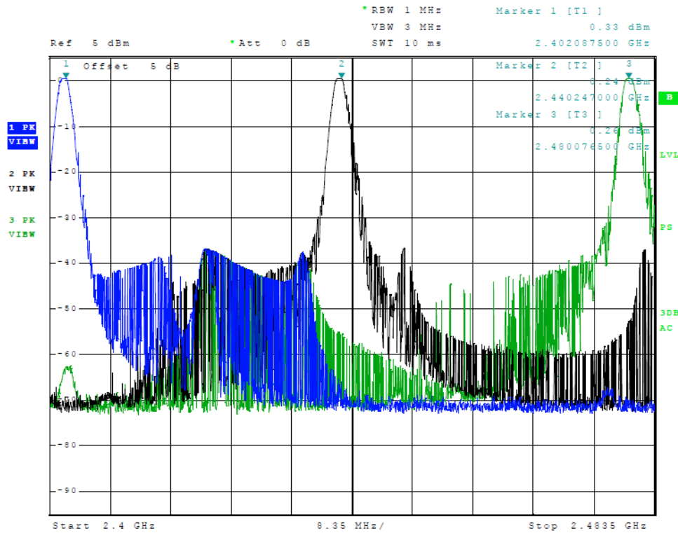
Figure 1 Plot of Transmitter Emissions (In 2402-2480 MHz)
