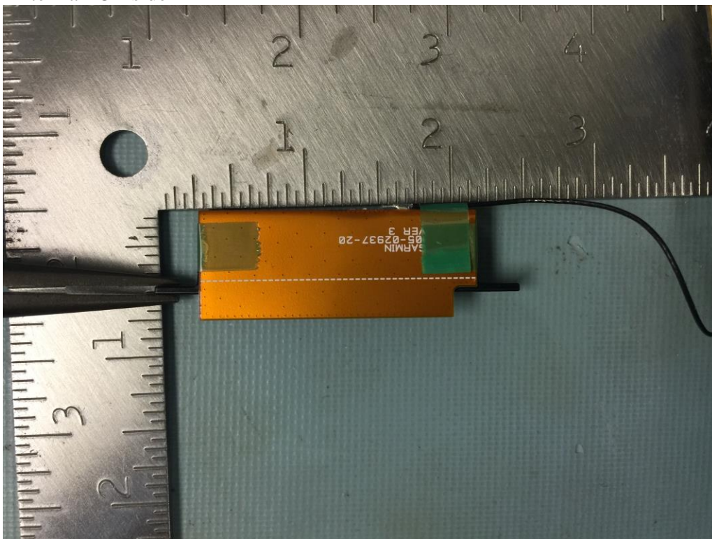
Antenna PCB side
