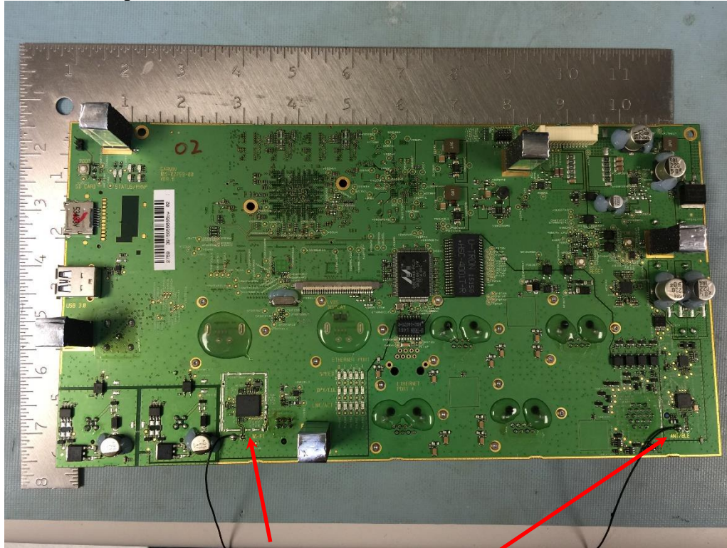
Transmitter sections
