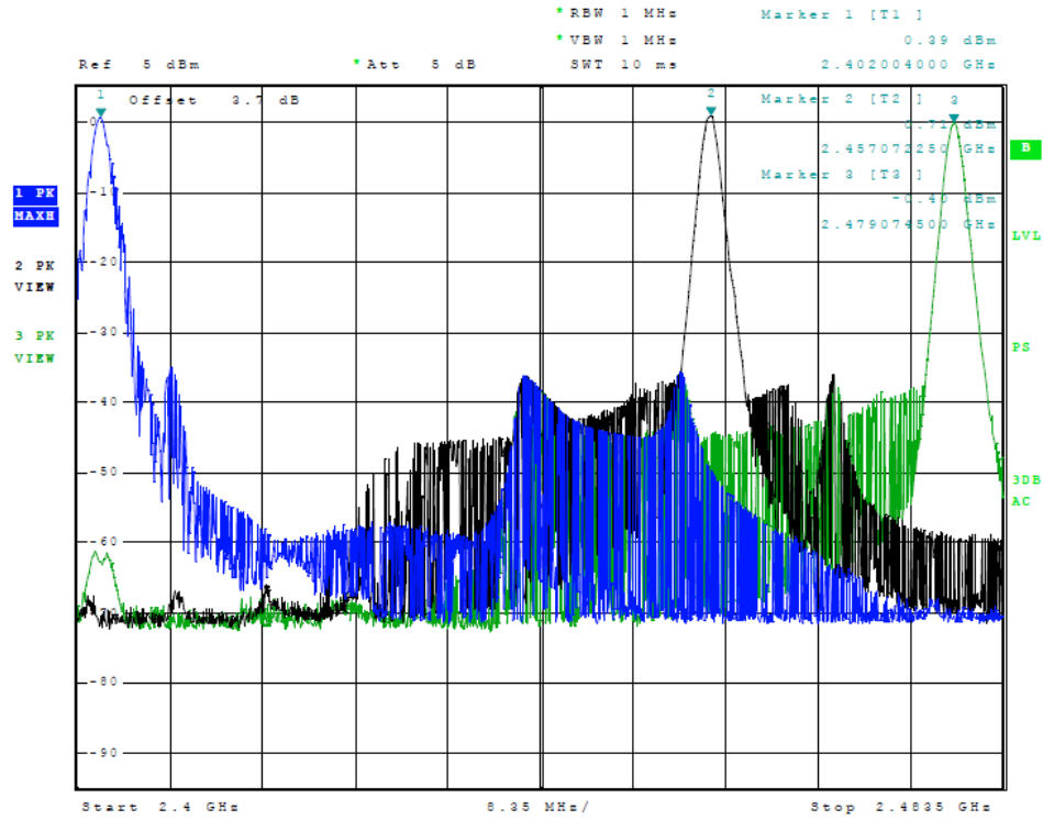
Figure 11 Plot of Transmitter Emissions (In 2402-2480 MHz Band) (Mode 1)
