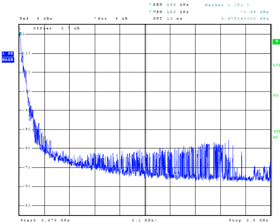
Figure 14 Plot of Low Band Edge (High Band Edge) (Mode 1)
