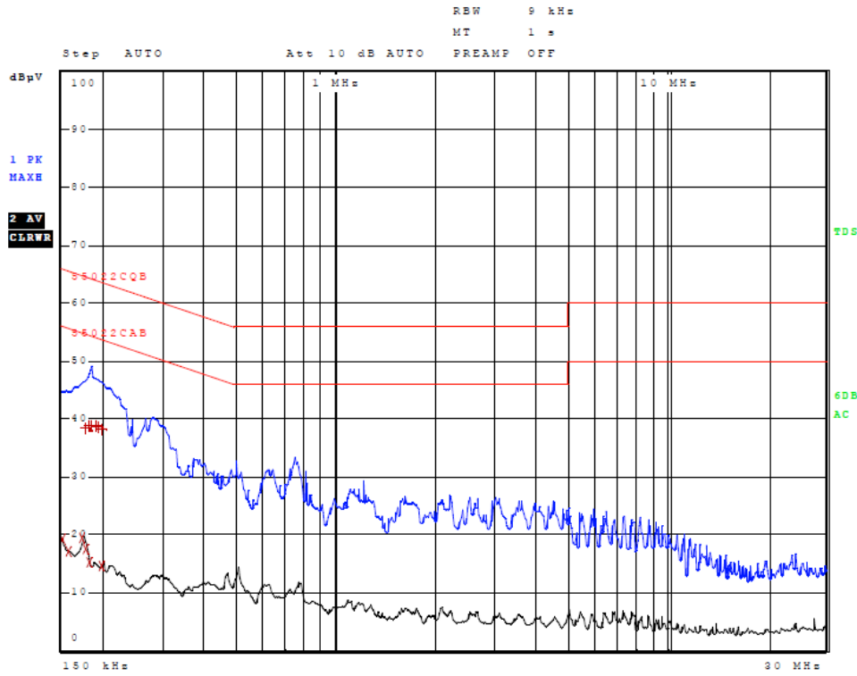
Figure 7 AC Line Conducted emissions of EUT line 2 (EUT AC Adapter, 362-00087-00)
