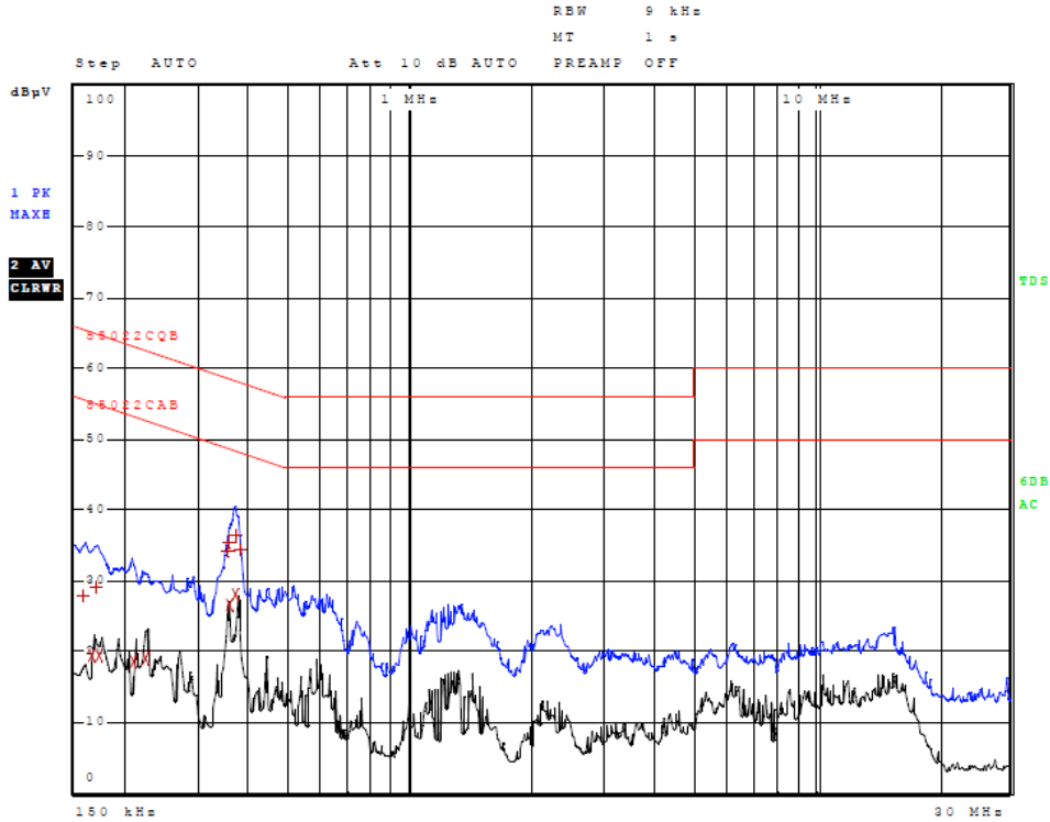
Figure 3 AC Line Conducted emissions of EUT line 2 (EUT AC Adapter, 362-00072-00)
