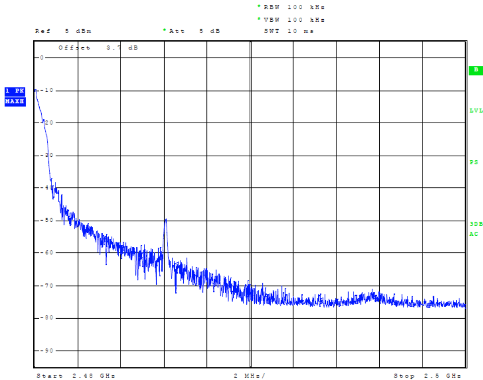
Figure 18 Plot of Low Band Edge (High Band Edge) (Mode 2)
