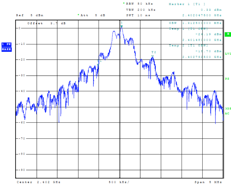
Figure 12 Plot of Transmitter Emissions (99% Occupied Bandwidth) (Mode 1)
