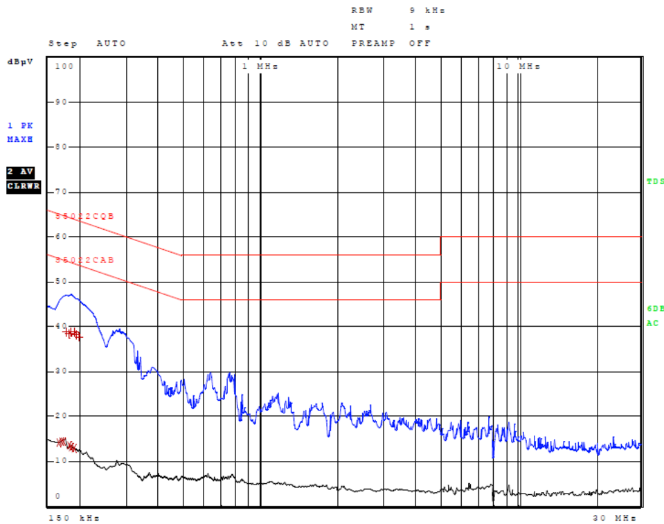
Figure 8 AC Line Conducted emissions of EUT line 2 (EUT AC Adapter, 362-00087-00)
