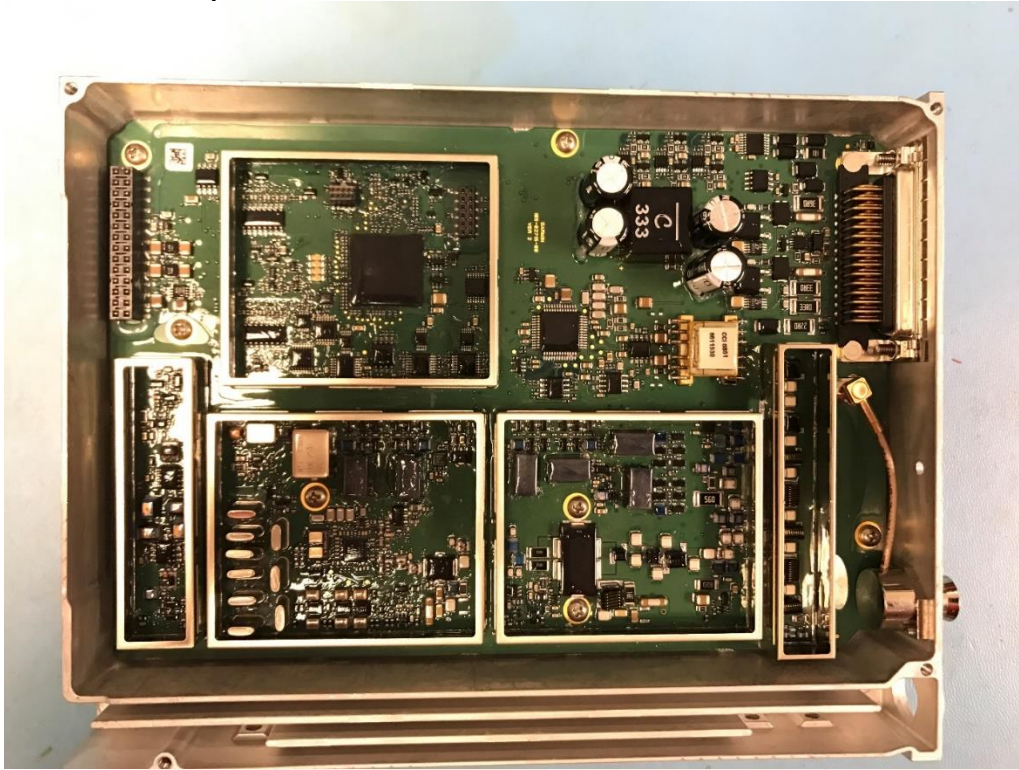
Comm Board top side
