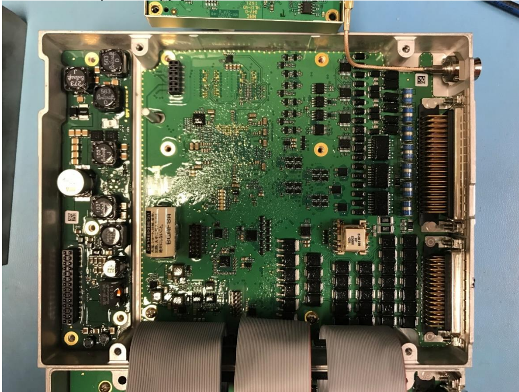
Main Board 2
