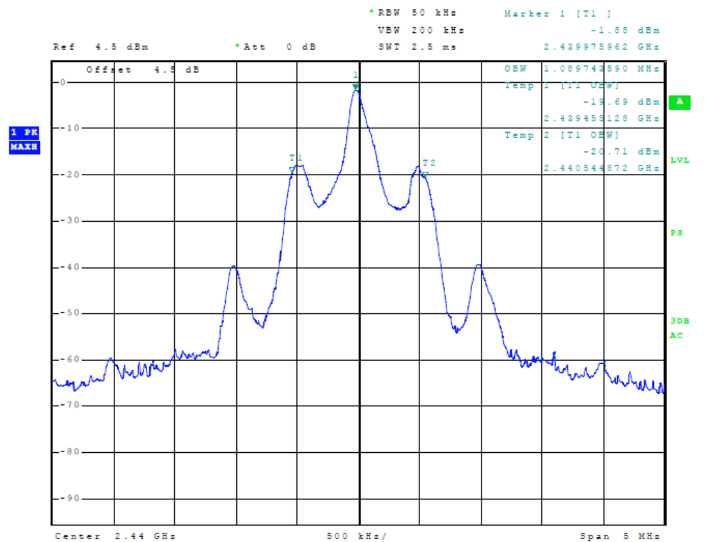
Figure 12 Plot of Transmitter Emissions (2402-2480 MHz, 99% Occupied Bandwidth)
