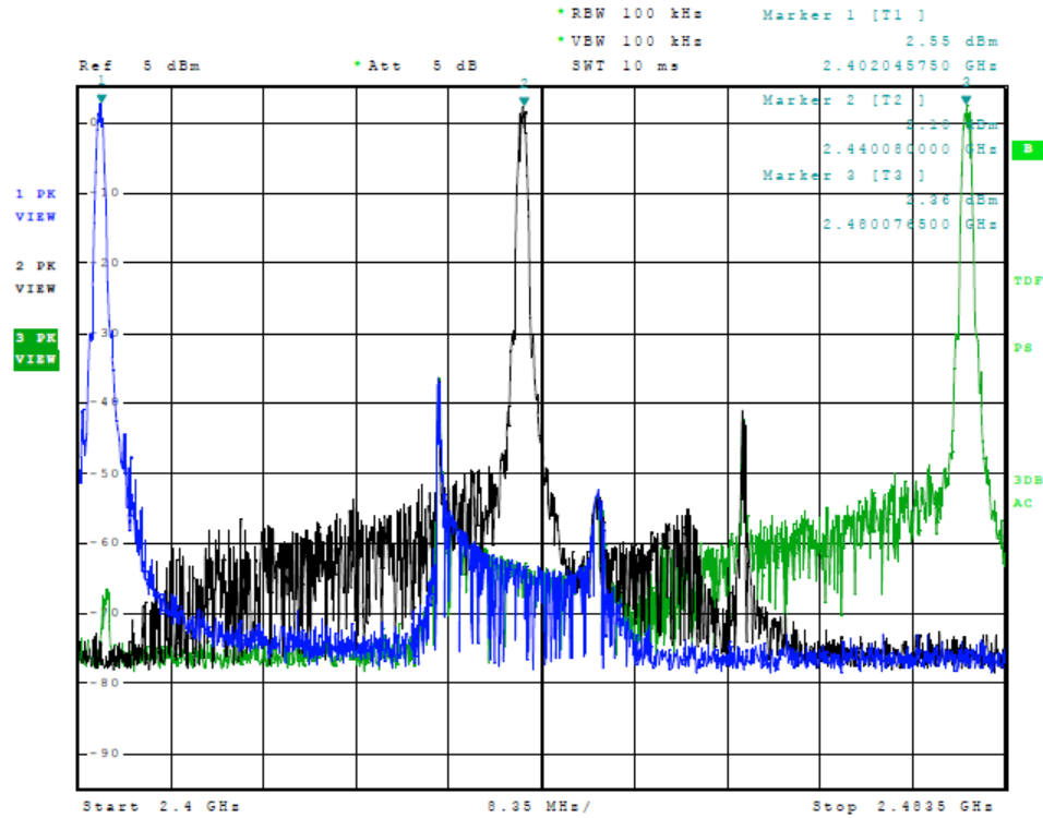
Figure 11 Plot of Transmitter Emissions (In 2402-2480 MHz Band) (Mode 2)
