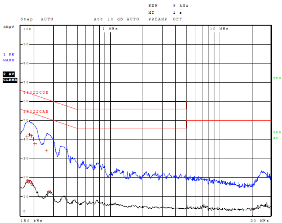
Figure 4 AC Line Conducted emissions of EUT line 2 (EUT AC Adapter, 362-00087-00)
