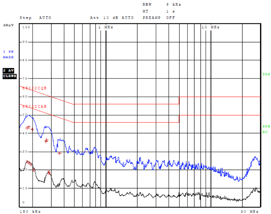
Figure 3 AC Line Conducted emissions of EUT line 2 (EUT AC Adapter, 362-00087-00)
