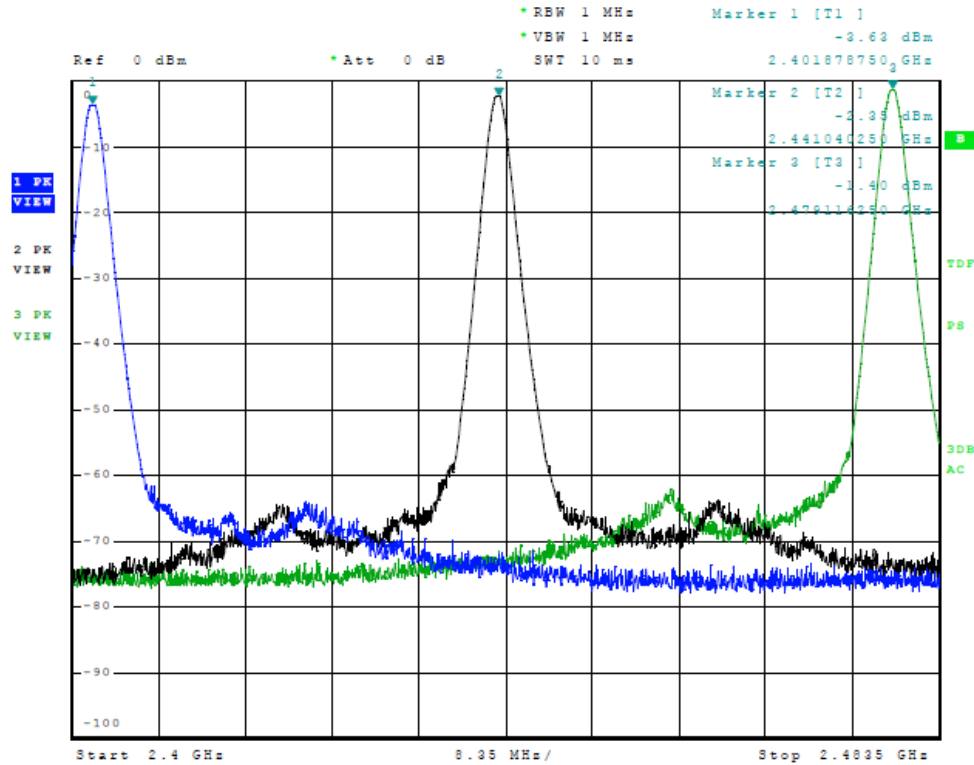
Figure 1 Plot of Transmitter Emissions (In 2402-2479 MHz Band)
