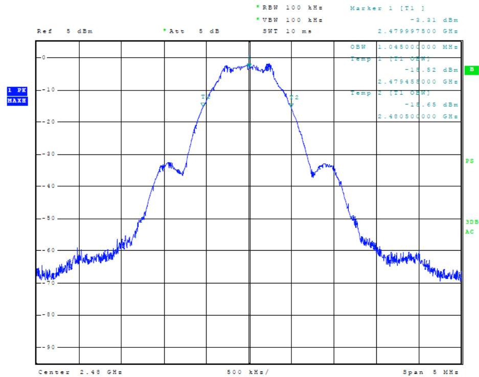
Figure 8 Plot of Transmitter Emissions (99% Occupied Bandwidth, Mode 2)
