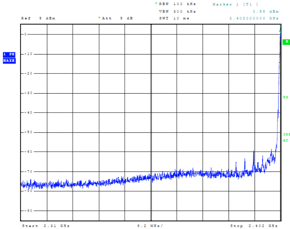
Figure 9 Plot of Transmitter Emissions (Low Band Edge)
