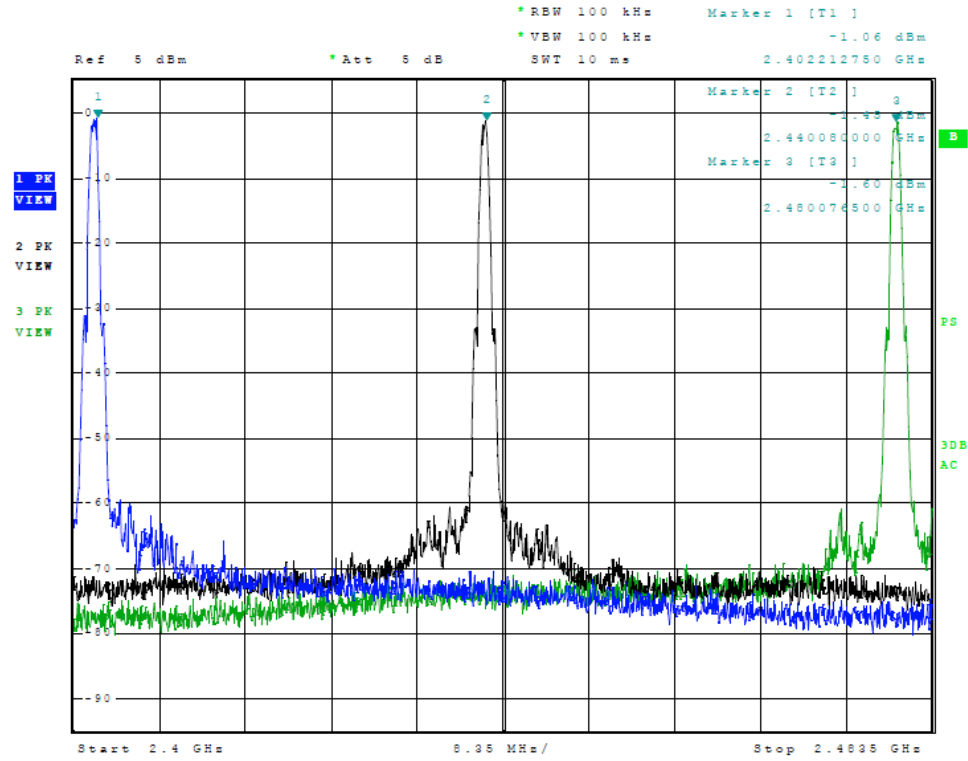
Figure 7 Plot of Transmitter Emissions (In 2402-2480 MHz Band, Mode 2)
