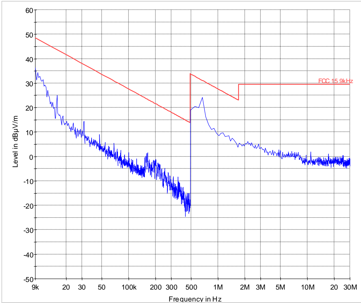
— FCC 15.9kHz.LimitLine — Preview Result 1
