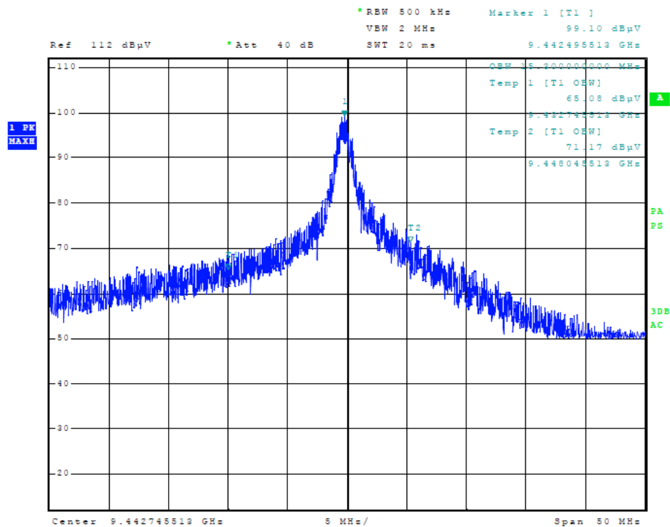
Figure 3 Plot RF power output at 3 meters distance 1/8 nm range
