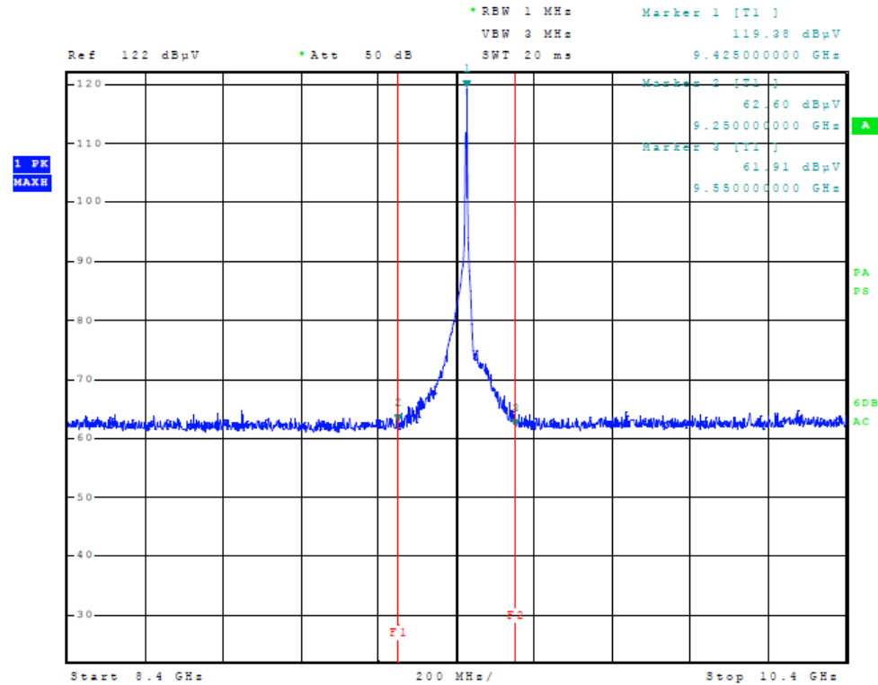
Figure 2 Plot 18 RF power output at 3 meters distance 48 nm range
