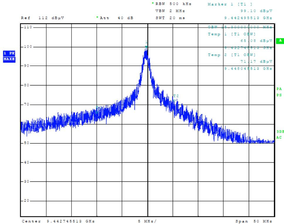
Figure 4 Plot of analyzer screen showing 23-dB occupied bandwidth (1/8 nm)
