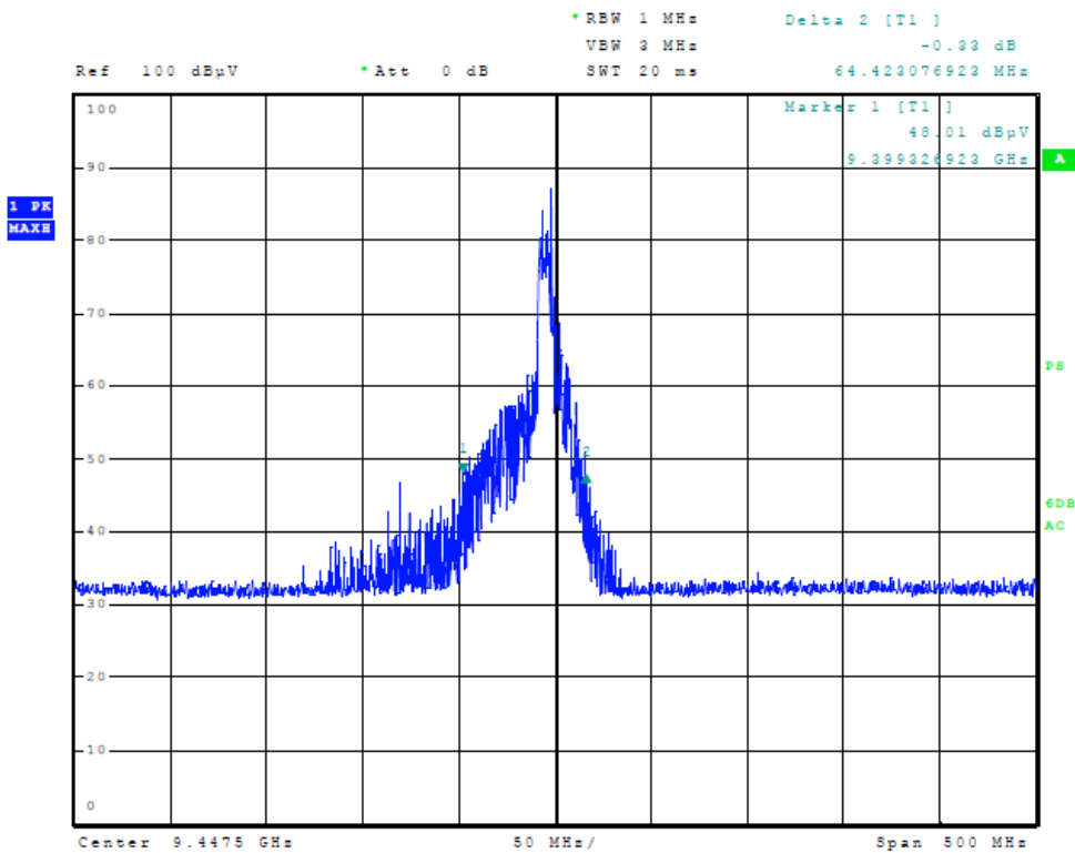
Figure 5 Plot of analyzer screen showing 40-dB occupied bandwidth (1/8 nm)
