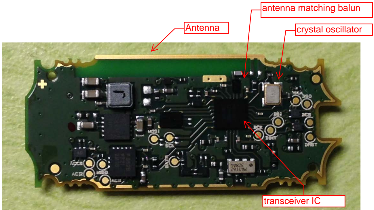
Top of circuit board
