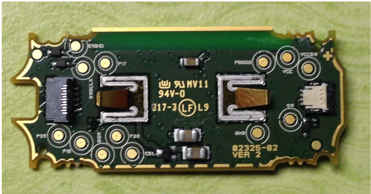
Bottom of circuit board
