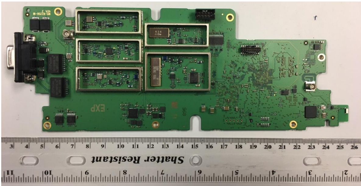
ADSB Board – Top without Shields
