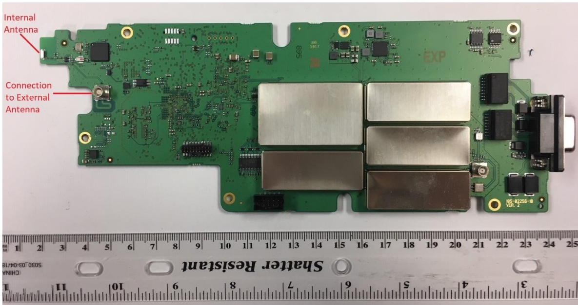
ADSB Board – Top with Shields
