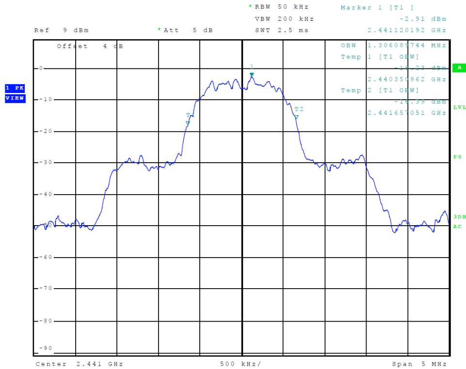
Figure 7 Plot of Transmitter Emissions 99% Occupied Bandwidth (3EDR (8DPSK))
