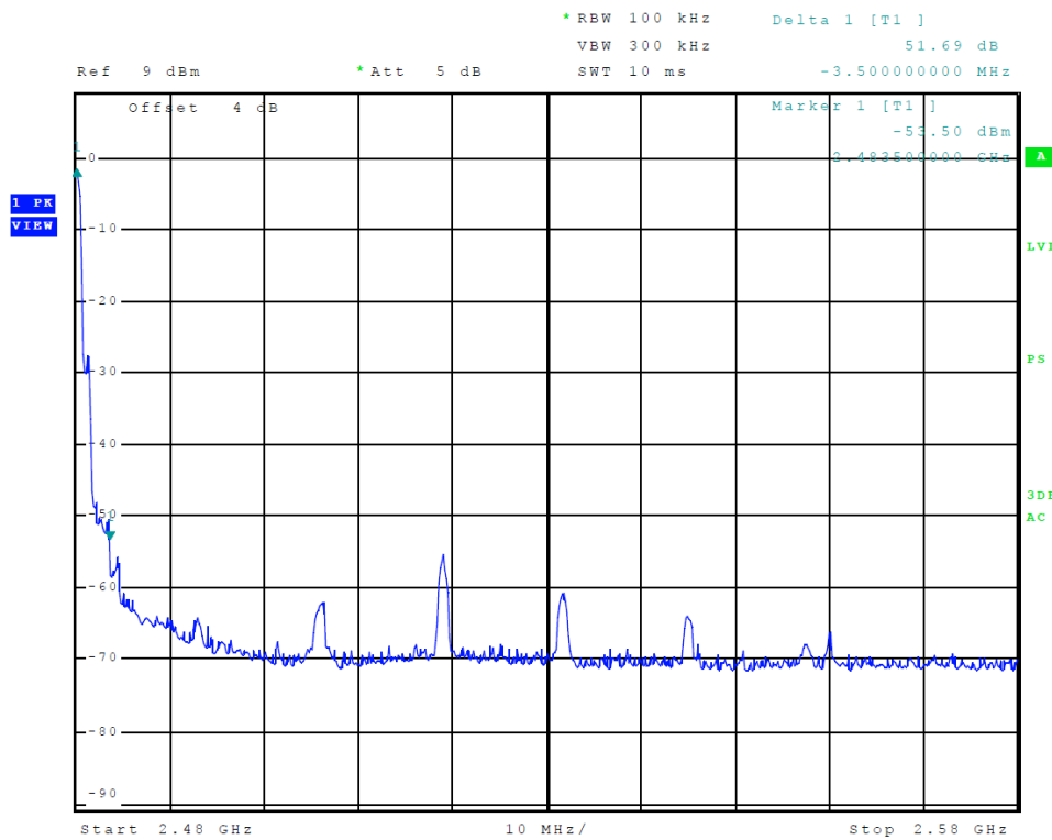
Figure 14 Plot of Transmitter Emissions High Band Edge (2EDR (PI/4 DQPSK))
