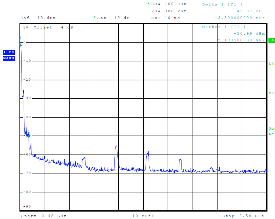
Figure 15 Plot of Transmitter Emissions High Band Edge (3EDR (8DPSK))
