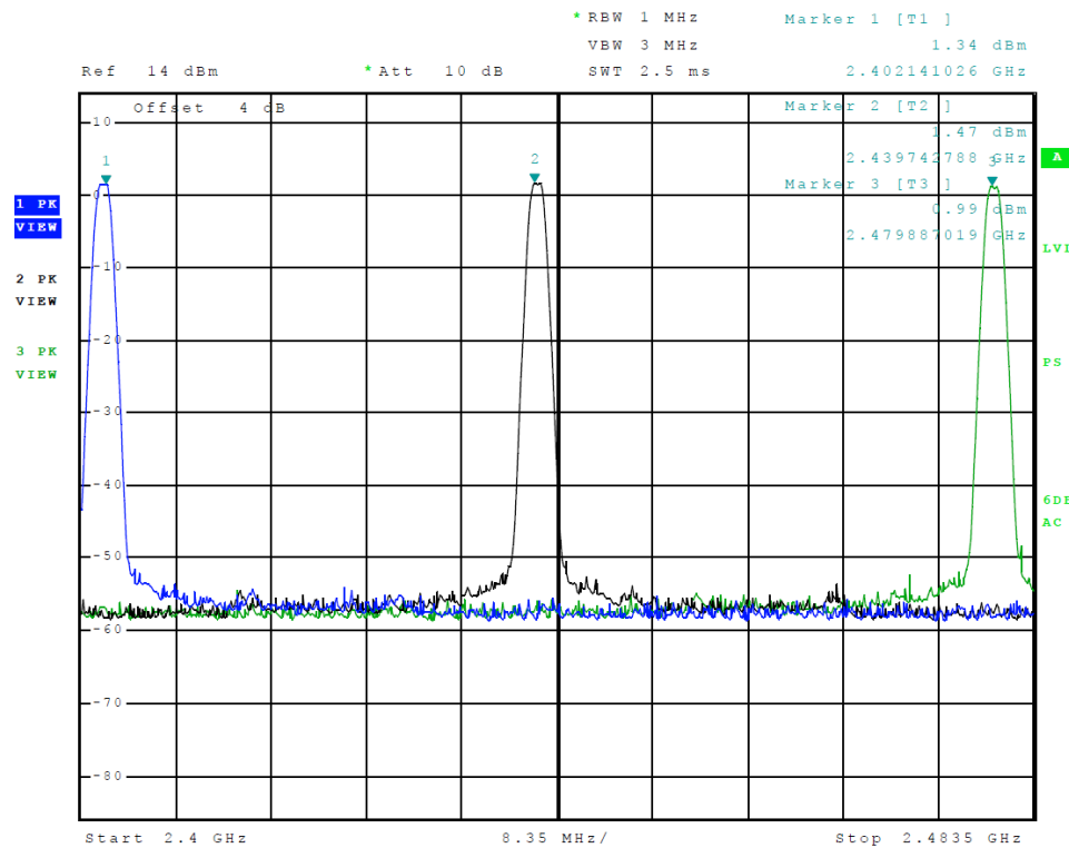
Figure 4 Plot of Transmitter Emissions Operation in 2402-2480 MHz (BLE (GMSK))
