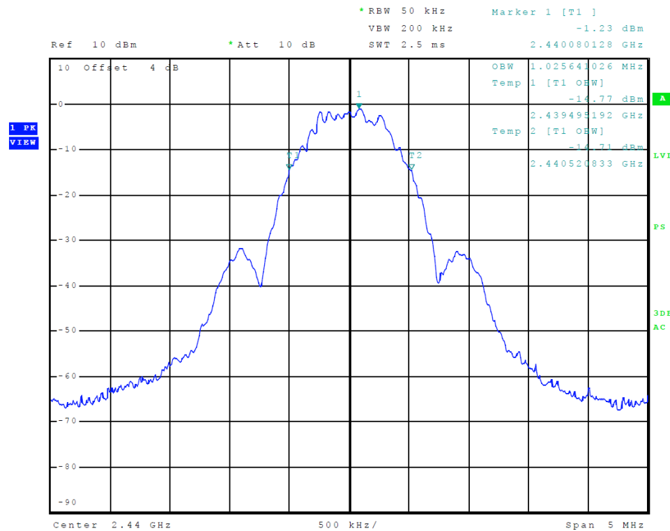
Figure 8 Plot of Transmitter Emissions 99% Occupied Bandwidth (BLE (GMSK))
