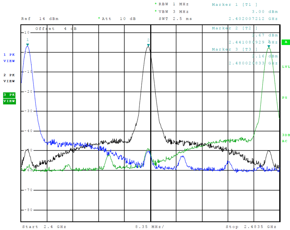
Figure 3 Plot of Transmitter Emissions Operation in 2402-2480 MHz (3EDR (8DPSK))
