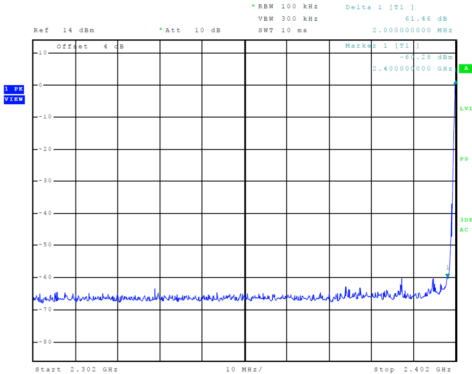
Figure 9 Plot of Transmitter Emissions Low Band Edge (BR (GFSK))
