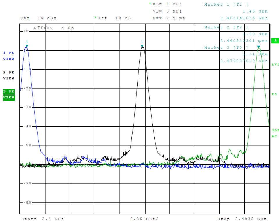
Figure 1 Plot of Transmitter Emissions Operation in 2402-2480 MHz (BR (GFSK))
