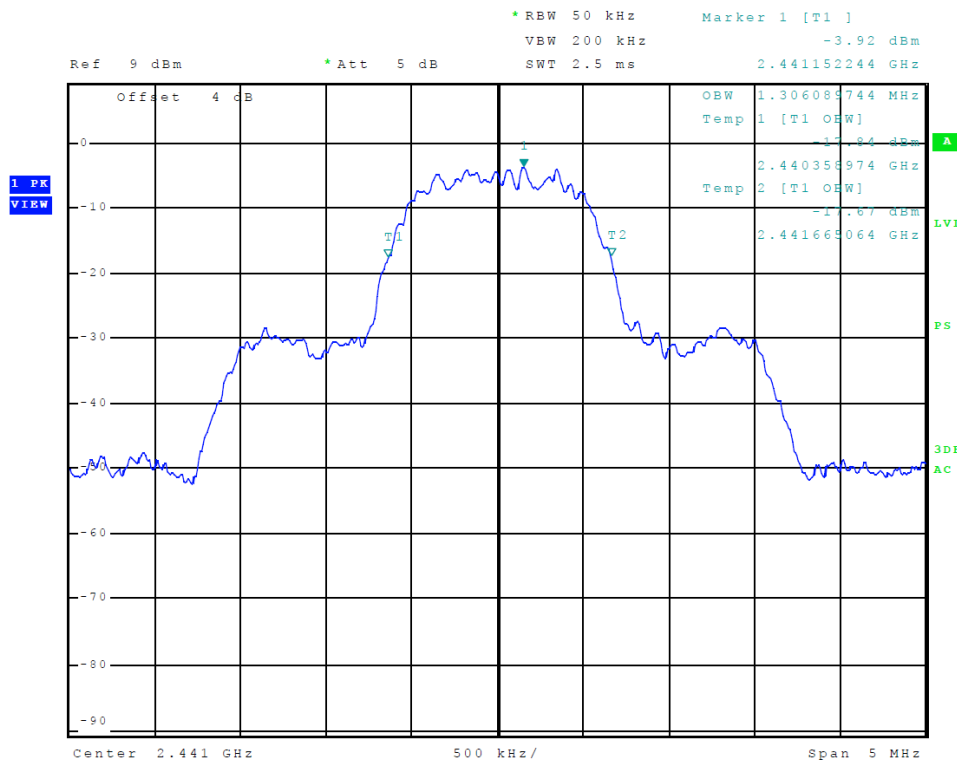
Figure 6 Plot of Transmitter Emissions 99% Occupied Bandwidth (2EDR (PI/4 DQPSK))
