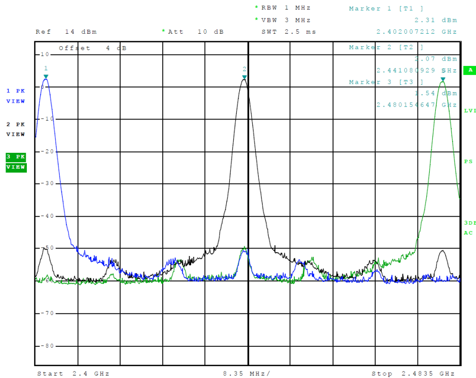
Figure 2 Plot of Transmitter Emissions Operation in 2402-2480 MHz (2EDR (PI/4 DQPSK))
