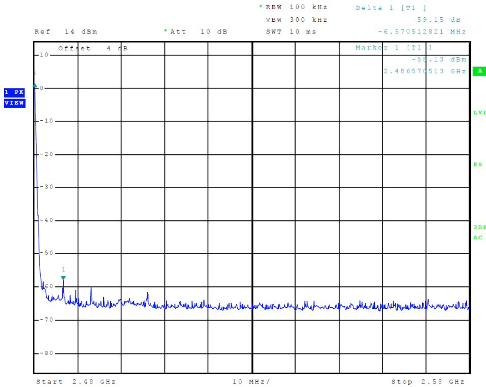
Figure 13 Plot of Transmitter Emissions High Band Edge (BR (GFSK))
