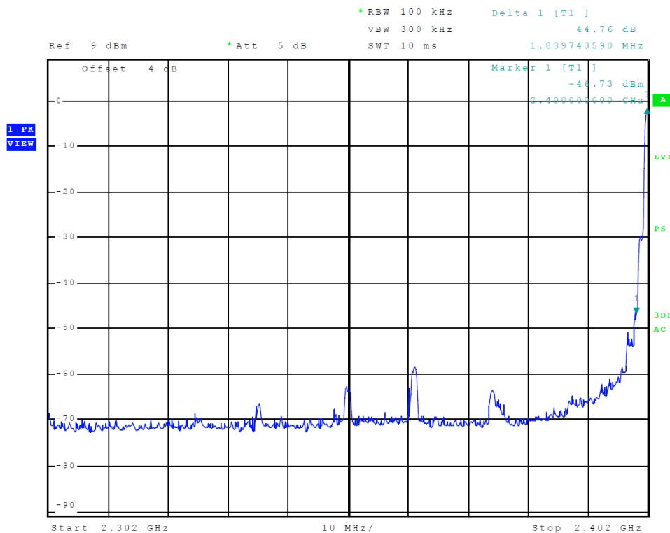
Figure 10 Plot of Transmitter Emissions Low Band Edge (2EDR (PI/4 DQPSK))
