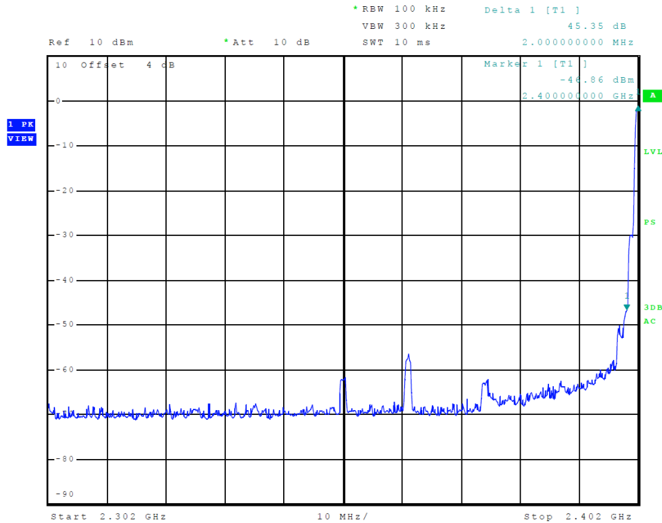
Figure 11 Plot of Transmitter Emissions Low Band Edge (3EDR (8DPSK))
