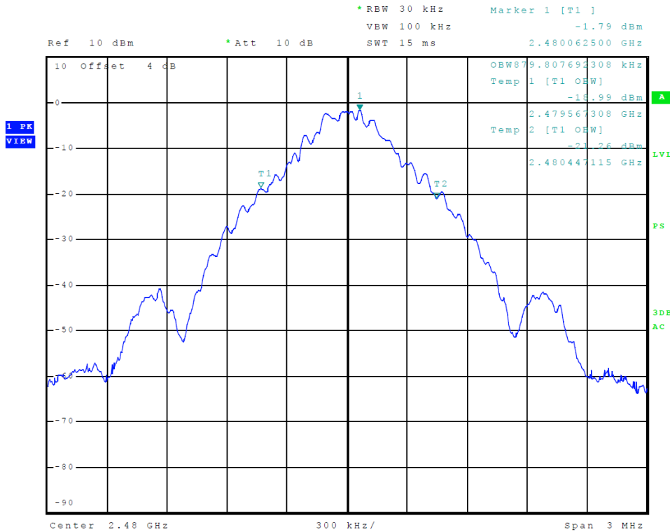
Figure 5 Plot of Transmitter Emissions 99% Occupied Bandwidth (BR (GFSK))
