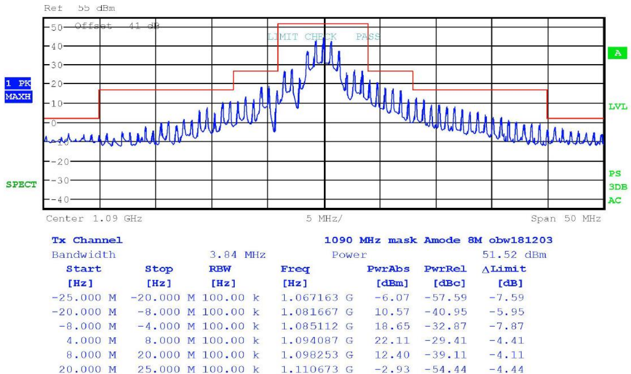
Figure 8 Emissions Mask (Mode-A)
