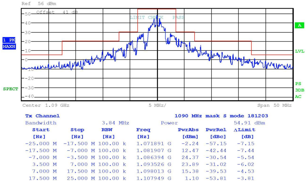
Figure 9 Emissions Mask (Mode-S)
