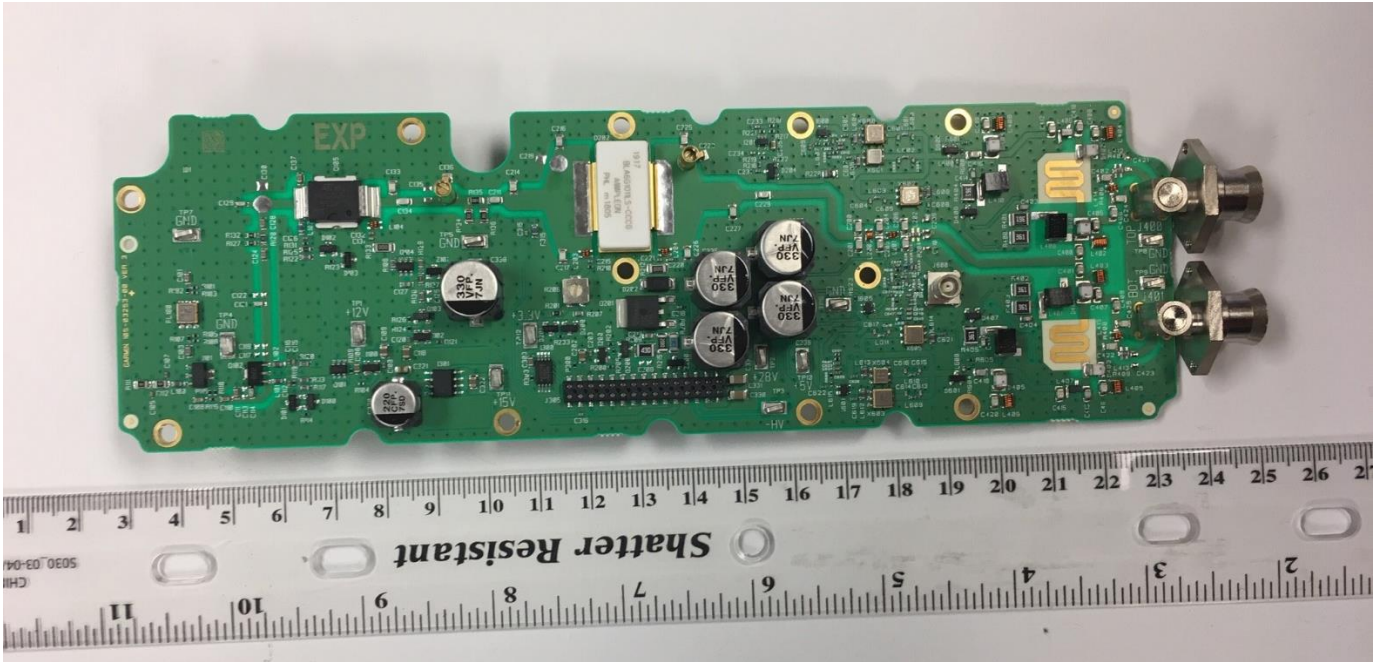
Transponder Board - Top
