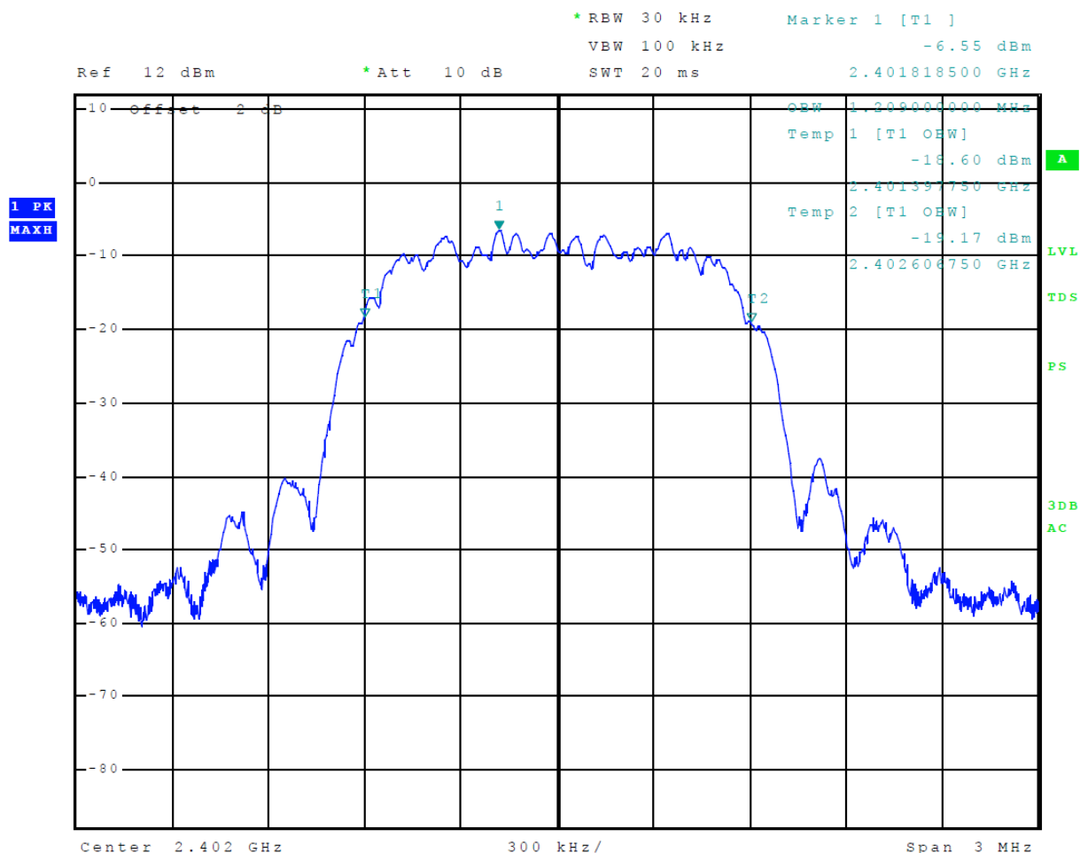
Figure 14 Plot of 99% Occupied Bandwidth Mode 2 BT 2EDR ( \pi/4 -DQPSK)
