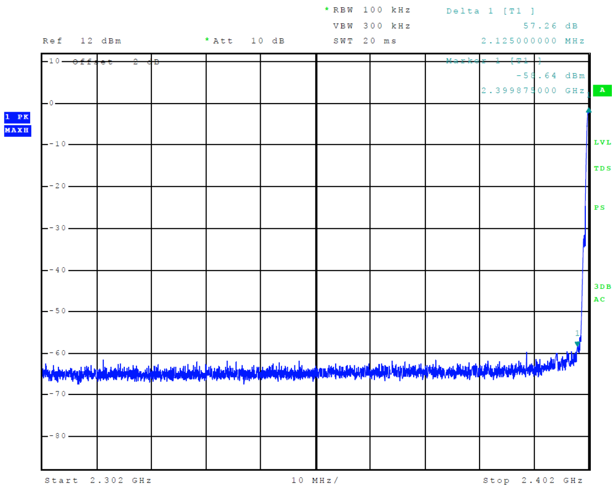
Figure 8 Plot of Transmitter Emissions Low Band Edge Mode 4 BT BLE (GMSK)
