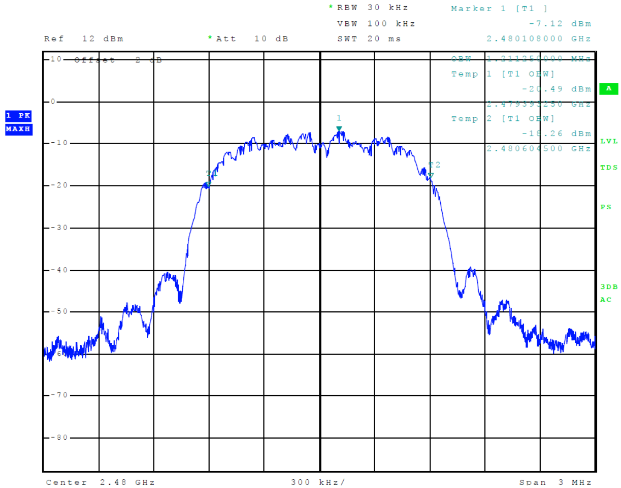
Figure 15 Plot of 99% Occupied Bandwidth Mode 3 BT 3EDR (8DPSK)
