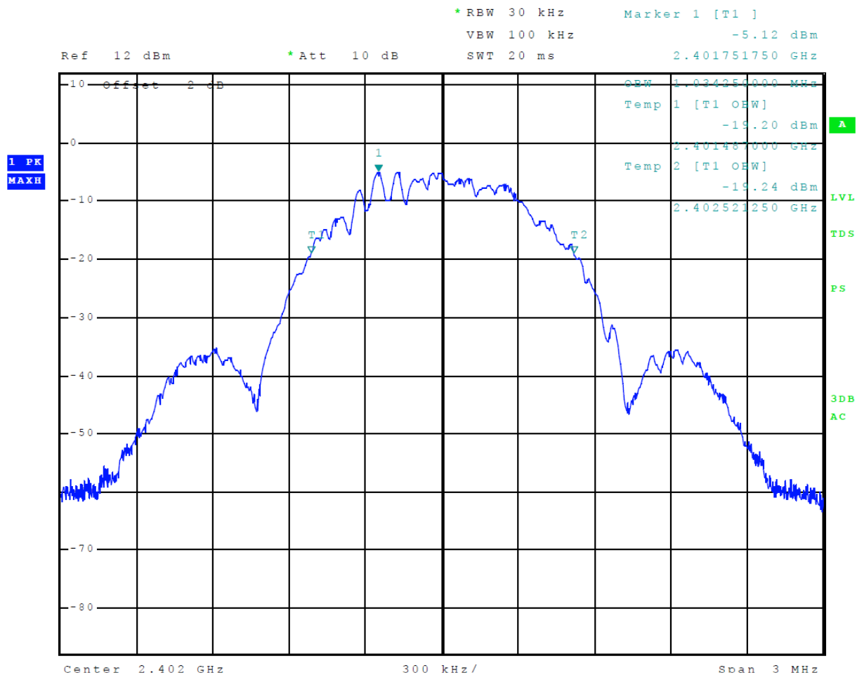
Figure 16 Plot of 99% Occupied Bandwidth Mode 4 BT BLE (GMSK)
