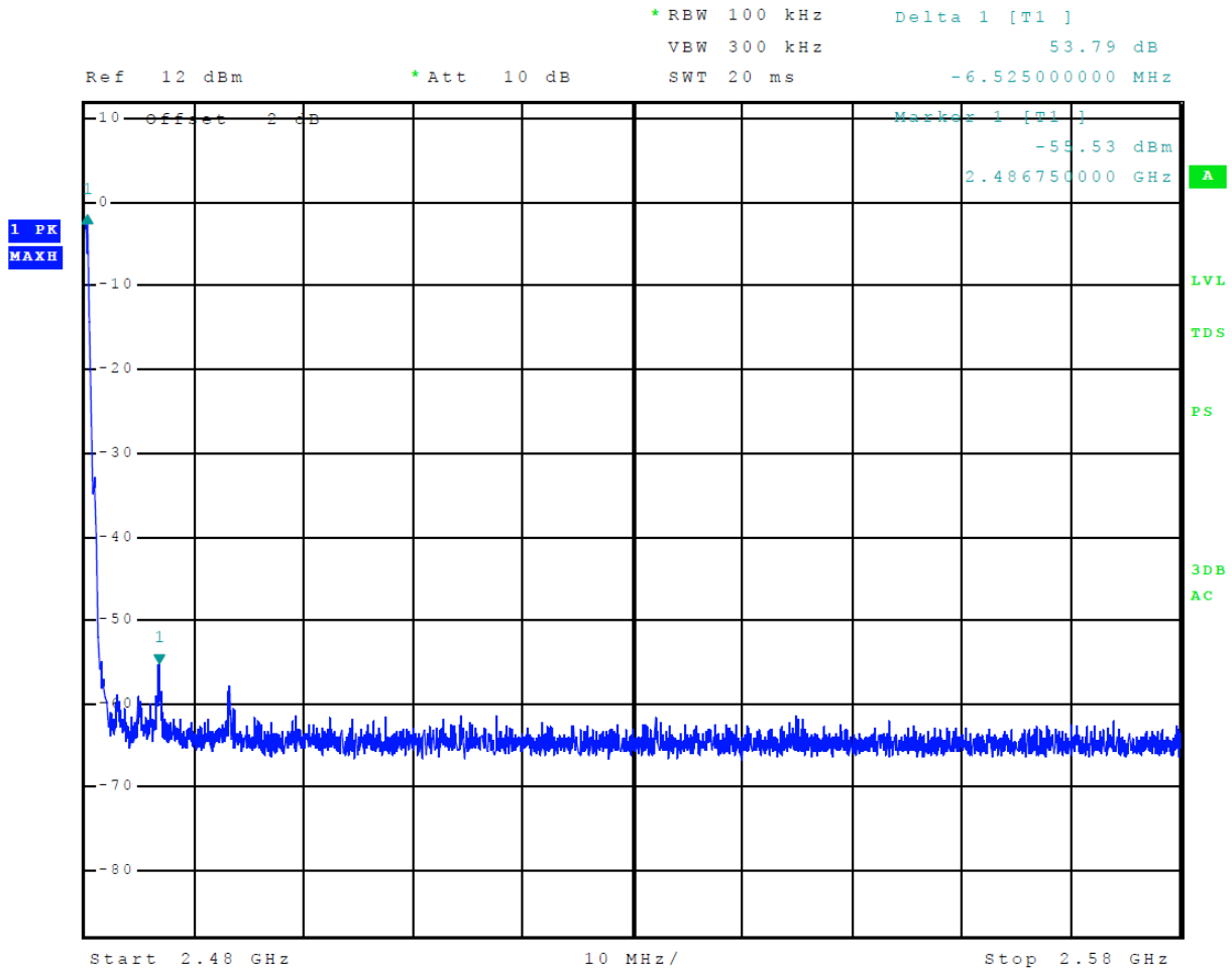
Figure 9 Plot of Transmitter Emissions High Band Edge Mode 1 BT BR (GFSK)
