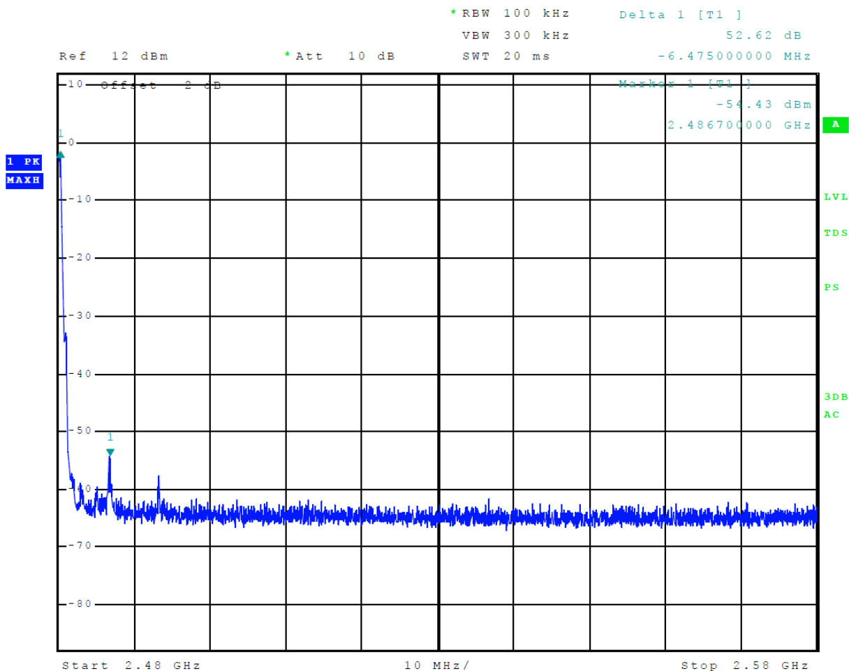
Figure 11 Plot of Transmitter Emissions High Band Edge Mode 3 BT 3EDR (8DPSK)
