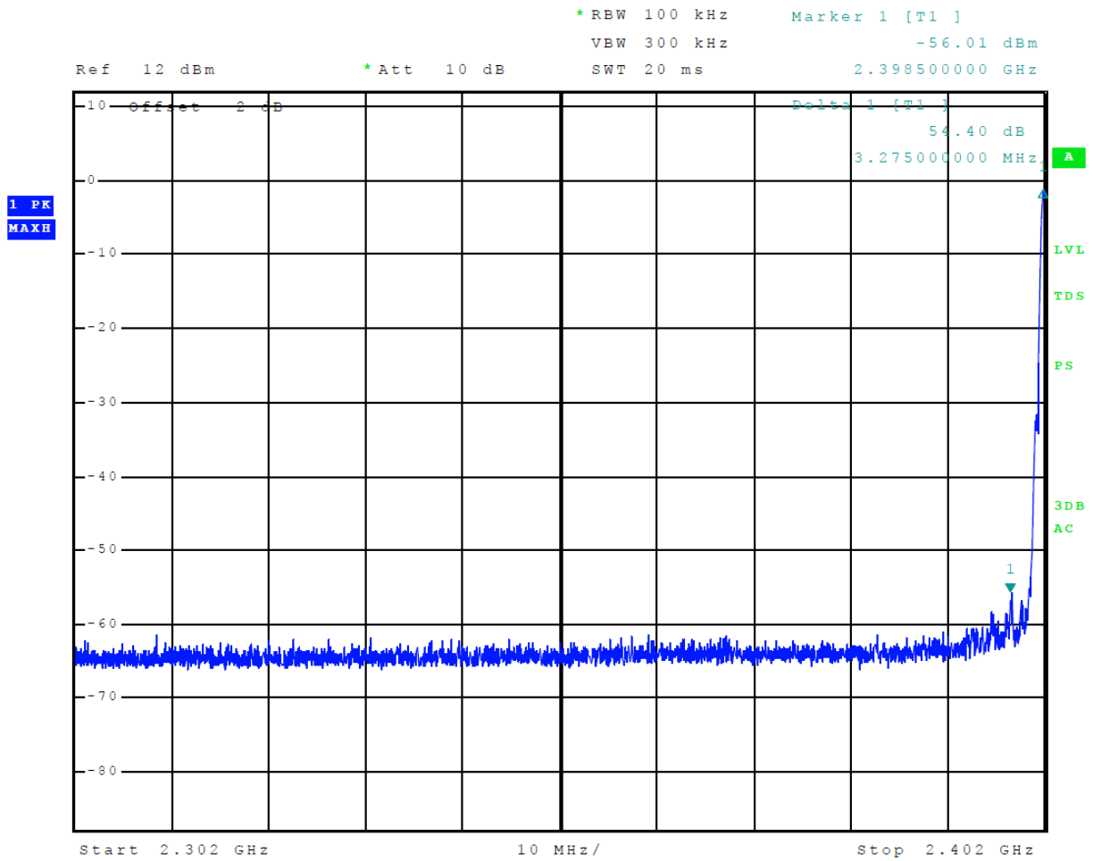
Figure 5 Plot of Transmitter Emissions Low Band Edge Mode 1 BT BR (GFSK)
