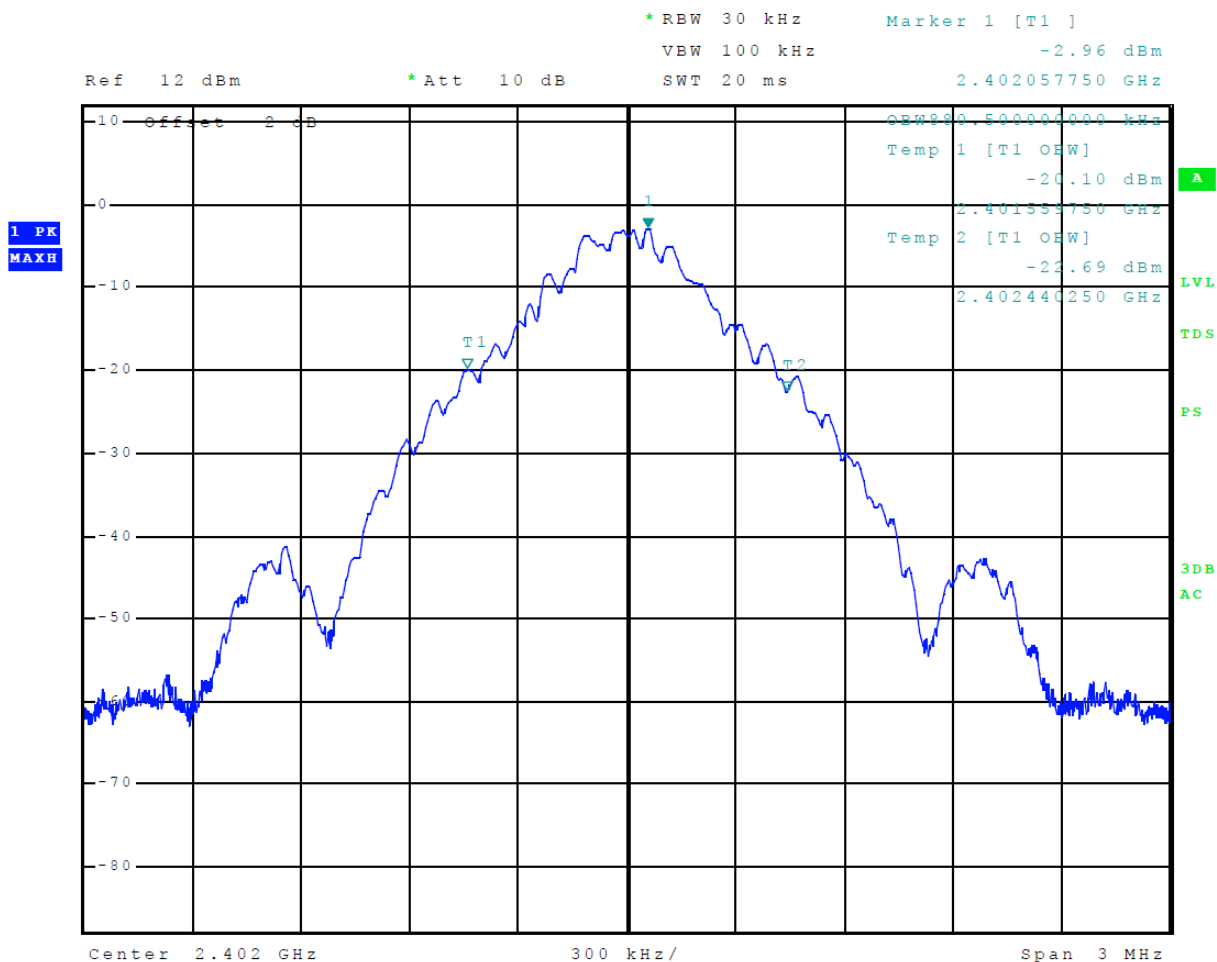
Figure 13 Plot of 99% Occupied Bandwidth Mode 1 BT BR (GFSK)
