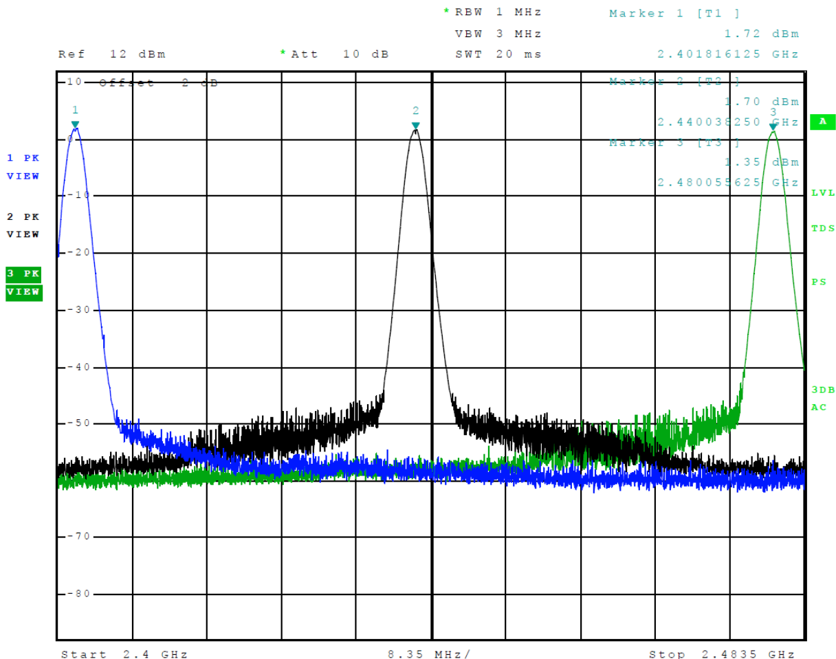
Figure 3 Plot of Transmitter Emissions in 2402-2480 MHz Mode 3 BT 3EDR (8DPSK)
