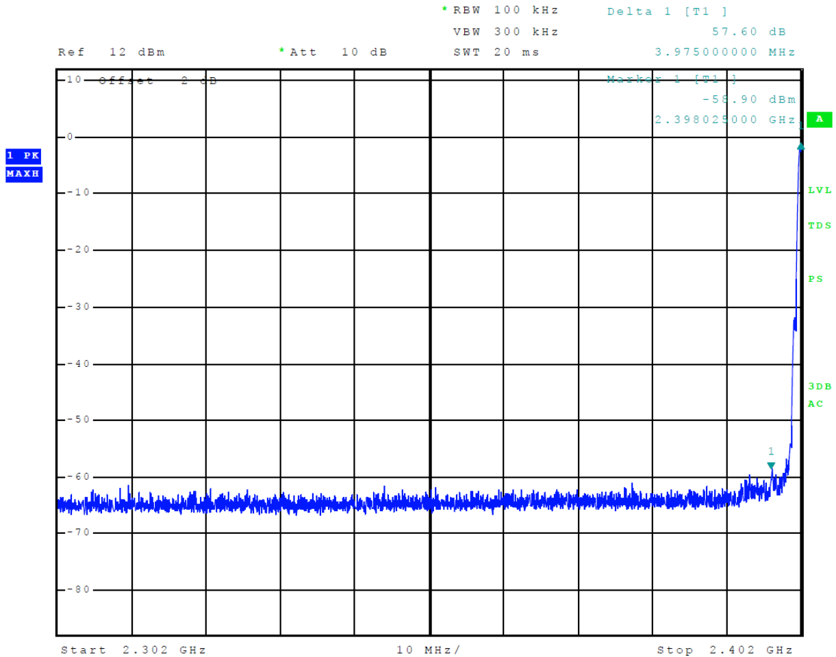
Figure 7 Plot of Transmitter Emissions Low Band Edge Mode 3 BT 3EDR (8DPSK)
