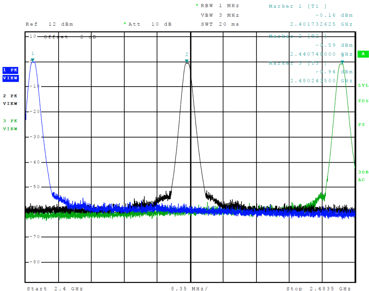
Figure 4 Plot of Transmitter Emissions in 2402-2480 MHz Mode 4 BT BLE (GMSK)
