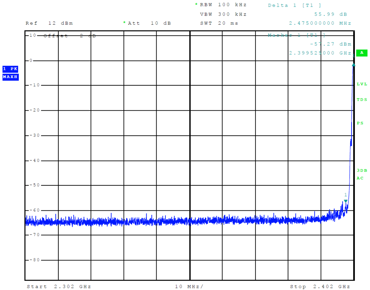
Figure 6 Plot of Transmitter Emissions Low Band Edge Mode 2 BT 2EDR ( \pi/4 -DQPSK)
