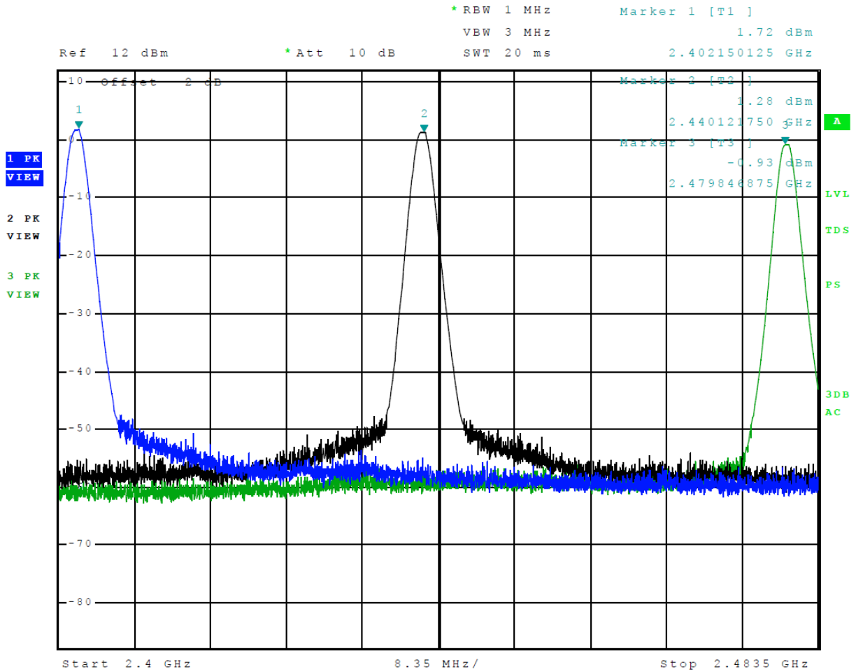
Figure 2 Plot of Transmitter Emissions in 2402-2480 MHz Mode 2 BT 2EDR ( \pi/4 -DQPSK)
