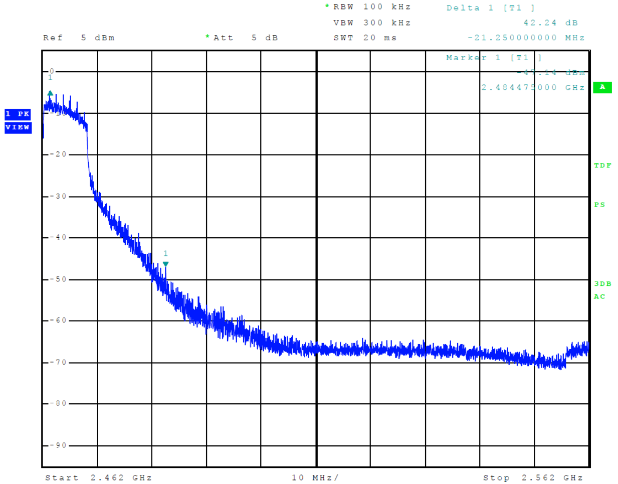
Figure 8 Plot of Transmitter Emissions High Band Edge Mode 6 802.11g
