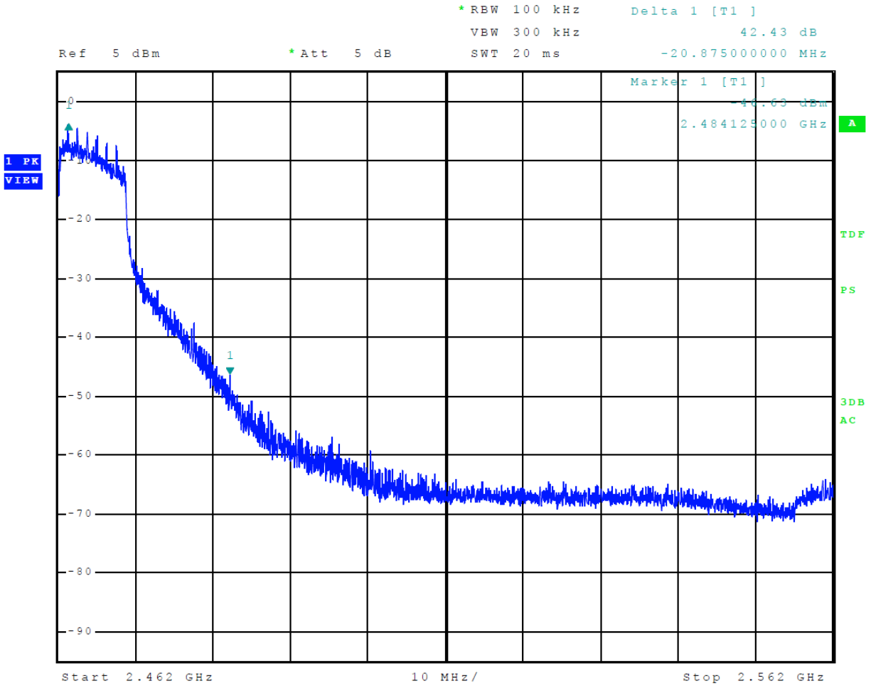
Figure 9 Plot of Transmitter Emissions High Band Edge Mode 7 802.11n
