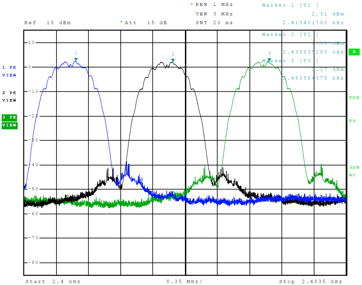
Figure 1 Plot of Transmitter Operation in 2412-2462 MHz Mode 5 802.11b
