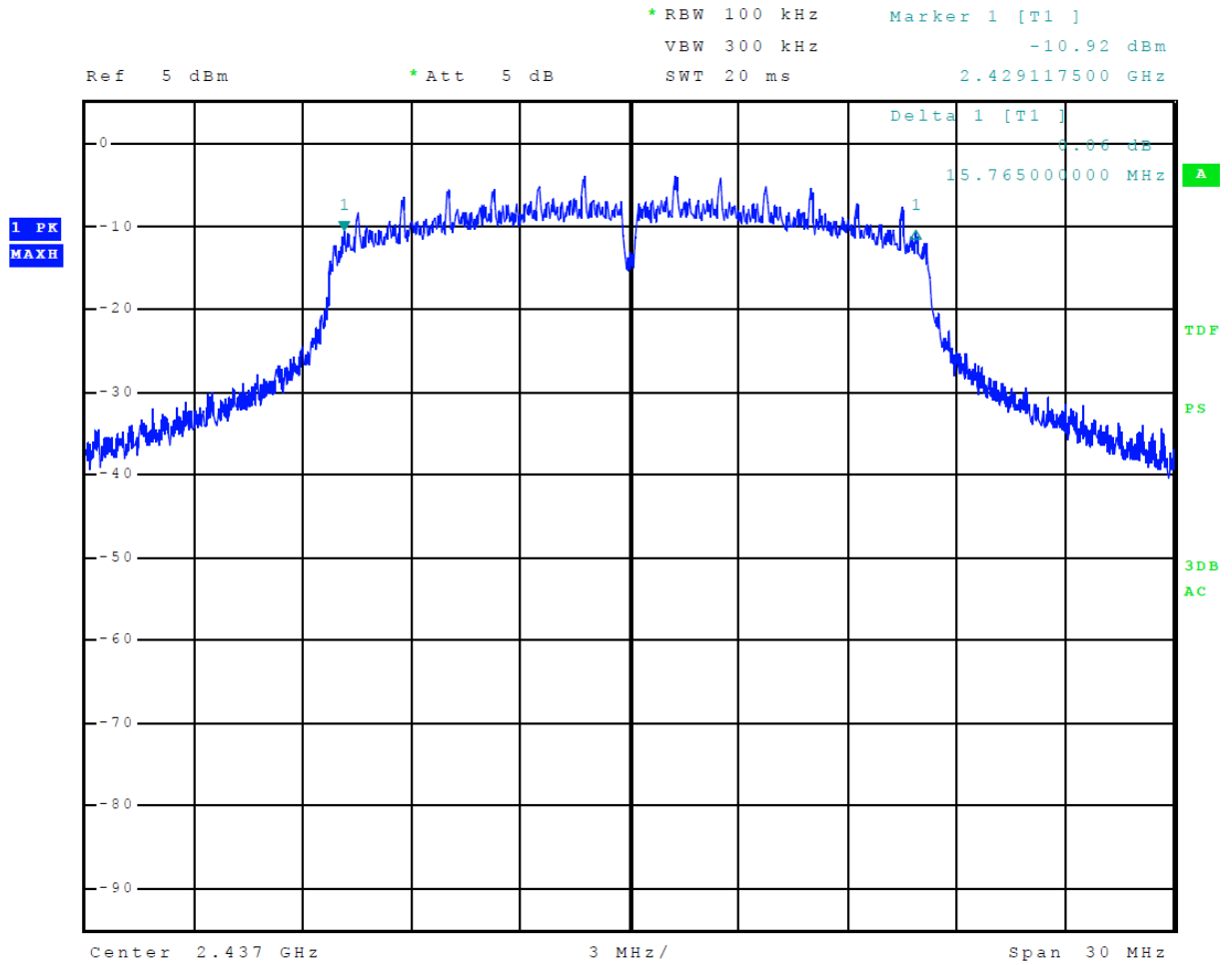
Figure 12 Plot of 6-dB Occupied Bandwidth Mode 6 802.11g
