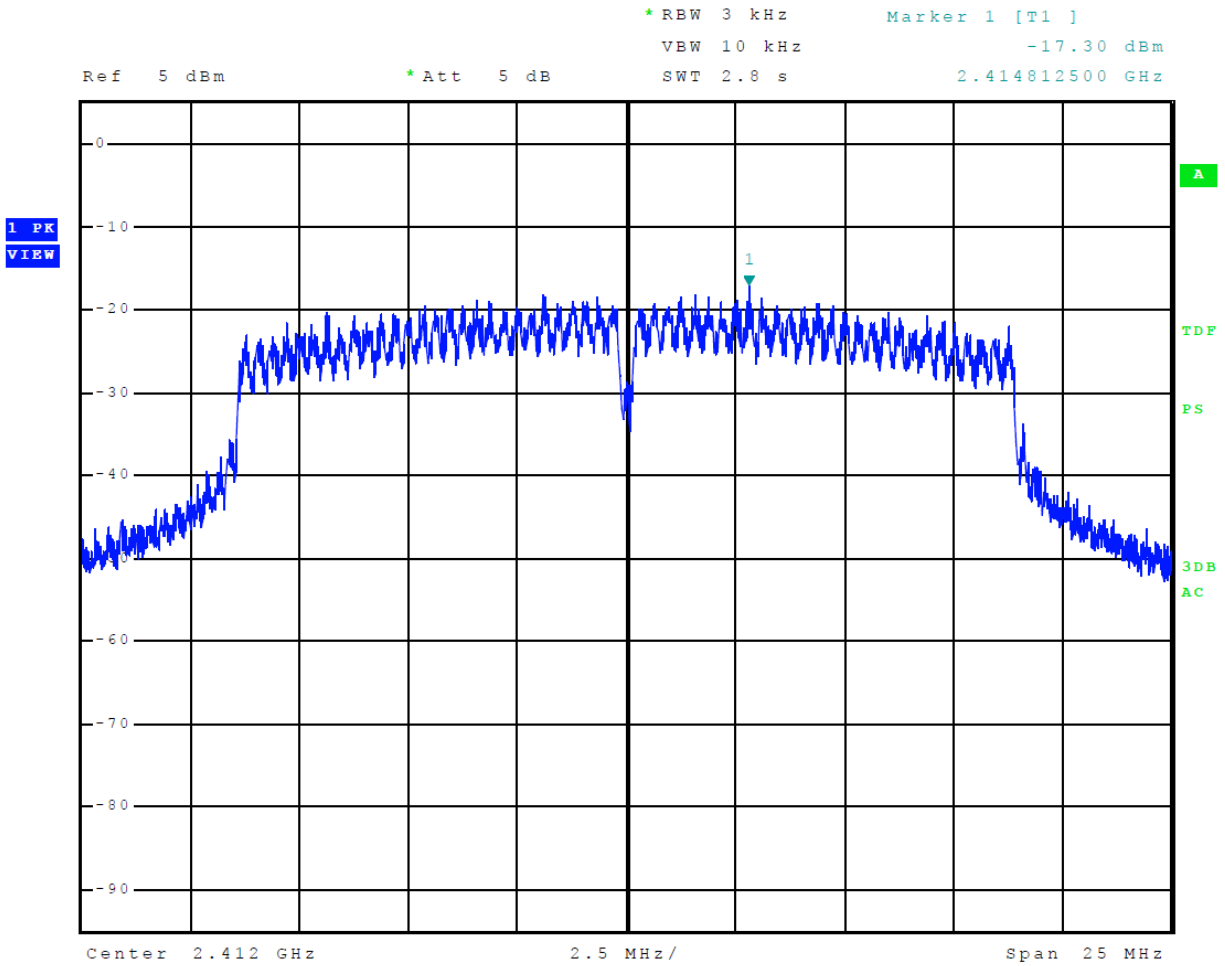
Figure 18 Plot of Transmitter Power Spectral Density Mode 7 802.11n
