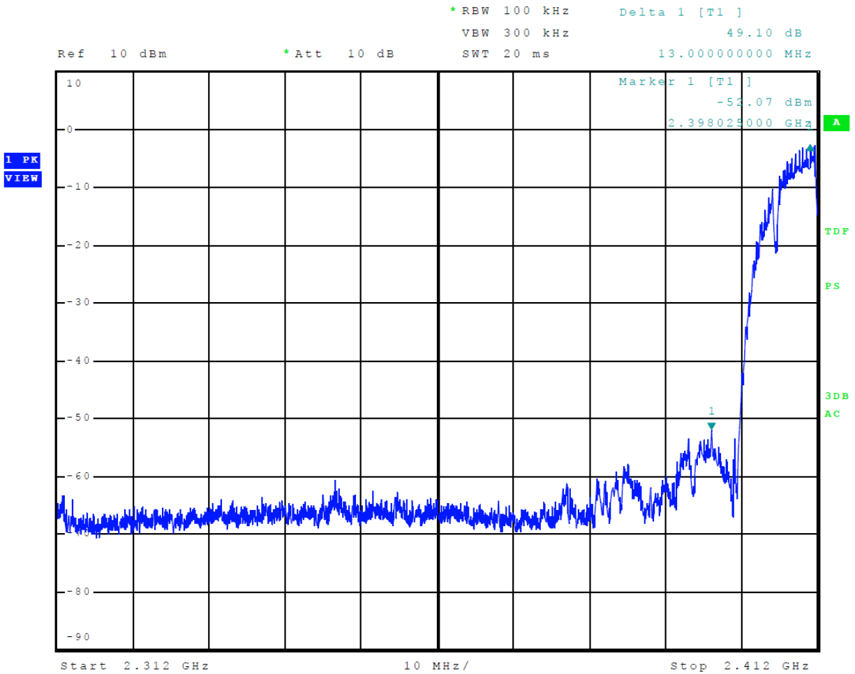
Figure 4 Plot of Transmitter Emissions Low Band Edge Mode 5 802.11b
