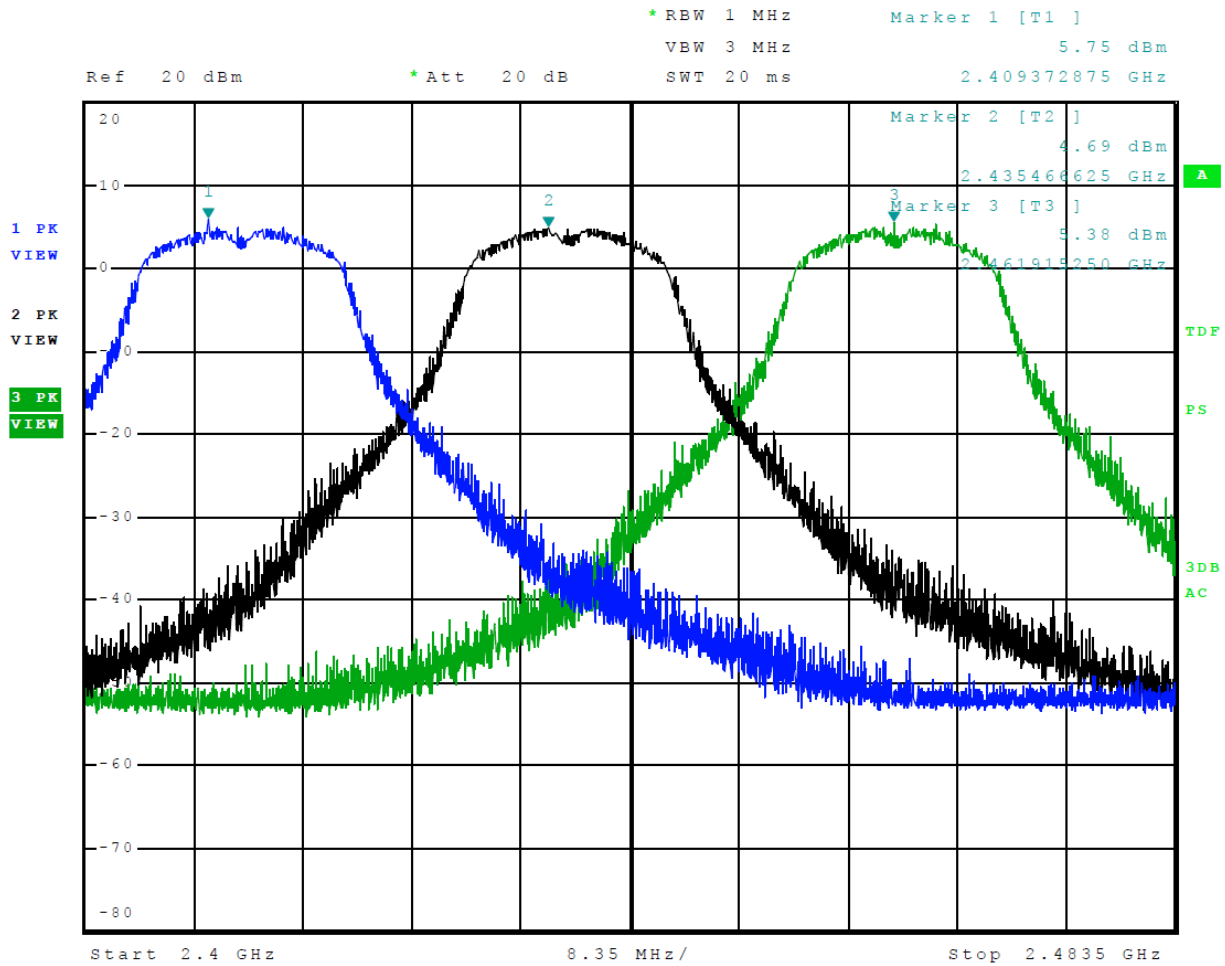
Figure 2 Plot of Transmitter Operation in 2412-2462 MHz Mode 6 802.11g
