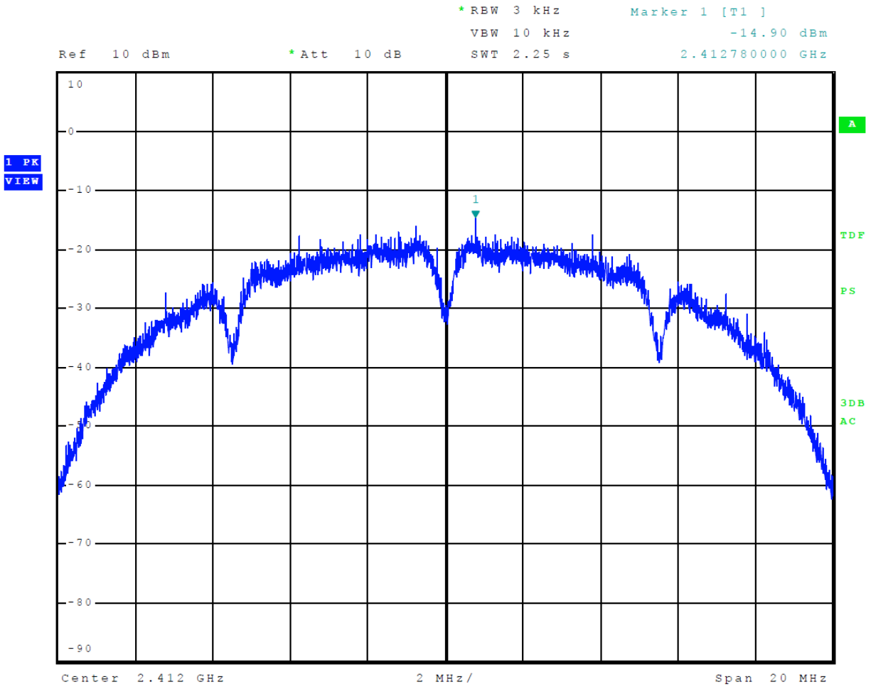
Figure 16 Plot of Transmitter Power Spectral Density Mode 5 802.11b
