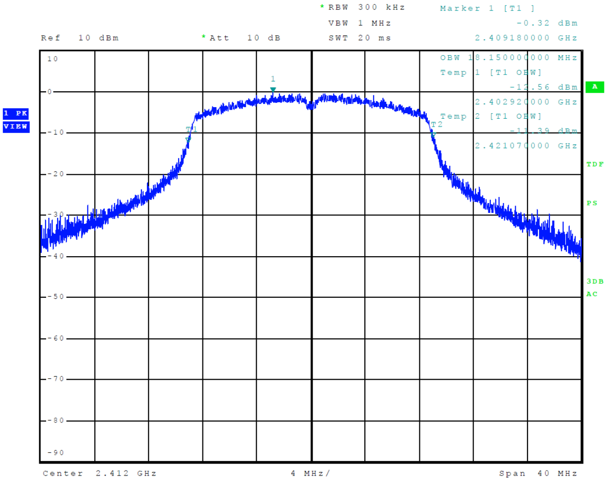
Figure 15 Plot of 99% Occupied Bandwidth Mode 7 802.11n
