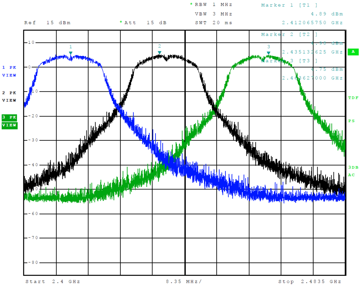
Figure 3 Plot of Transmitter Operation in 2412-2462 MHz Mode 7 802.11n
