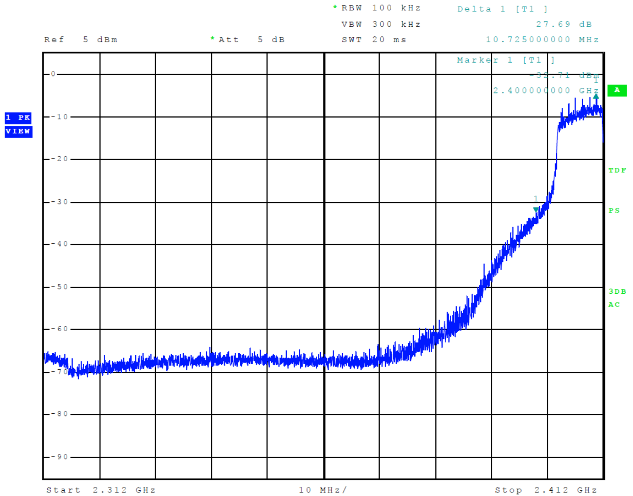
Figure 5 Plot of Transmitter Emissions Low Band Edge Mode 6 802.11g
