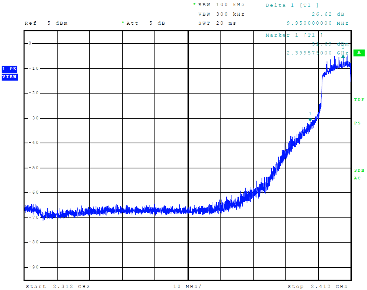
Figure 6 Plot of Transmitter Emissions Low Band Edge Mode 7 802.11n
