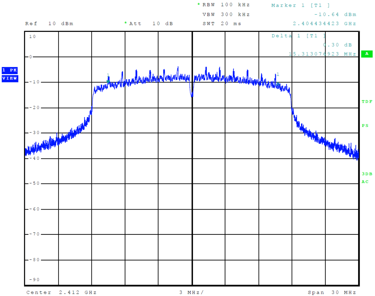
Figure 14 Plot of 6-dB Occupied Bandwidth Mode 7 802.11n
