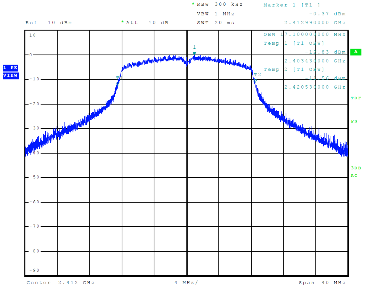
Figure 13 Plot of 99% Occupied Bandwidth Mode 6 802.11g
