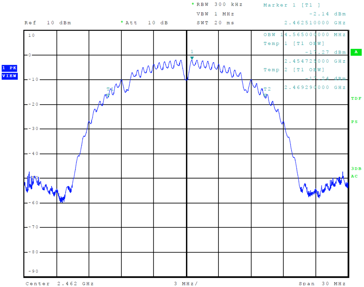
Figure 11 Plot of 99% Occupied Bandwidth Mode 5 802.11b
