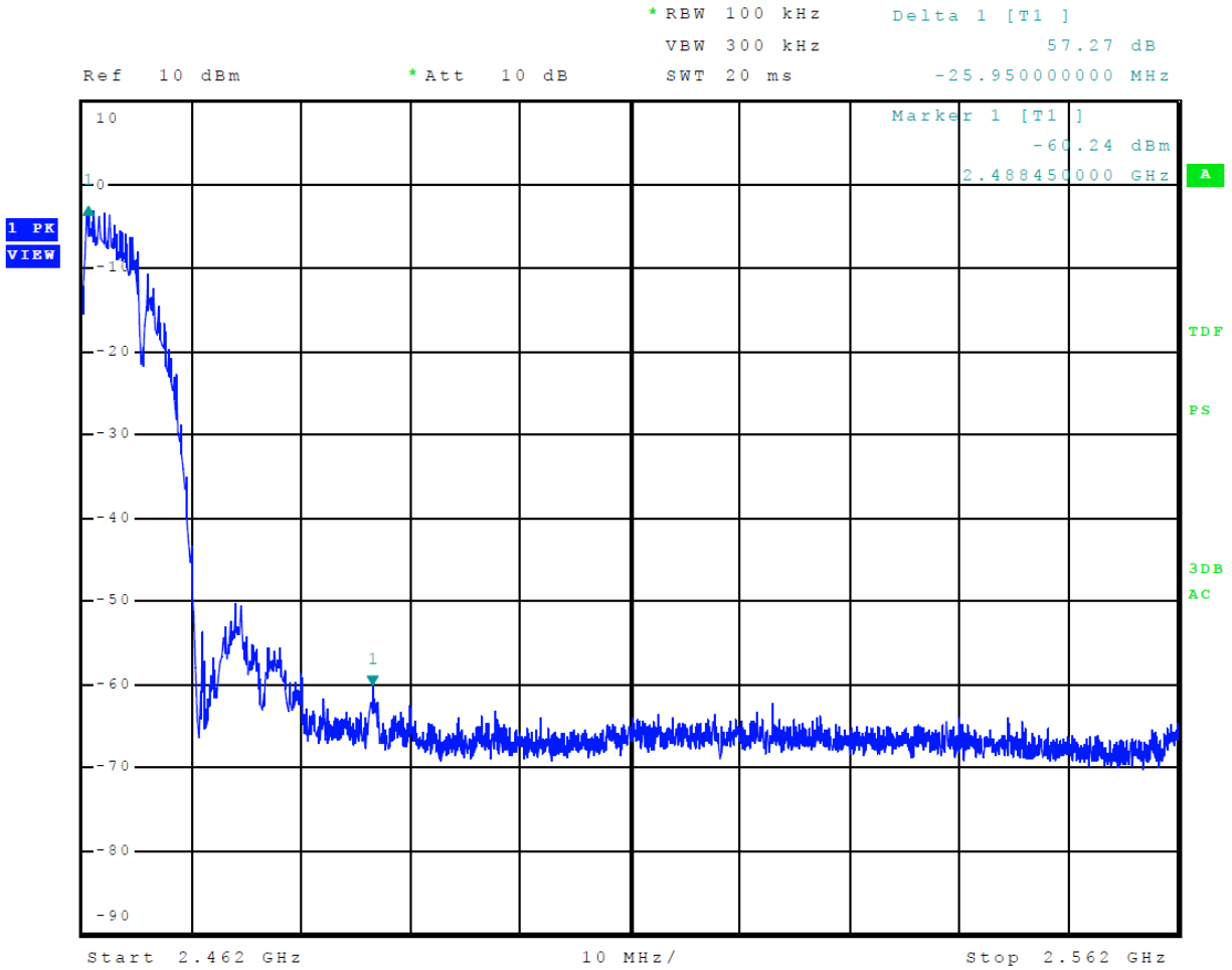
Figure 7 Plot of Transmitter Emissions High Band Edge Mode 5 802.11b
