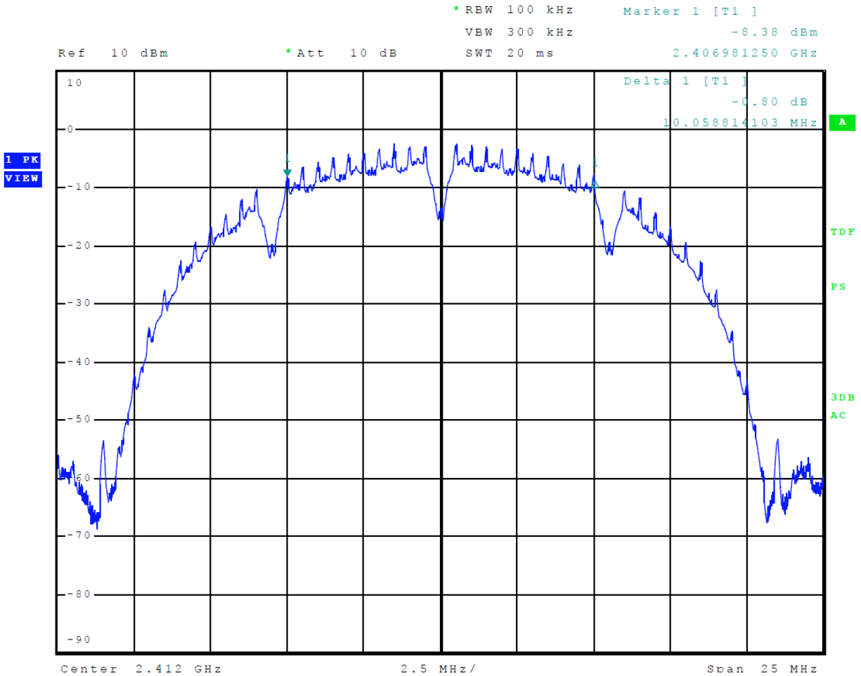
Figure 10 Plot of 6-dB Occupied Bandwidth Mode 5 802.11b
