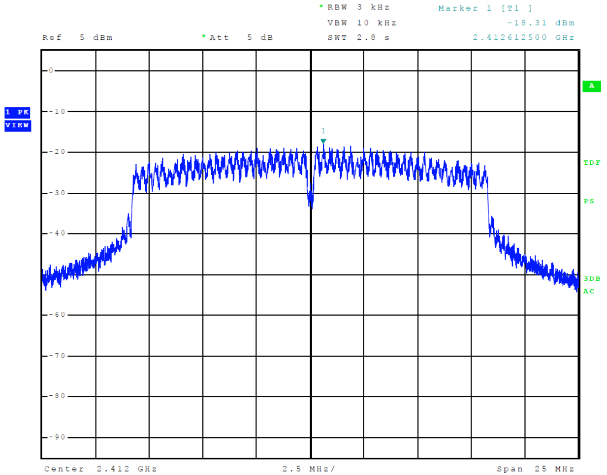
Figure 17 Plot of Transmitter Power Spectral Density Mode 6 802.11g
