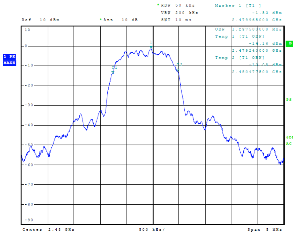
Figure 2 Plot of Transmitter Emissions (2402-2480 MHz, 99% Occupied Bandwidth)
