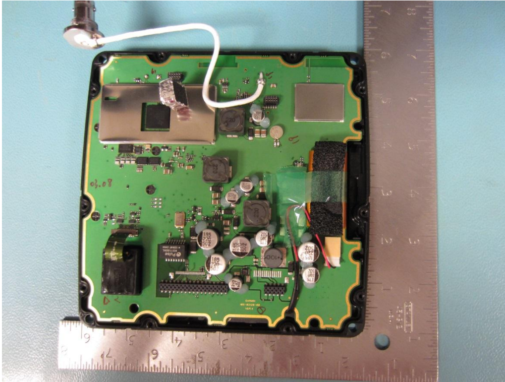
Transmitter board Back
