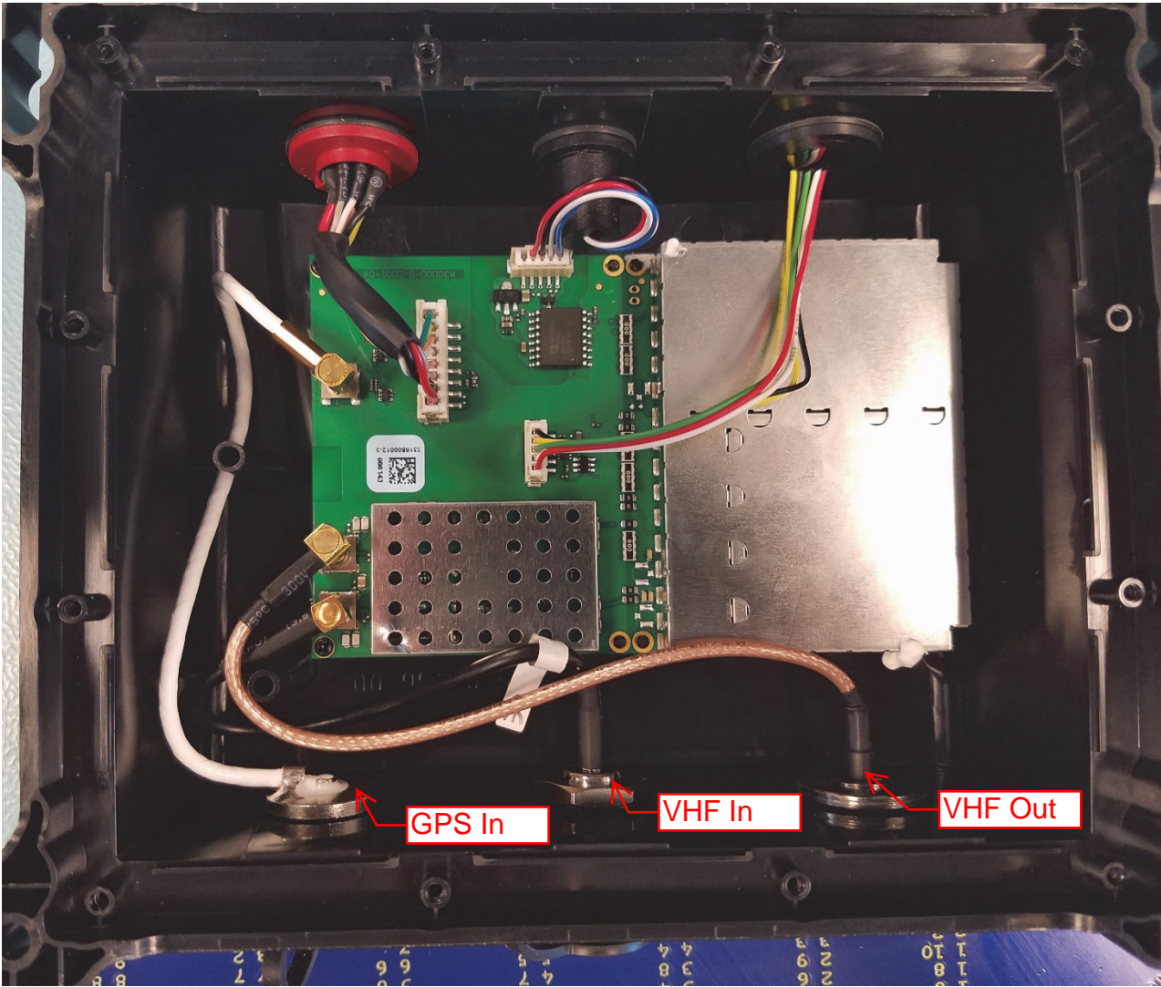
Bottom Cover Removed
