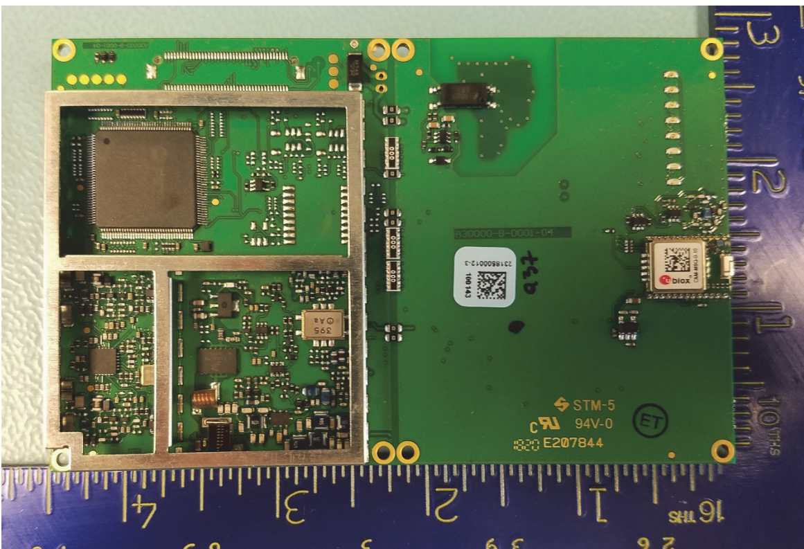
Circuit Board Side 2 – Shield Removed
