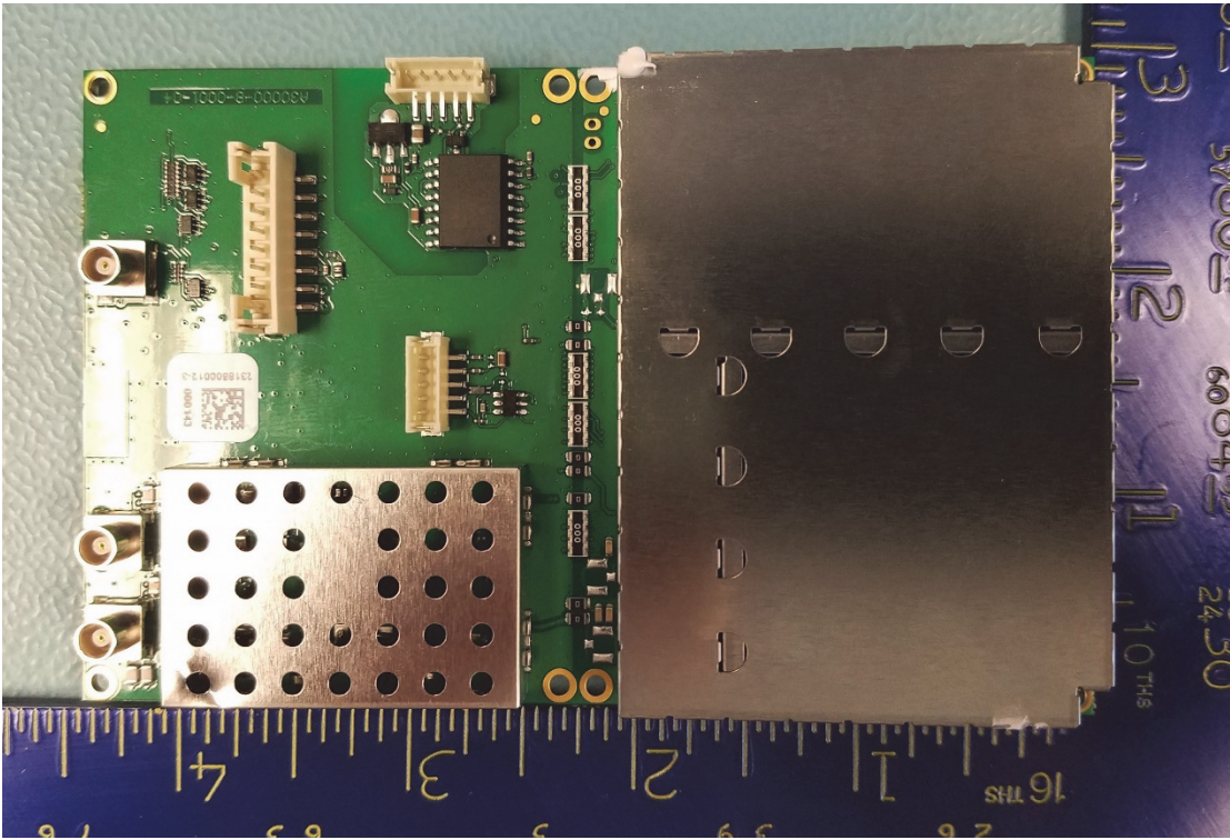
Circuit Board Side 1 – Shields On
