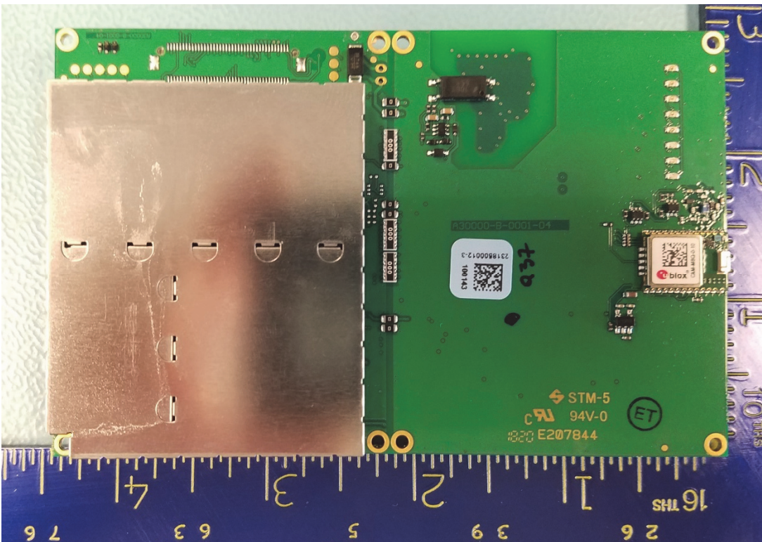
Circuit Board Side 2 – Shield On
