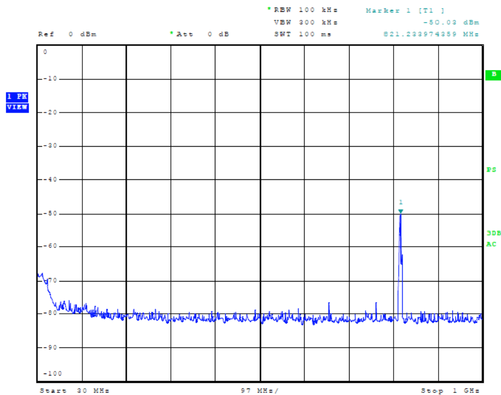
Figure Sixteen Plot of Frequency Spectrum at Temporary Antenna Port
