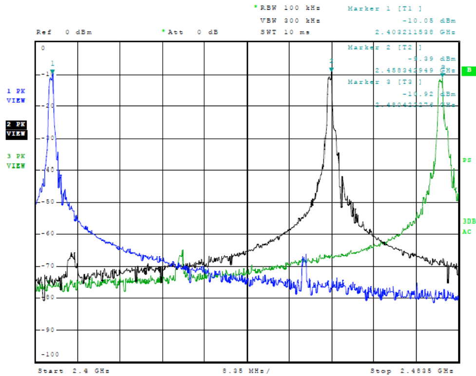
Figure Thirteen Plot of Operation across frequency band
