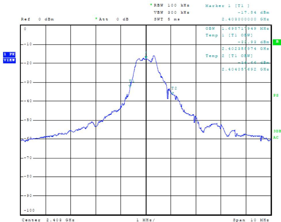
Figure Ten Plot of 99.5% Occupied Bandwidth (Low channel)
