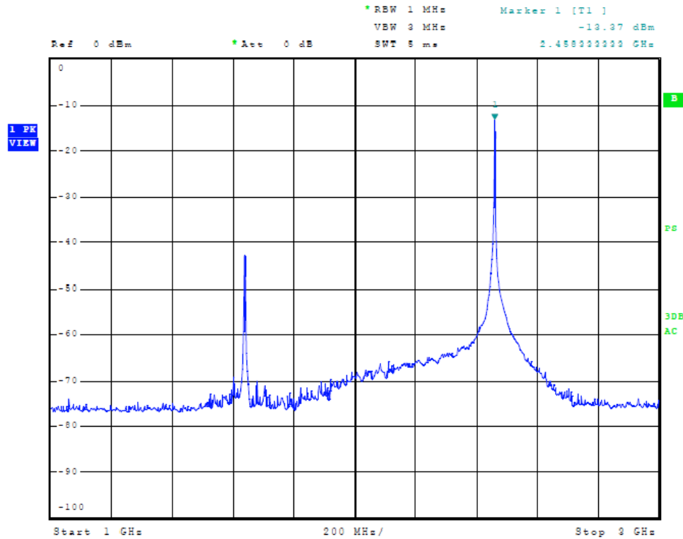
Figure Seventeen Plot of Frequency Spectrum at Temporary Antenna Port
