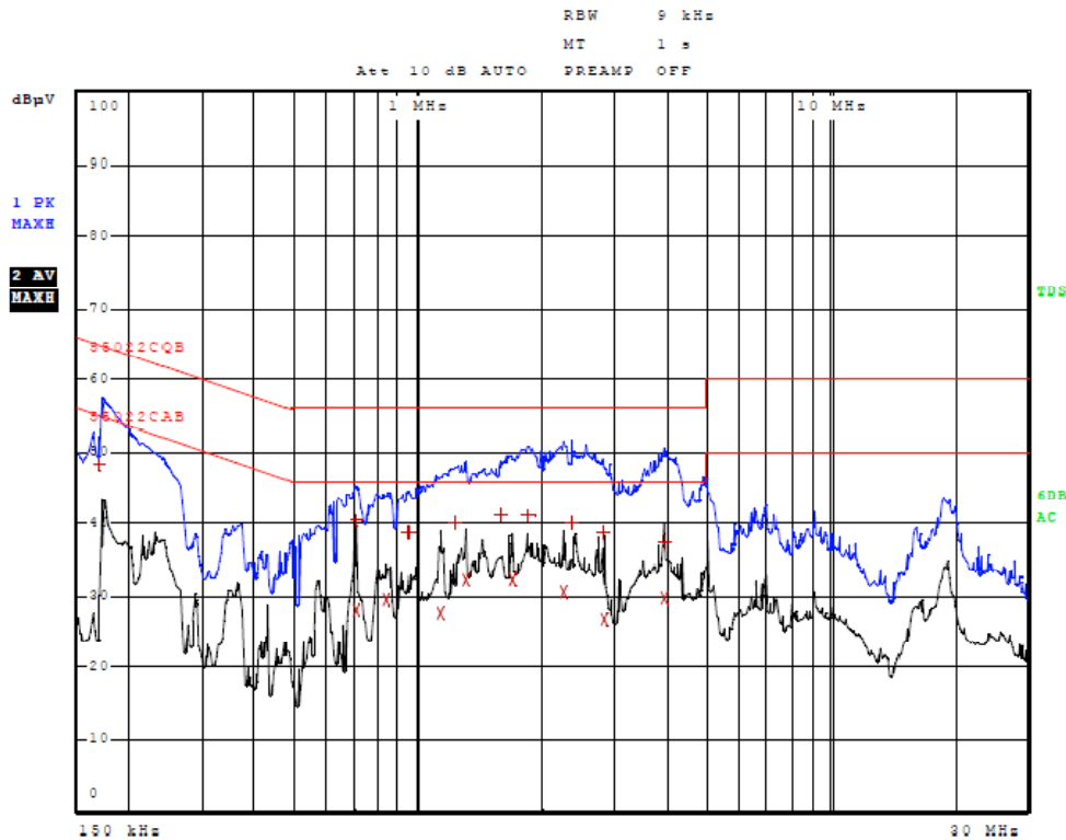
Figure One AC Line Conducted emissions of EUT line 1 (Configuration #2 CPU AC)
