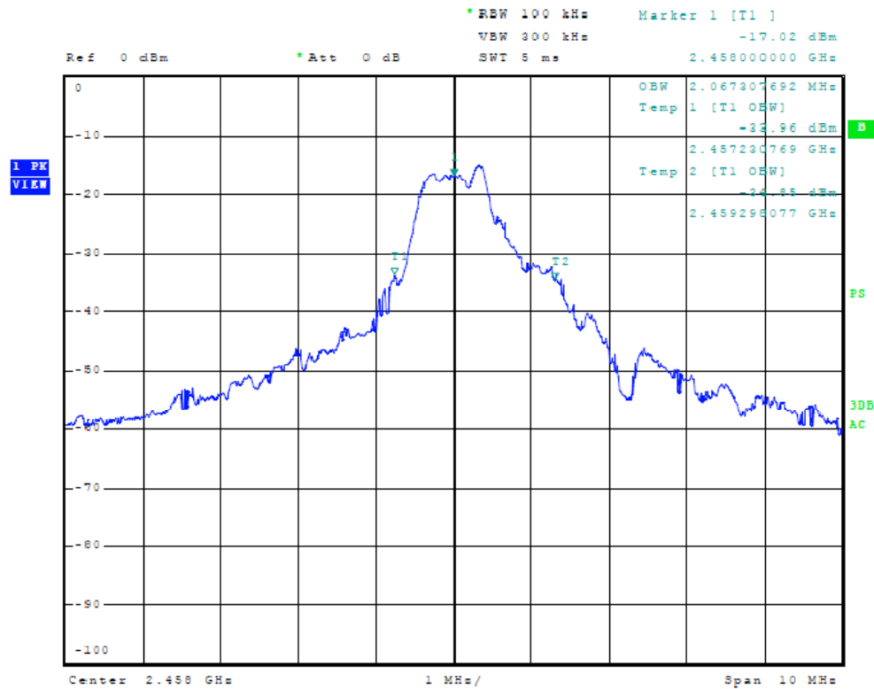
Figure Eleven Plot of 99.5% Occupied Bandwidth (Middle channel)
