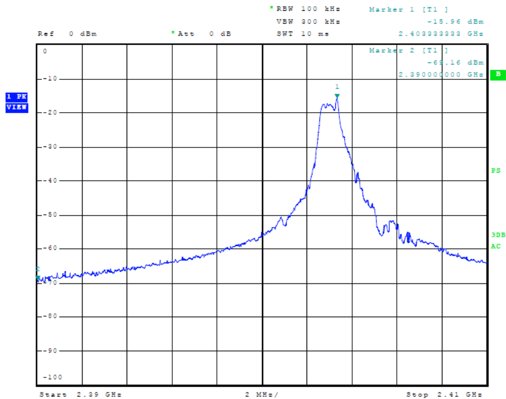
Figure Fourteen of Low Frequency Band Edge
