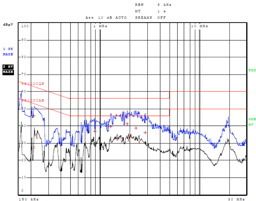
Figure Two AC Line Conducted emissions of EUT line 2 (Configuration #2 CPU AC)
