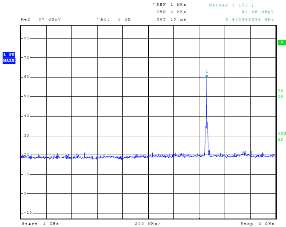
Figure Twelve Radiated Emissions in screen room (DC CLA powered)
