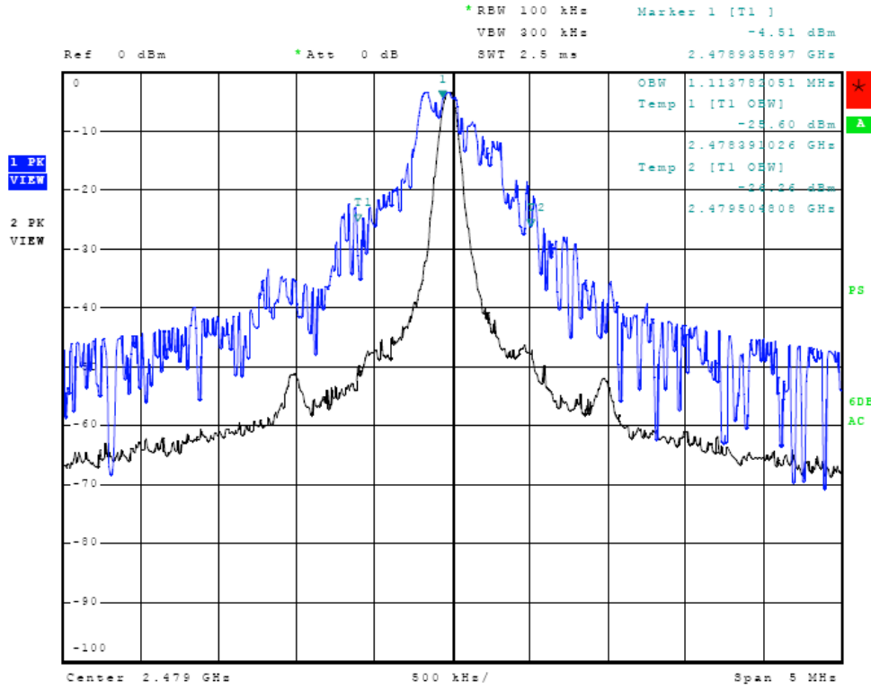
Figure Twenty-seven Occupied Bandwidth (high channel)
