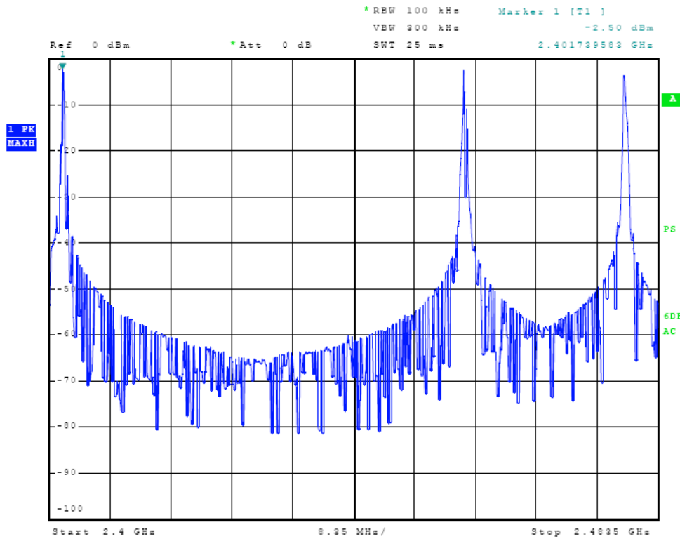
Figure Twenty-eight Operation across frequency band
