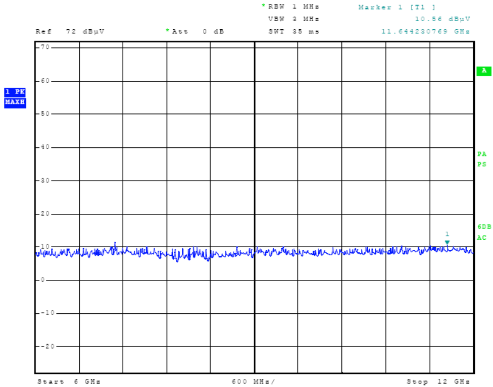
Figure Seven Radiated Emissions in screen room (DC powered)
