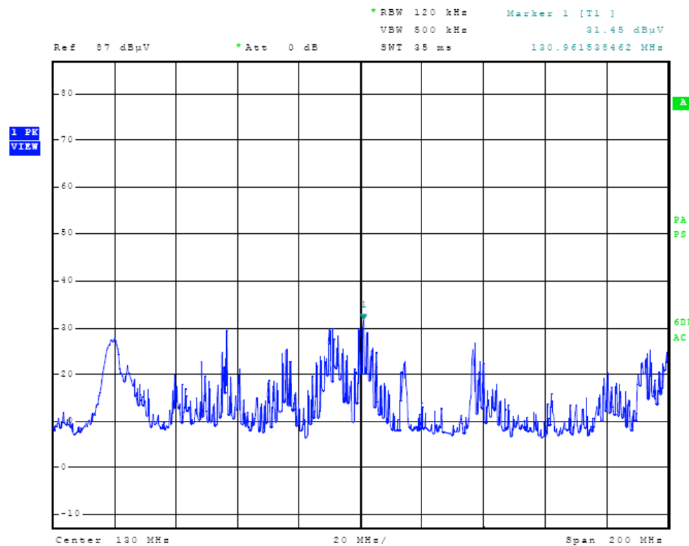
Figure Ten Radiated Emissions in screen room (DC CLA powered)
