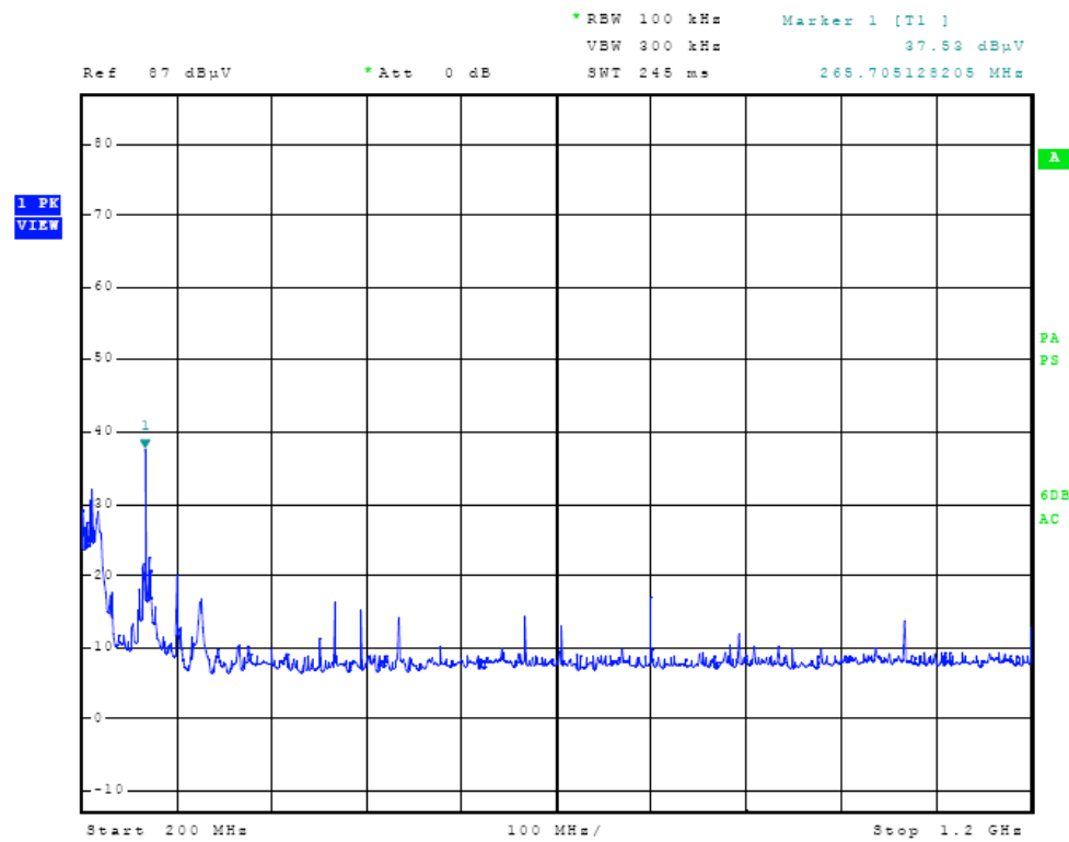
Figure Four Radiated Emissions in screen room (DC powered)
