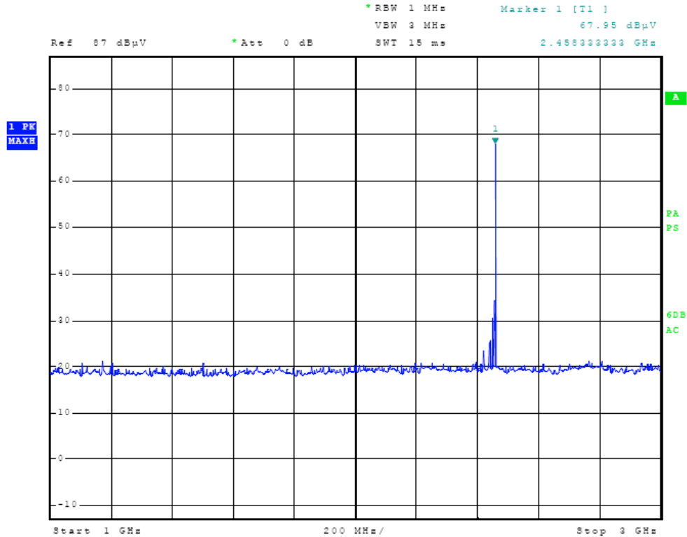
Figure Five Radiated Emissions in screen room (DC powered)
