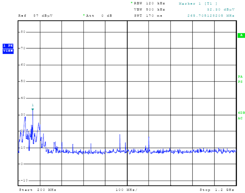
Figure Eleven Radiated Emissions in screen room (DC CLA powered)
