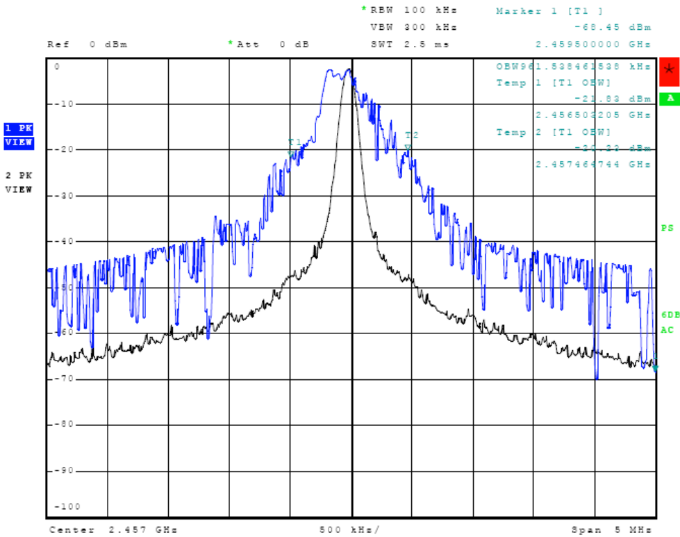
Figure Twenty-six Occupied Bandwidth (middle channel)
