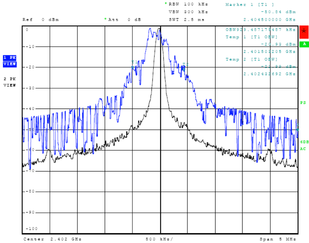
Figure Twenty-five Occupied Bandwidth (low channel)
