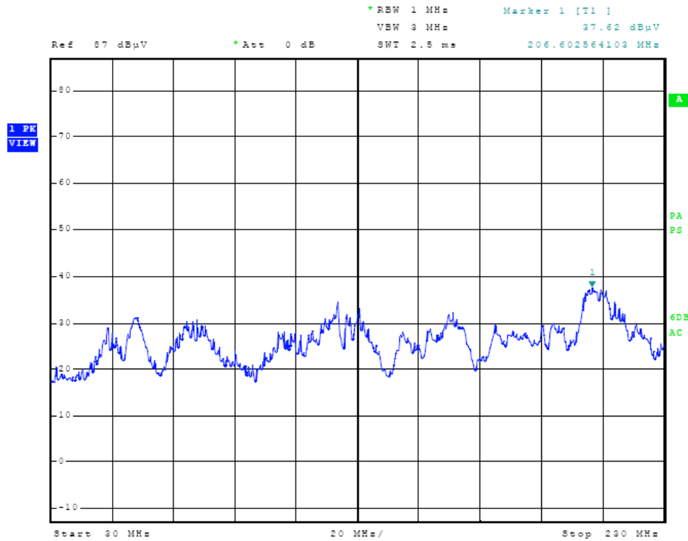
Figure Three Radiated Emissions in screen room (DC powered)
