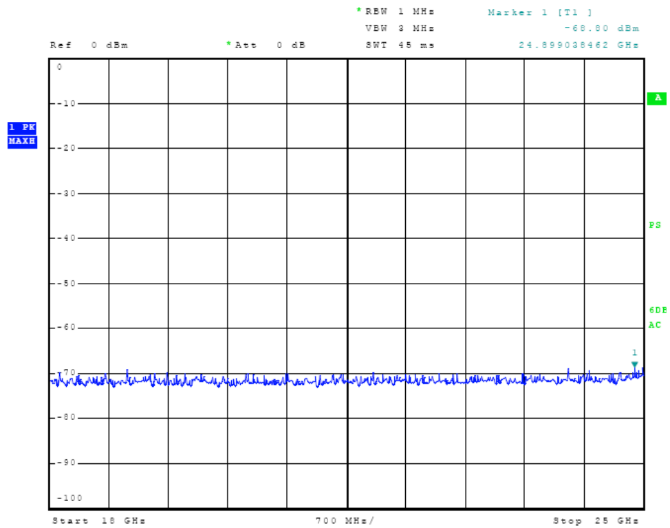
Figure Twenty-four output measured at temporary antenna terminal
