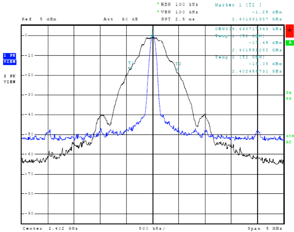
Figure Twenty-three Occupied Bandwidth (low channel)
