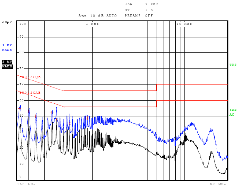
Figure Two AC Line Conducted emissions of EUT line 2 (AC Adapter 362-00072-00)
