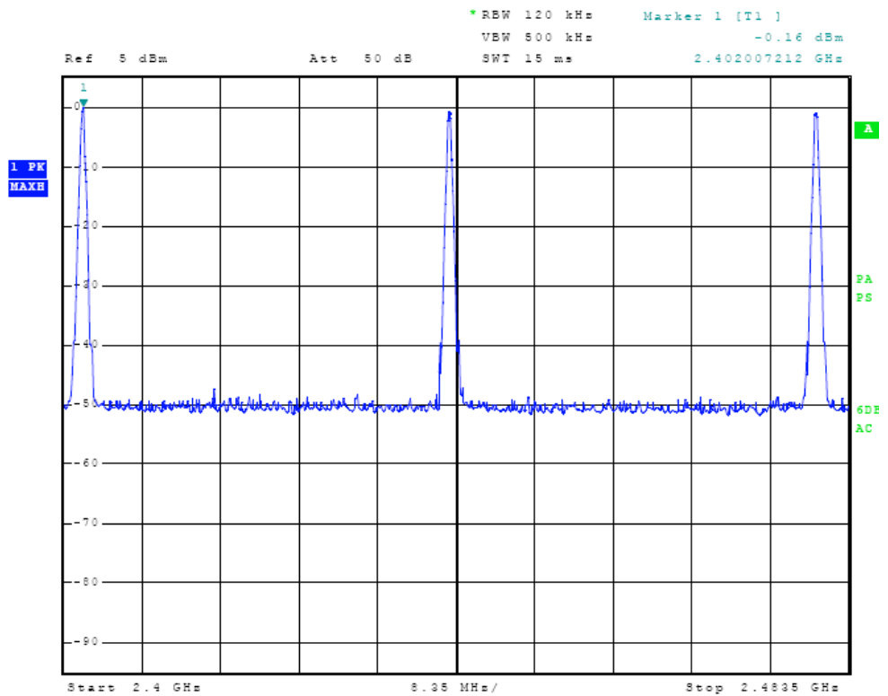
Figure Twenty-six Operation across frequency band
