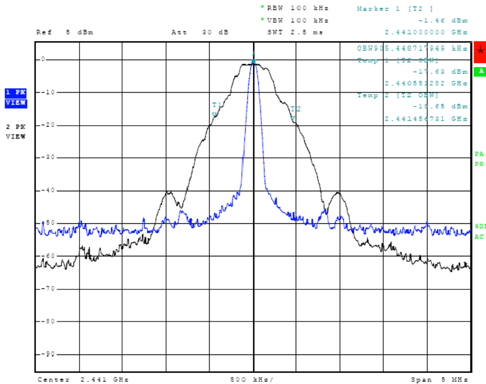
Figure Twenty-four Occupied Bandwidth (middle channel)
