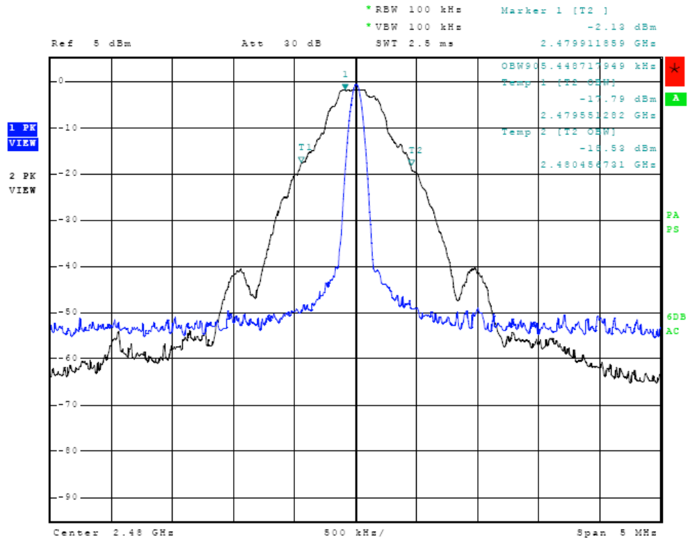
Figure Twenty-five Occupied Bandwidth (high channel)
