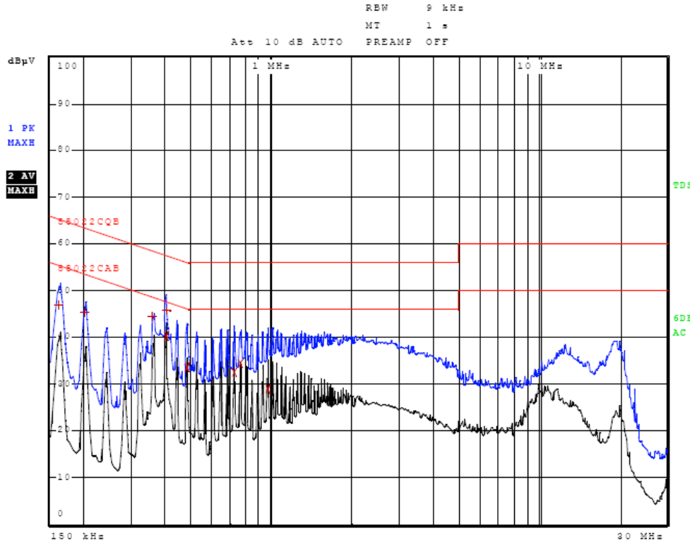
Figure One AC Line Conducted emissions of EUT line 1 (AC Adapter 362-00072-00)
