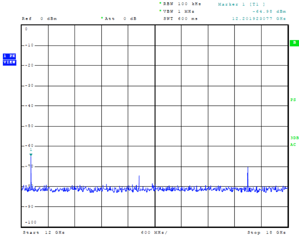
Figure Twenty-Two Plot of Frequency Spectrum at Temporary Antenna Port
