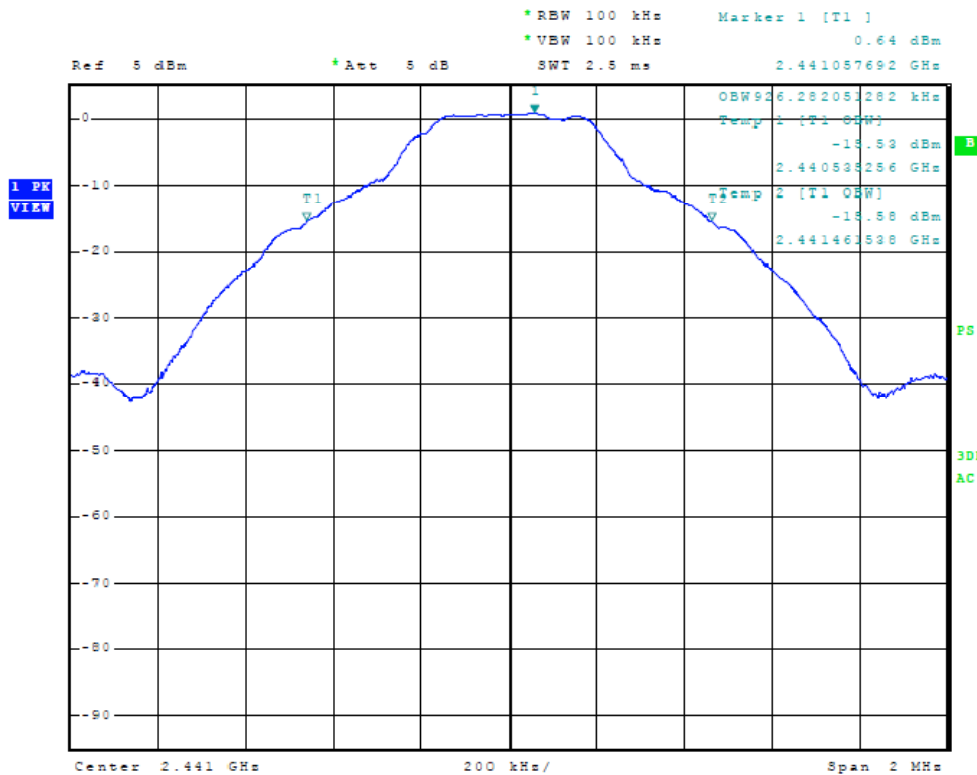
Figure Thirteen Plot of Occupied Bandwidth (Middle channel)
