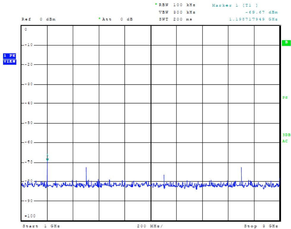
Figure Twenty-Five Receiver Temporary Antenna Port Conducted Emissions
