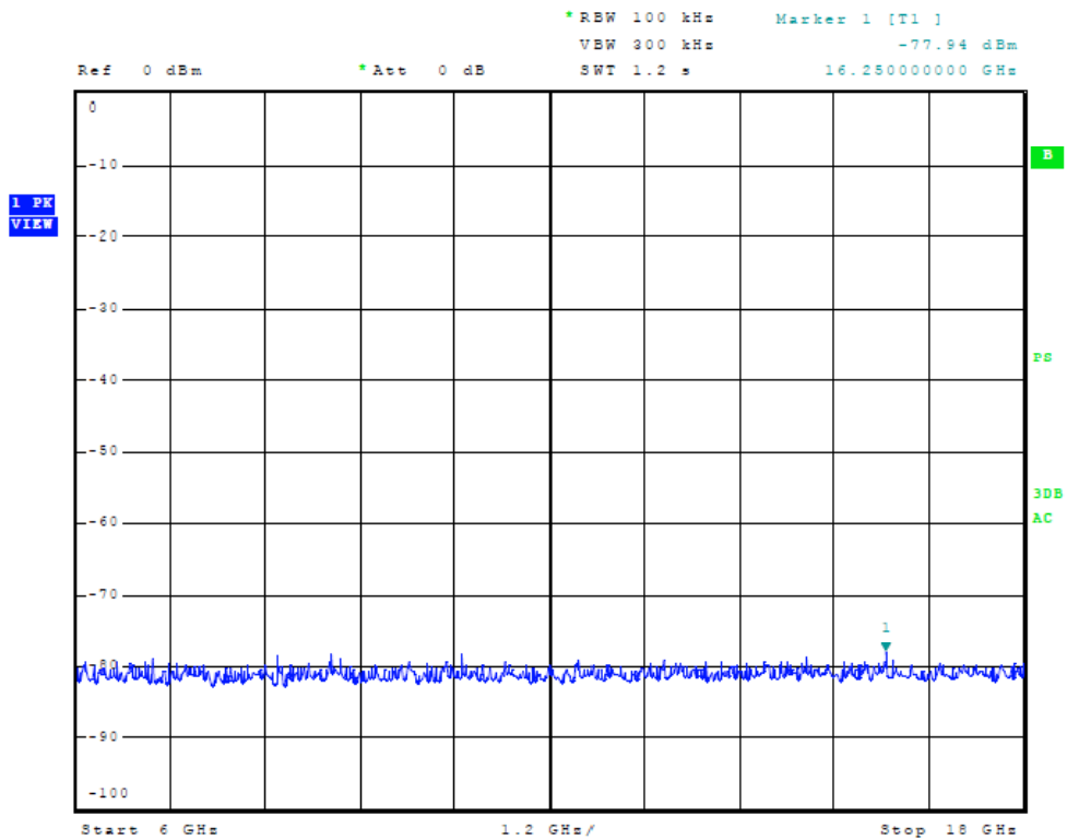
Figure Twenty-Seven Receiver Temporary Antenna Port Conducted Emissions
