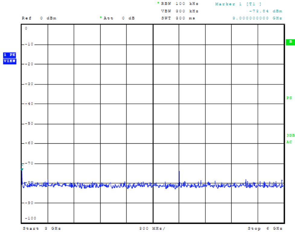
Figure Twenty-Six Receiver Temporary Antenna Port Conducted Emissions
