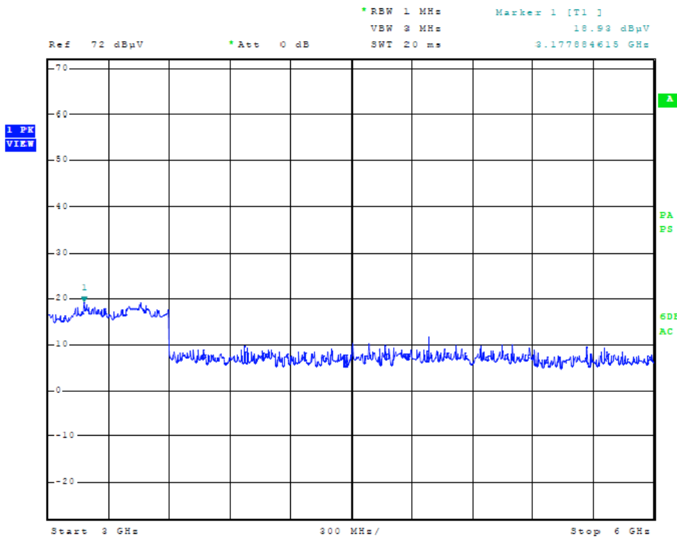
Figure Eight Plot of General Radiated Emissions (EUT CLA)
