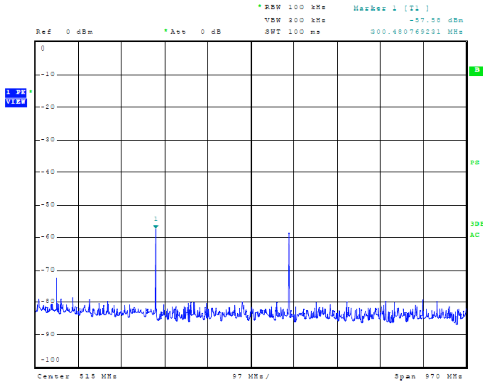
Figure Twenty-Four Receiver Temporary Antenna Port Conducted Emissions
