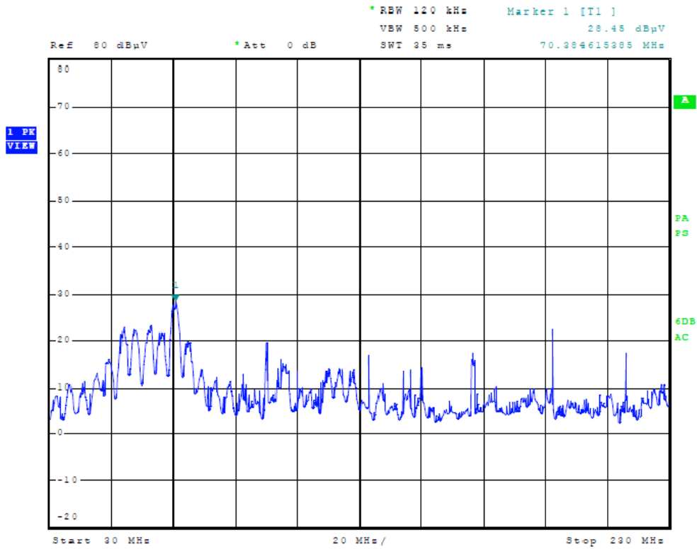
Figure Five Plot of General Radiated Emissions (EUT CLA)
