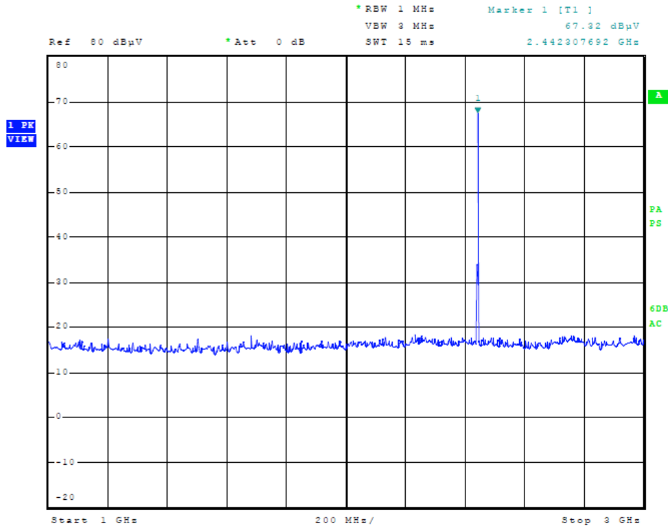
Figure Seven Plot of General Radiated Emissions (EUT CLA)
