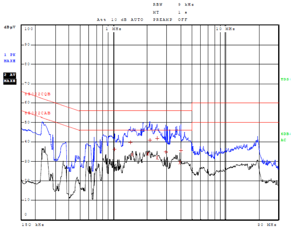
Figure Four AC Line Conducted emissions of EUT line 2 (CPU AC Adapter / USB)
