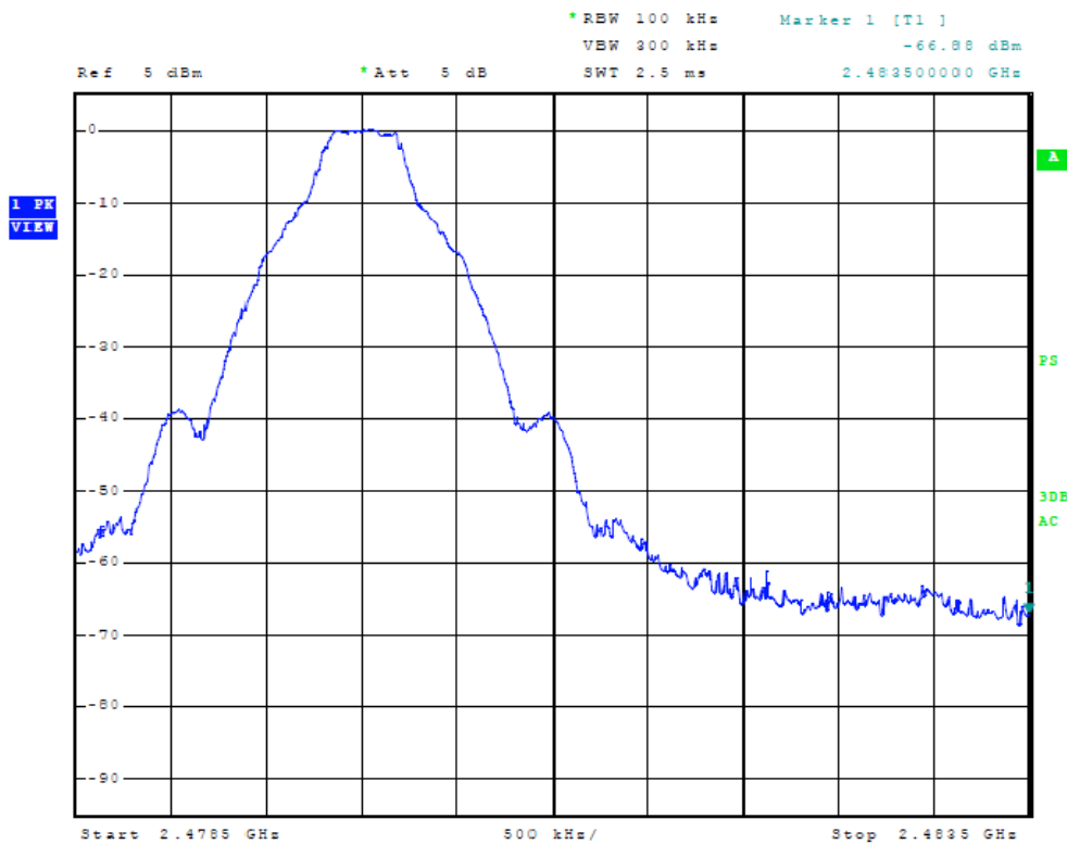
Figure Seventeen Plot of Higher Frequency Band Edge
