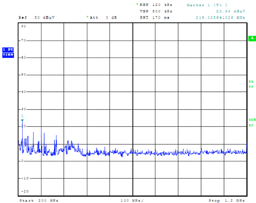
Figure Six Plot of General Radiated Emissions (EUT CLA)
