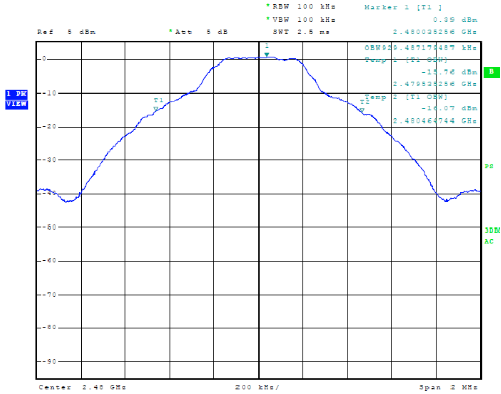
Figure Fourteen Plot of Occupied Bandwidth (High channel)
