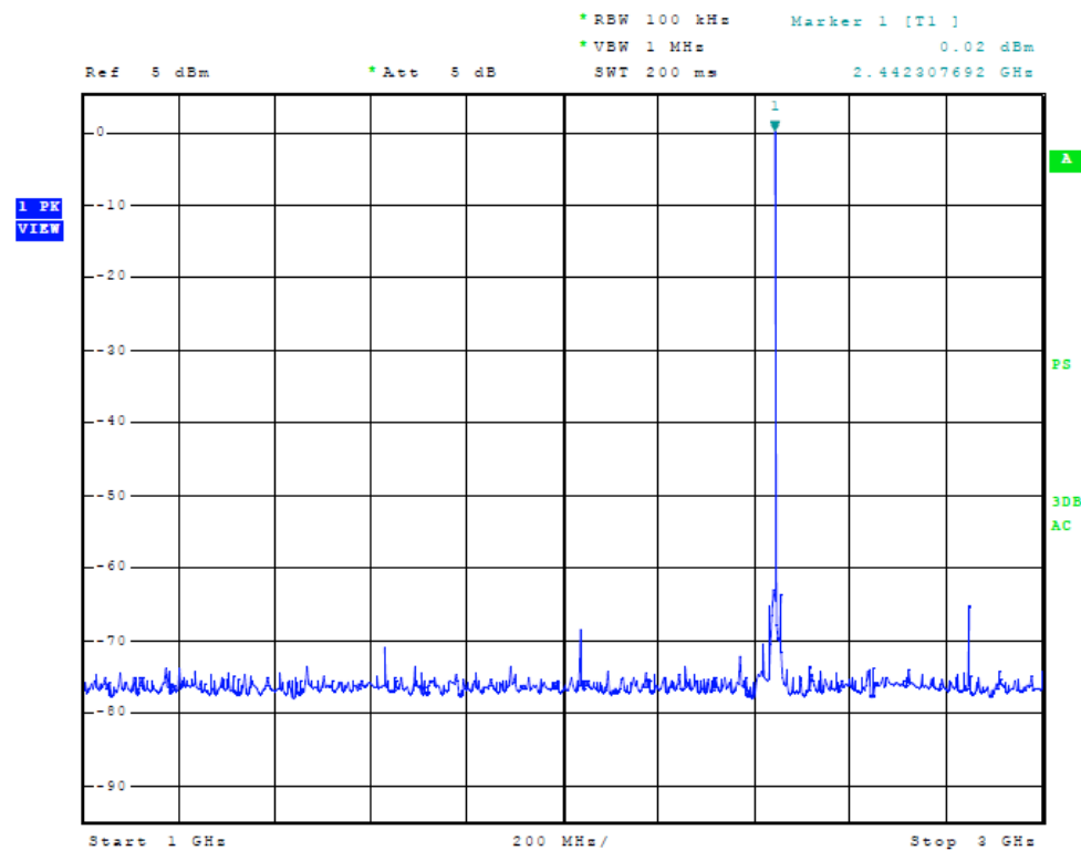
Figure Nineteen Plot of Frequency Spectrum at Temporary Antenna Port
