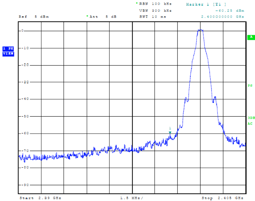
Figure Sixteen Plot of Lower Frequency Band Edge
