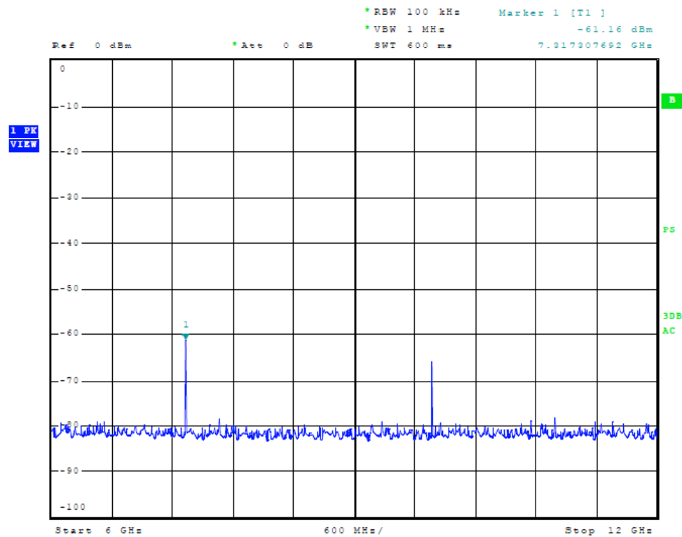
Figure Twenty-One Plot of Frequency Spectrum at Temporary Antenna Port
