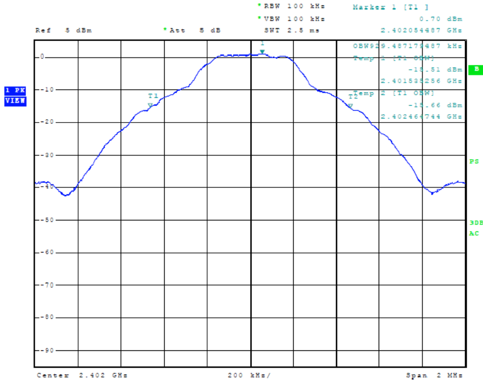
Figure Twelve Plot of Occupied Bandwidth (Low channel)
