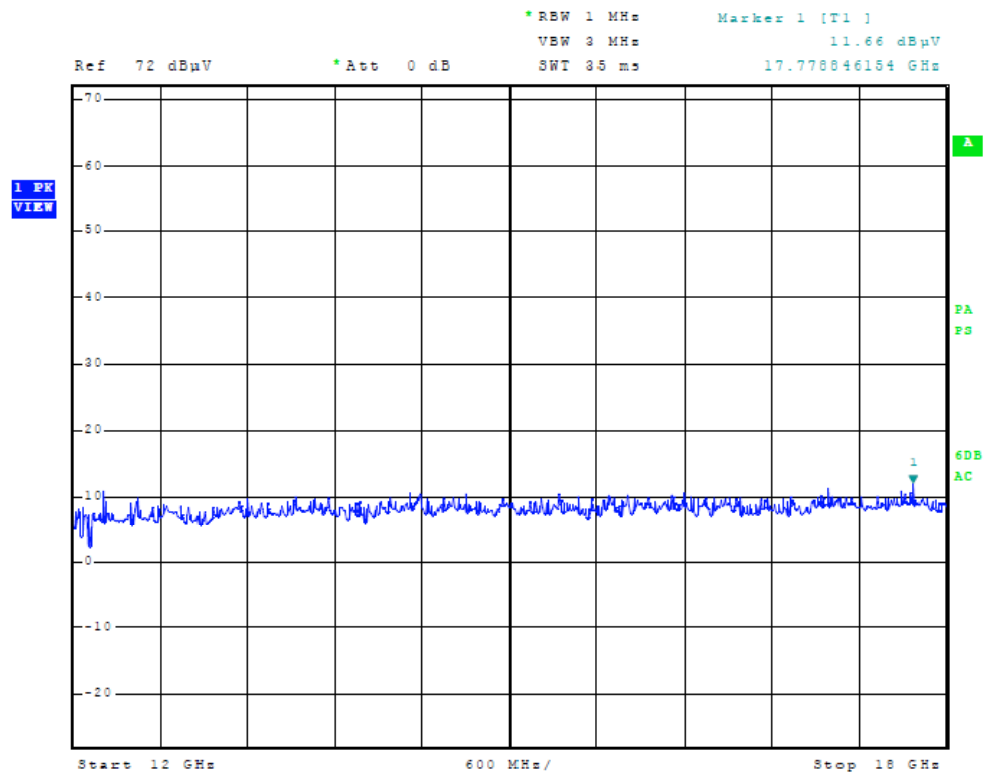
Figure Ten Plot of General Radiated Emissions (EUT CLA)
