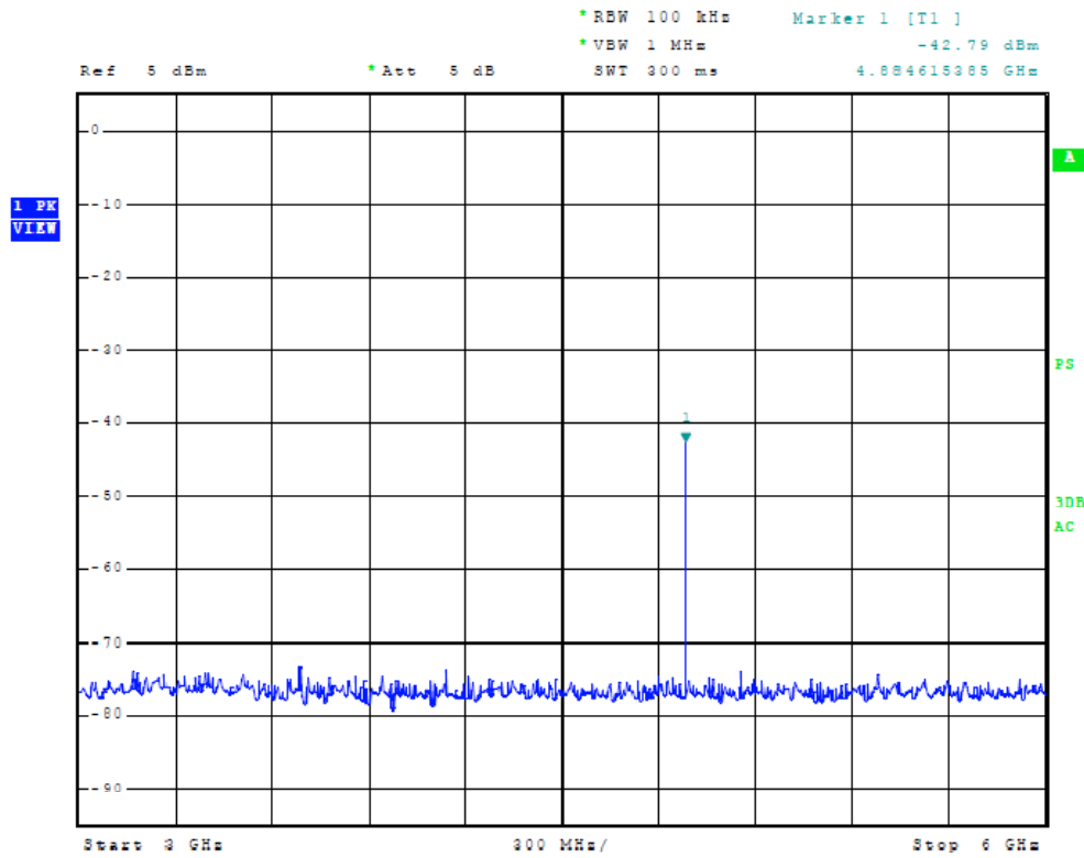
Figure Twenty Plot of Frequency Spectrum at Temporary Antenna Port
