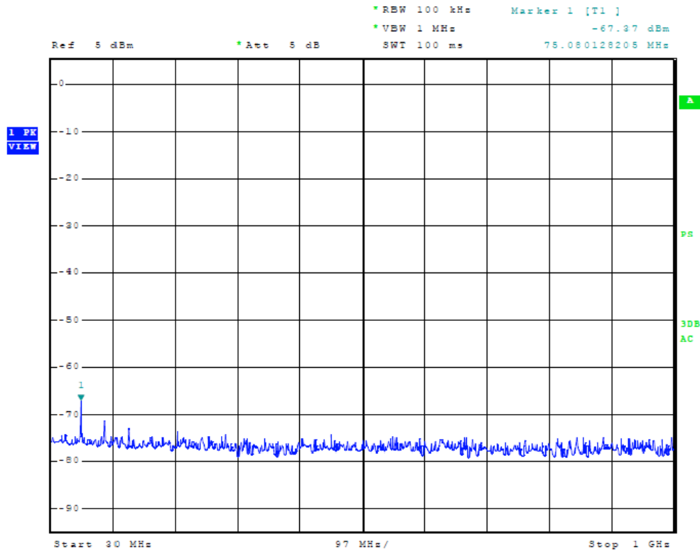
Figure Eighteen Plot of Frequency Spectrum at Temporary Antenna Port
