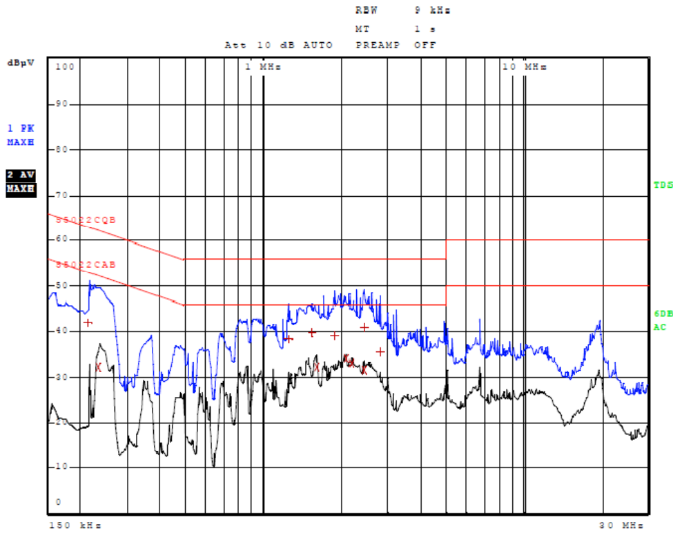
Figure Three AC Line Conducted emissions of EUT line 1 (CPU AC Adapter / USB)
