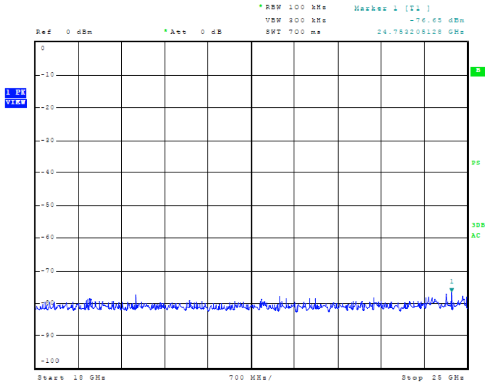
Figure Twenty-Eight Receiver Temporary Antenna Port Conducted Emissions
