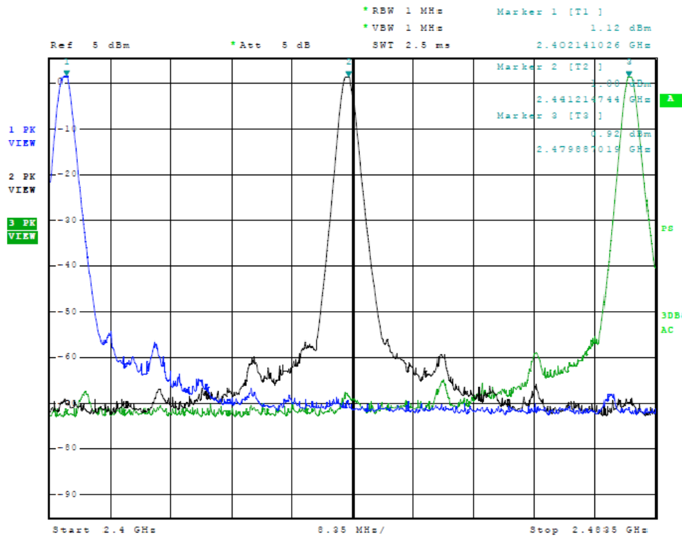
Figure Fifteen Plot of Operation across frequency band
