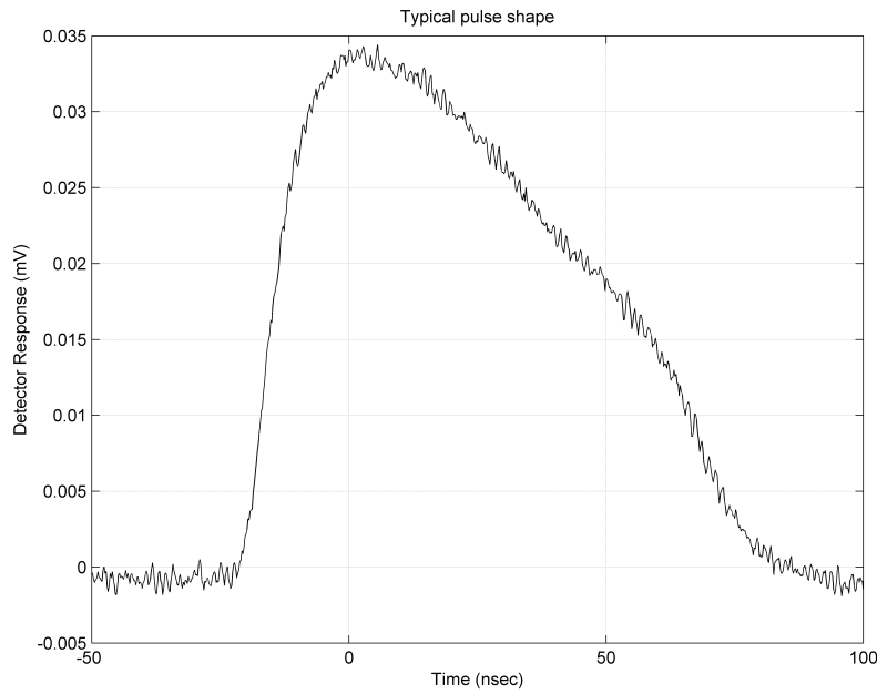
Figure 2. Typical pulse from EUT using wideband detector.
