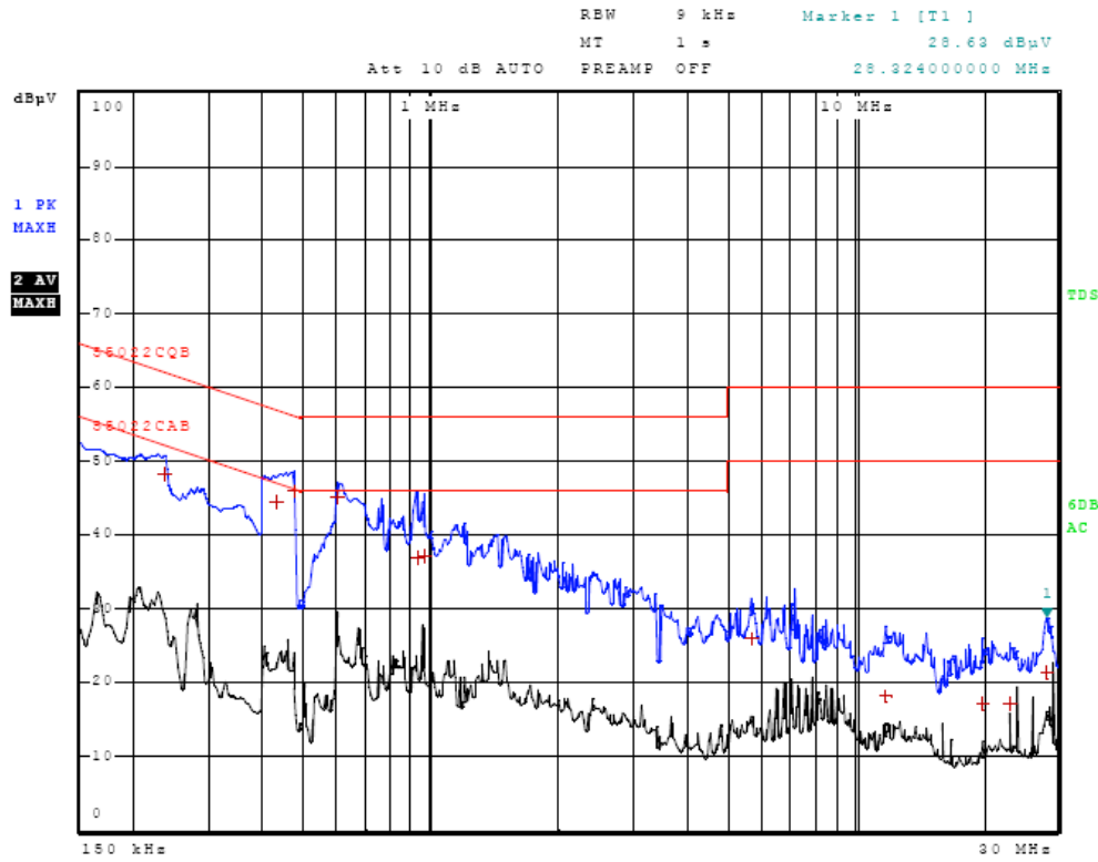
Figure One AC Line Conducted emissions of EUT line 1 (Configuration #1)
