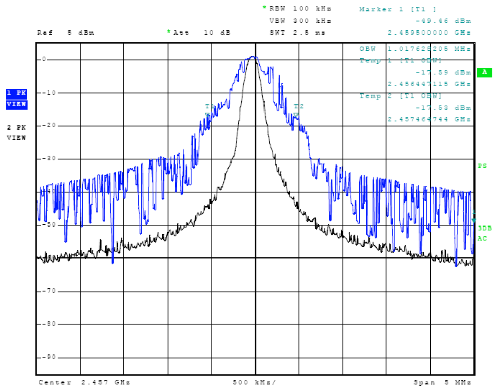
Figure Twenty-one Occupied Bandwidth measured at temporary antenna terminal
