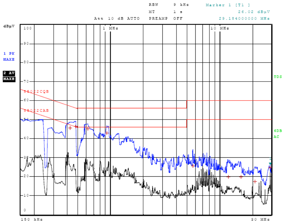
Figure Two AC Line Conducted emissions of EUT line 2 (Configuration #1)
