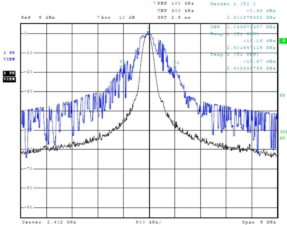
Figure Twenty Occupied Bandwidth measured at temporary antenna terminal
