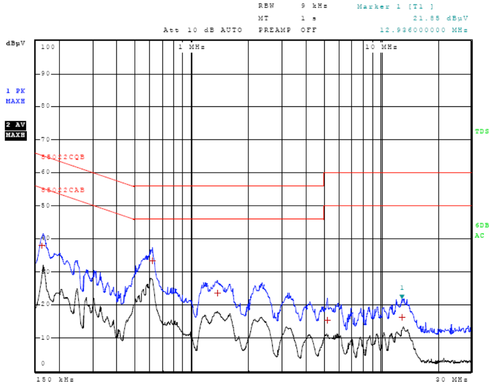
Figure Three AC Line Conducted emissions of EUT line 1 (Configuration #2)
