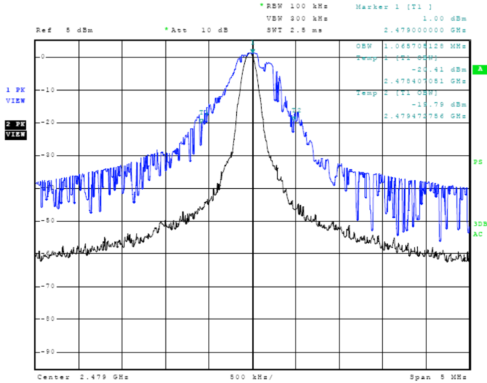
Figure Twenty-two Occupied Bandwidth measured at temporary antenna terminal
