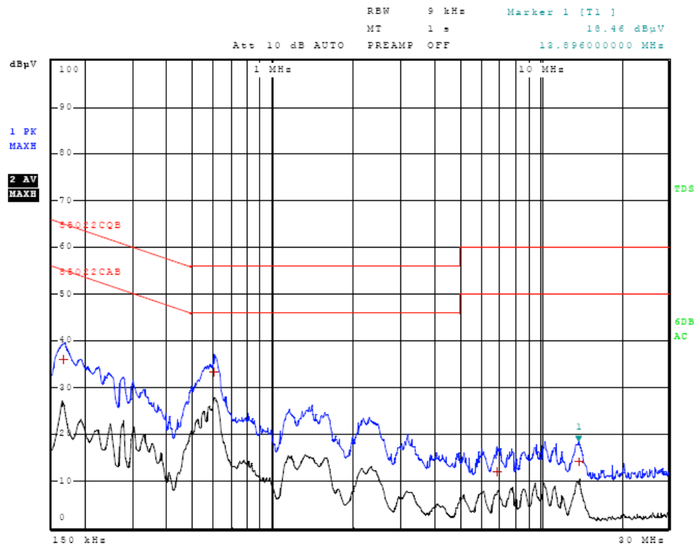
Figure Four AC Line Conducted emissions of EUT line 2 (Configuration #2)
