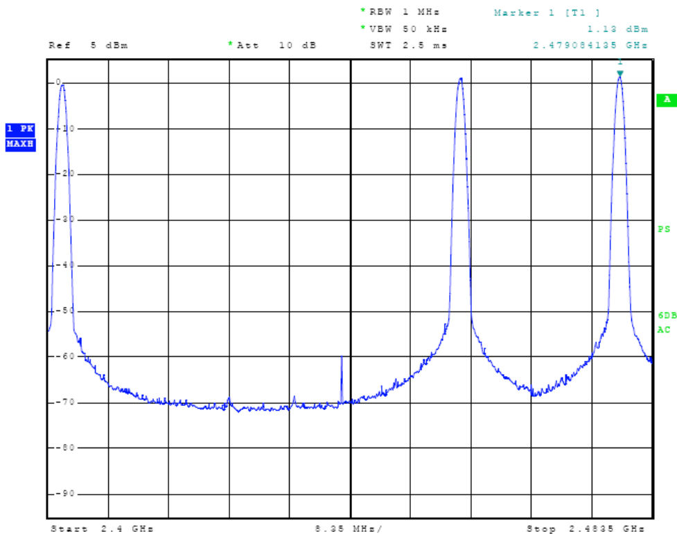
Figure Nineteen Output power across band measured at temporary antenna terminal
