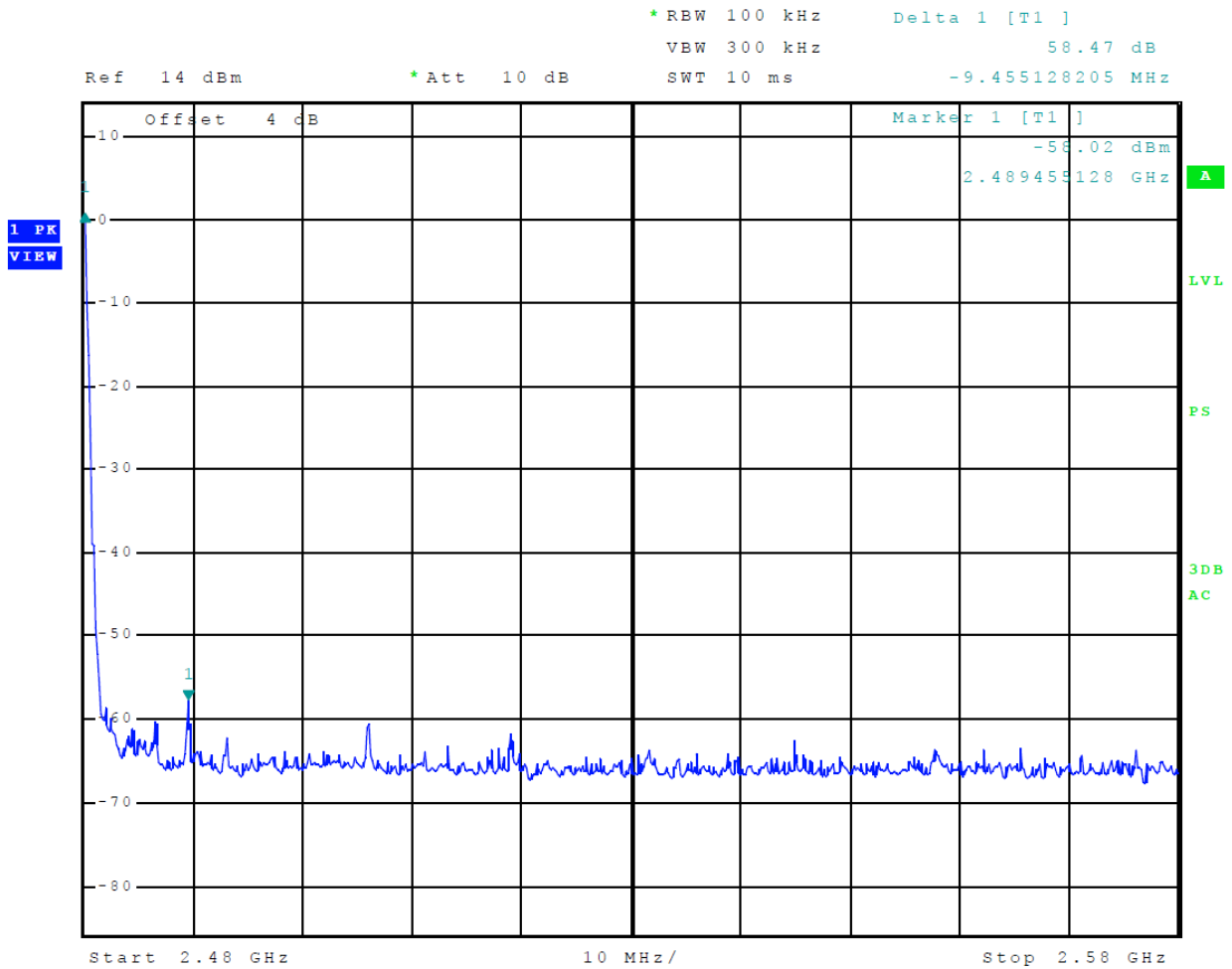
Figure 13 Plot of Transmitter Emissions High Band Edge Mode 1 (GFSK)
