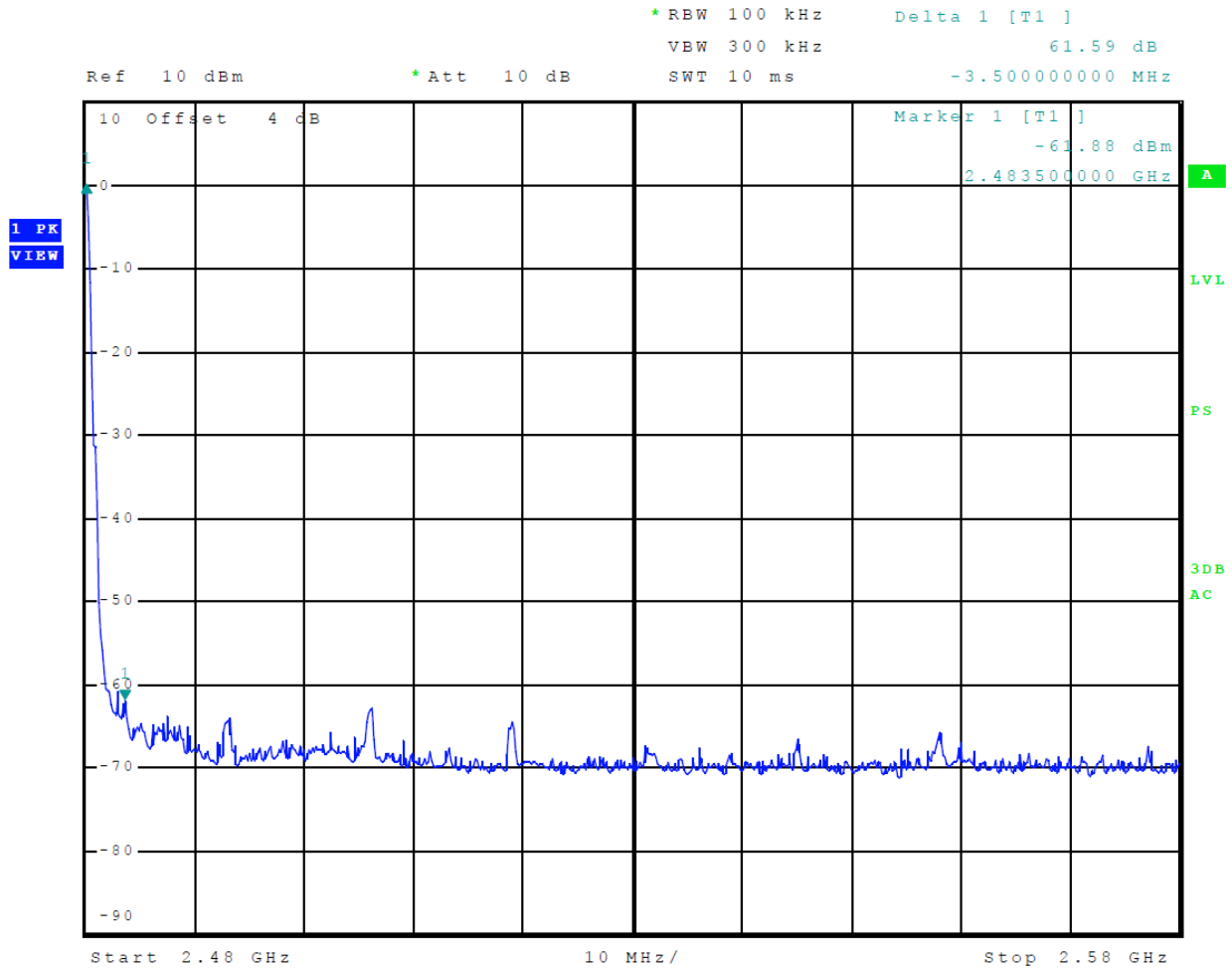
Figure 16 Plot of Transmitter Emissions High Band Edge Mode 4 (GMSK)
