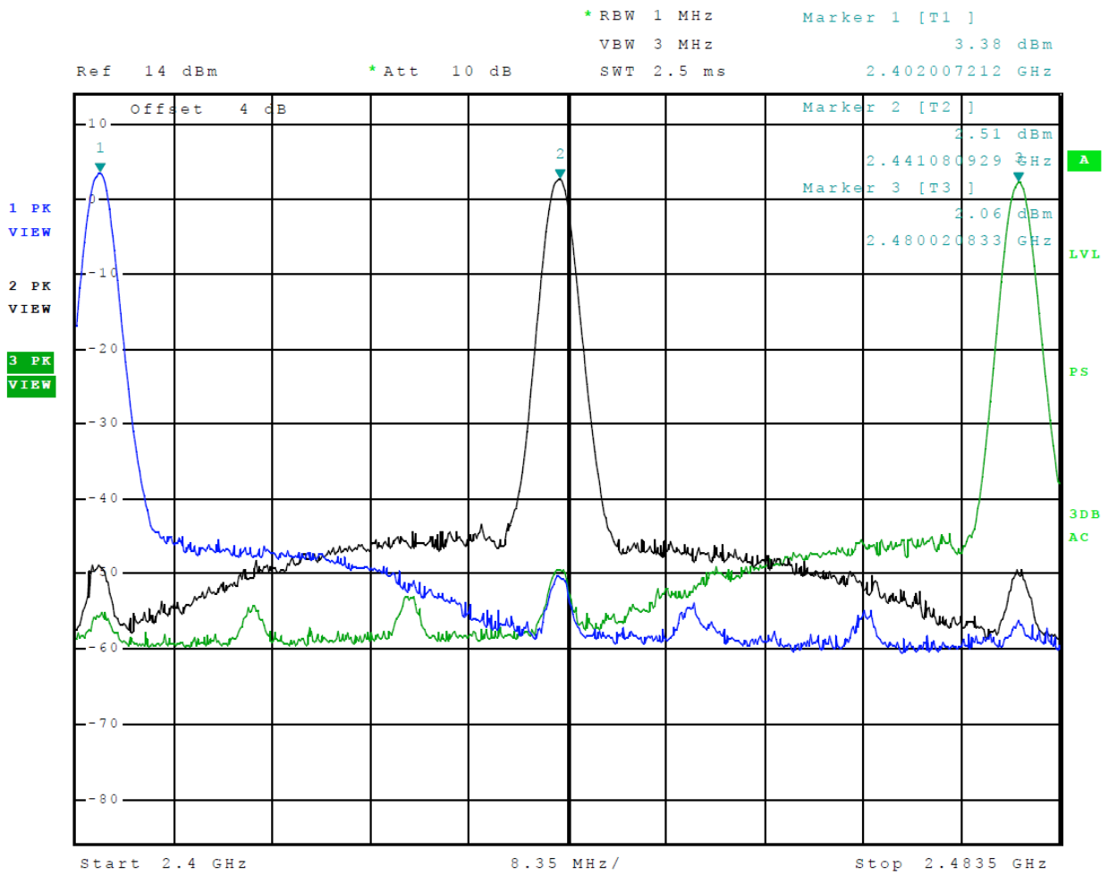
Figure 3 Plot of Transmitter Emissions Operation in 2402-2480 MHz Mode 3 (8-DPSK)
