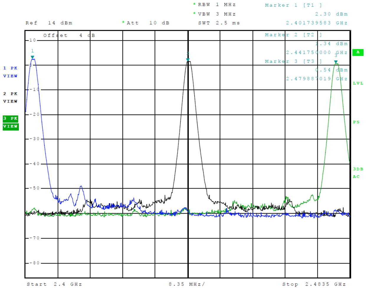
Figure 4 Plot of Transmitter Emissions Operation in 2402-2480 MHz Mode 4 (GMSK)
