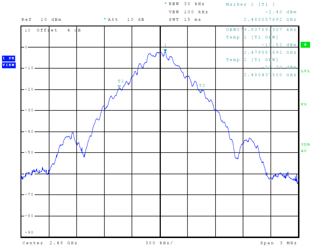
Figure 5 Plot of Transmitter Emissions 99% Occupied Bandwidth Mode 1 (GFSK)
