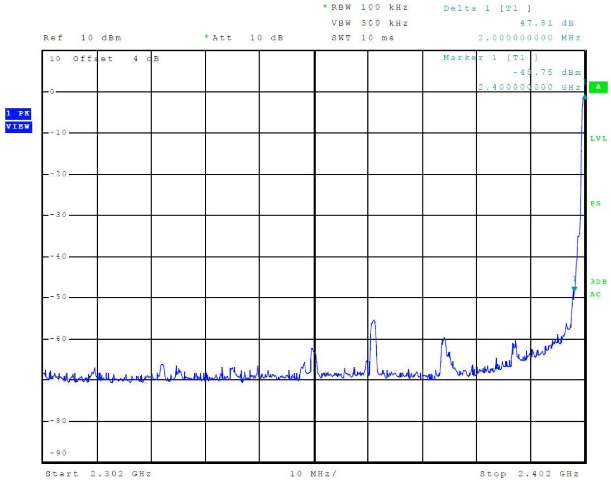
Figure 10 Plot of Transmitter Emissions Low Band Edge Mode 2 ( \pi/4 -DQPSK)
