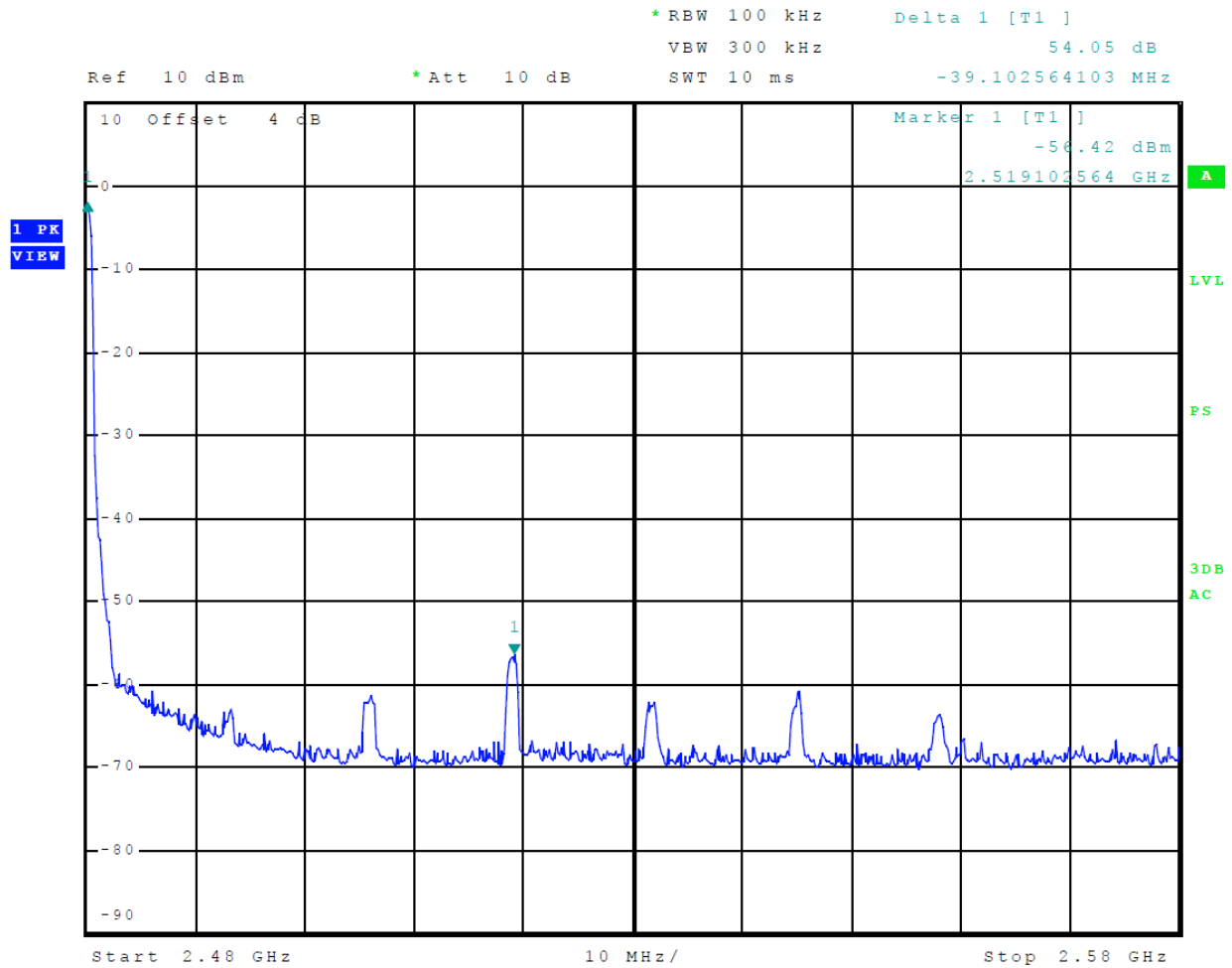
Figure 14 Plot of Transmitter Emissions High Band Edge Mode 2 ( \pi/4 -DQPSK)
