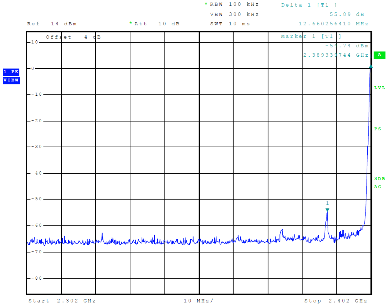
Figure 12 Plot of Transmitter Emissions Low Band Edge Mode 4 (GMSK)
