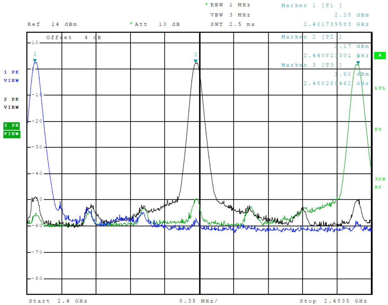
Figure 2 Plot of Transmitter Emissions Operation in 2402-2480 MHz Mode 2 ( \pi/4 -DQPSK)
