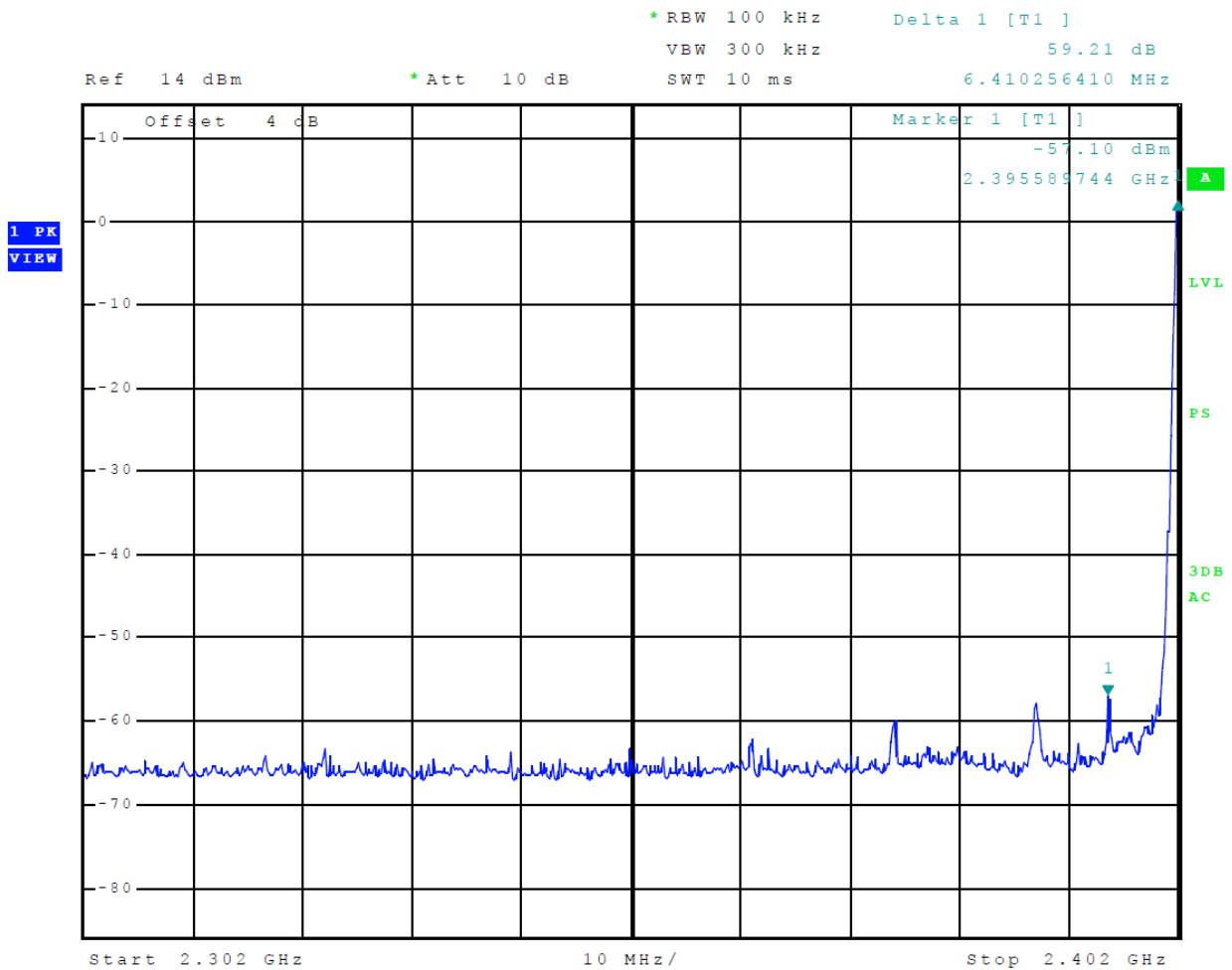
Figure 9 Plot of Transmitter Emissions Low Band Edge Mode 1 (GFSK)
