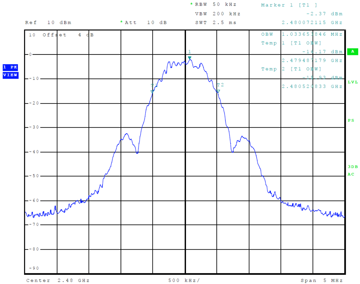
Figure 8 Plot of Transmitter Emissions 99% Occupied Bandwidth Mode 4 (GMSK)
