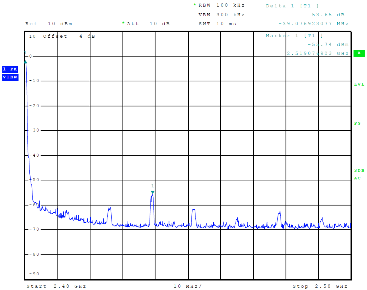
Figure 15 Plot of Transmitter Emissions High Band Edge Mode 3 (8-DPSK)
