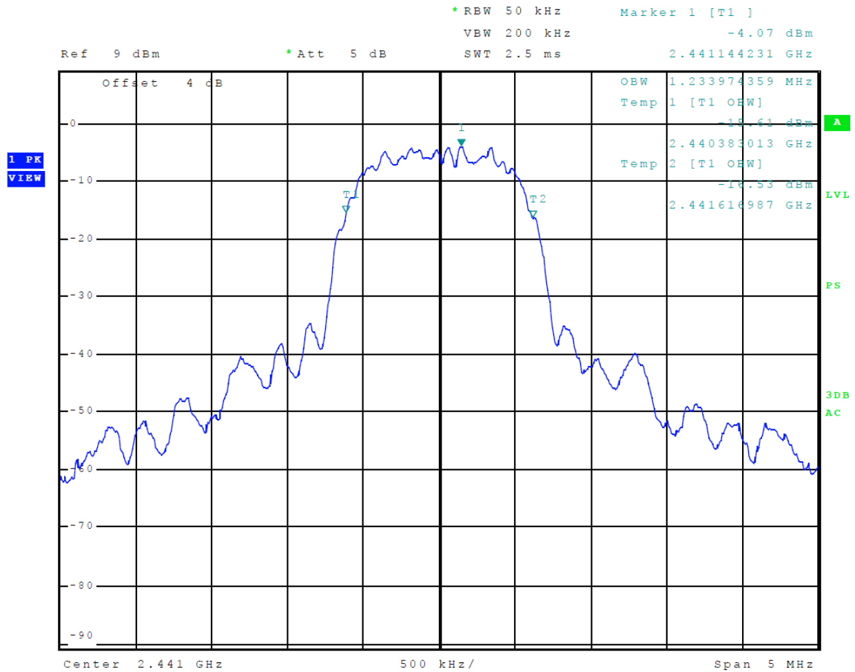
Figure 6 Plot of Transmitter Emissions 99% Occupied Bandwidth Mode 2 ( \pi/4 -DQPSK)
