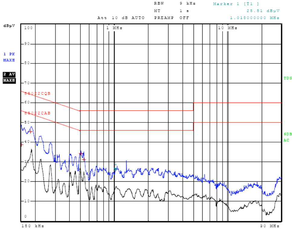
Figure Three AC Line Conducted emissions of EUT line 1 (Configuration #2, 362-00043-04)
