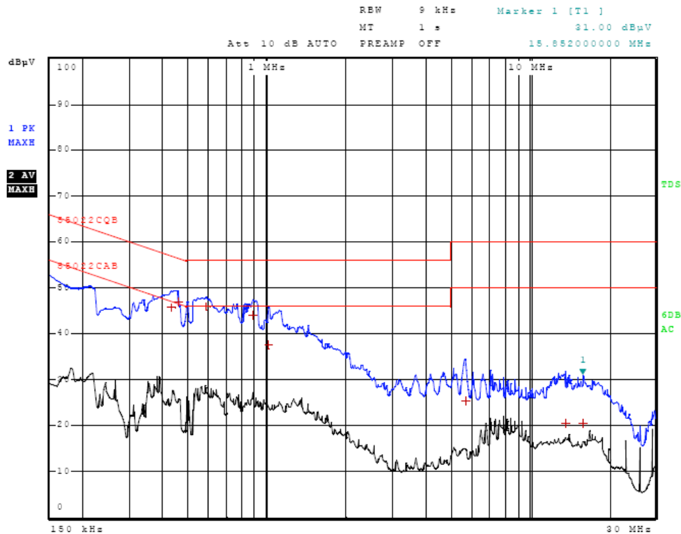
Figure Six AC Line Conducted emissions of EUT line 2 (Configuration #3)
