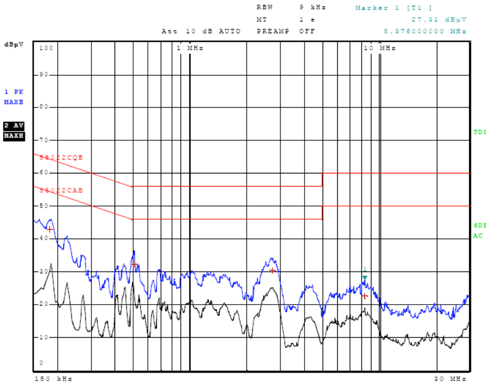
Figure Four AC Line Conducted emissions of EUT line 2 (Configuration #2, 362-00043-04)
