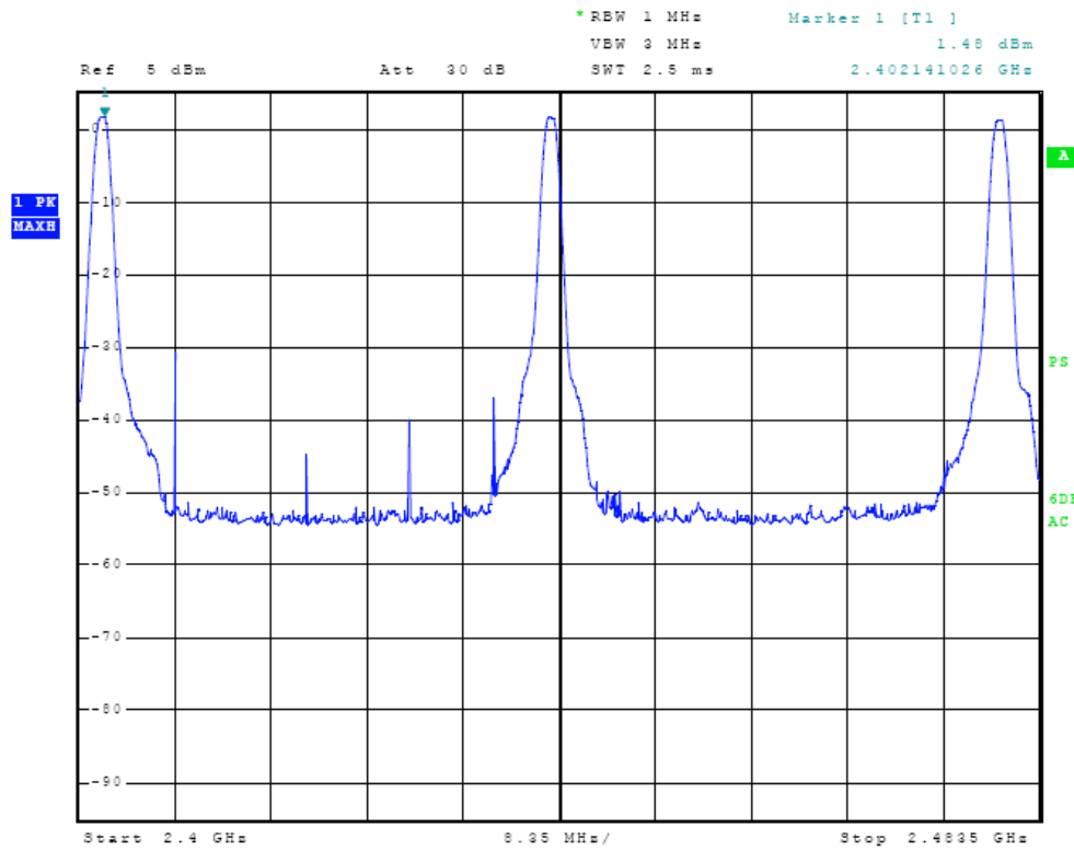
Figure Twenty-two Output power across band
