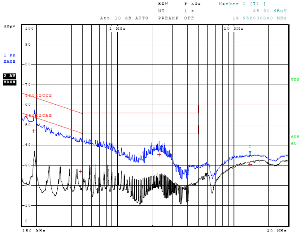
Figure One AC Line Conducted emissions of EUT line 1 (Configuration #2, 362-00042-00)
