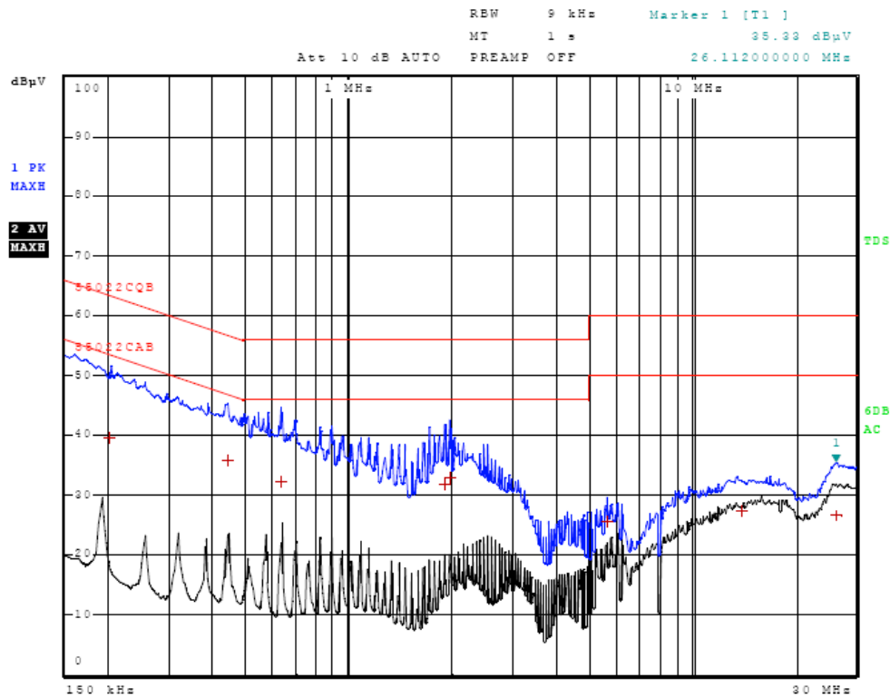
Figure Two AC Line Conducted emissions of EUT line 2 (Configuration #2, 362-00042-00)
