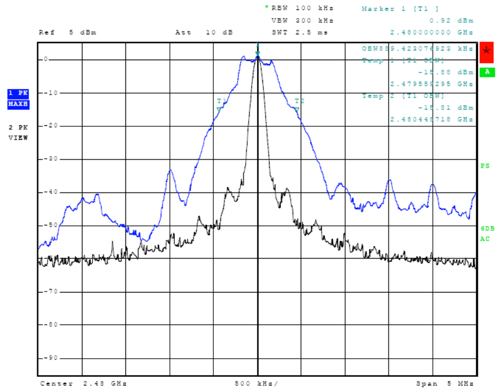
Figure Twenty-five Occupied Bandwidth
