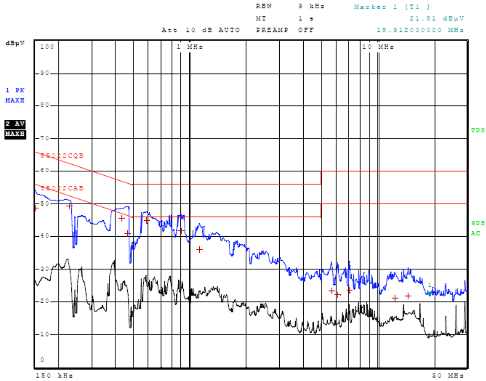
Figure Five AC Line Conducted emissions of EUT line 1 (Configuration #3)
