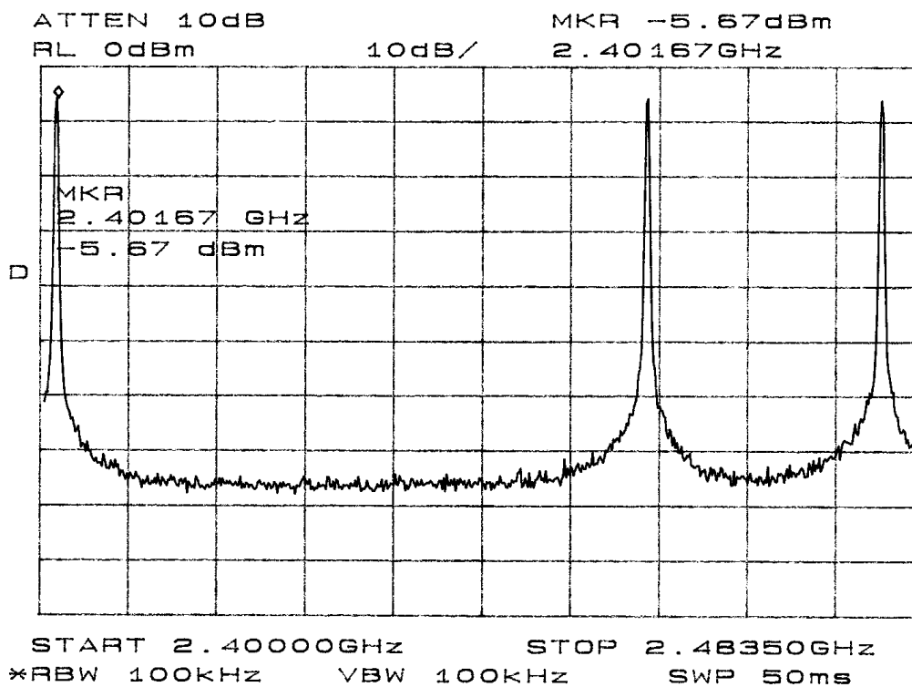
Figure Thirteen output measured at temporary antenna terminal
