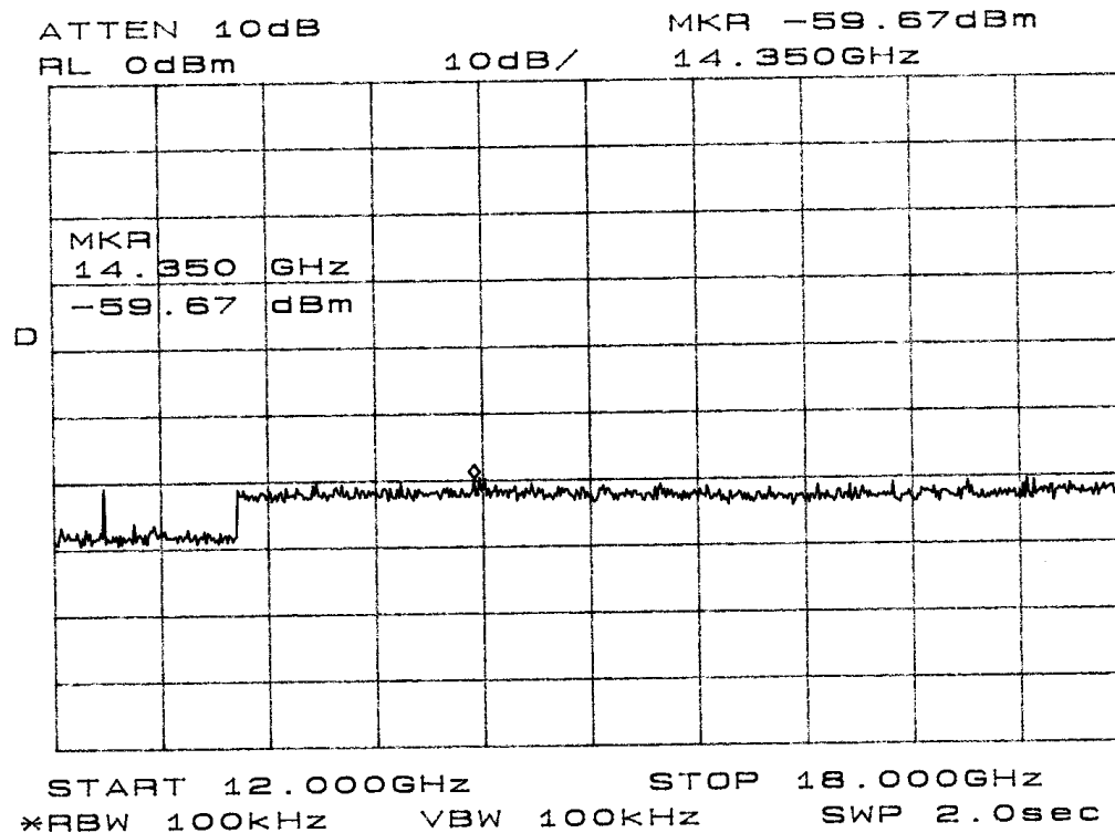
Figure Twelve output measured at temporary antenna terminal
