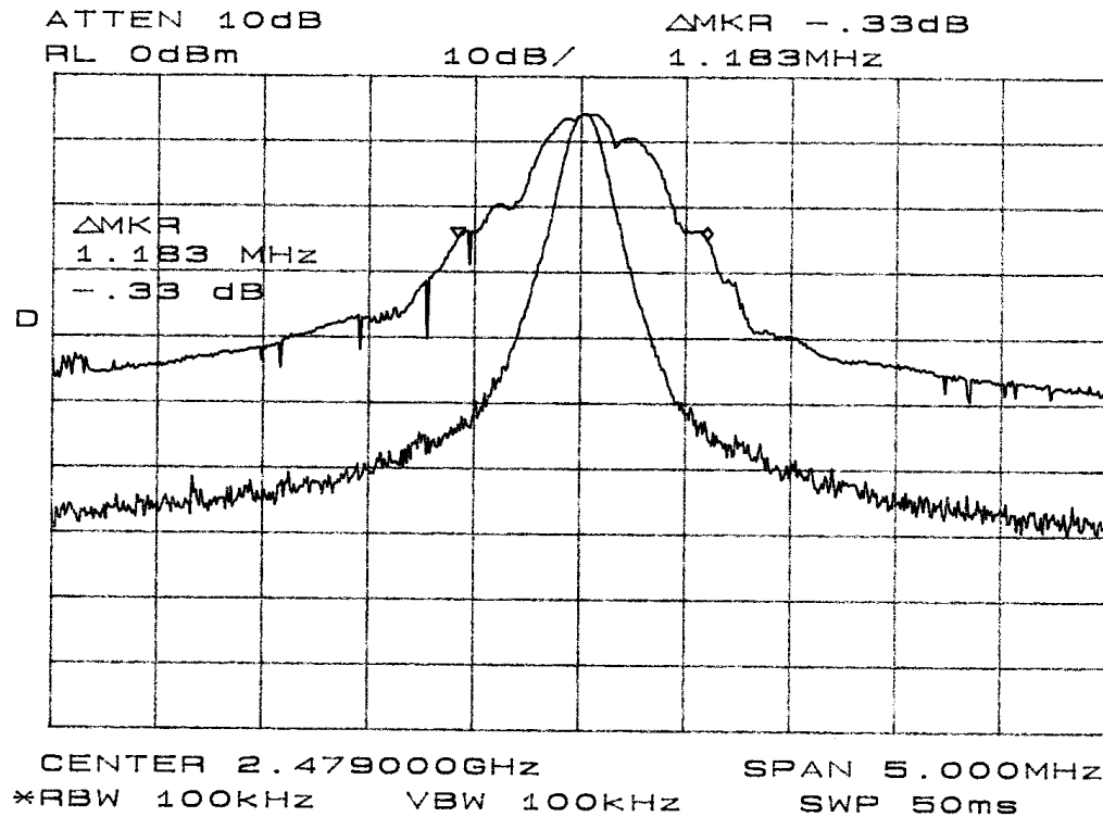
Figure Sixteen Occupied Bandwidth
