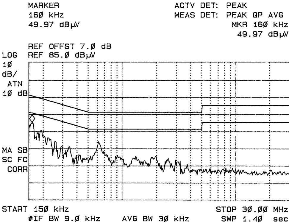
Figure two Conducted emissions of EUT line 2
