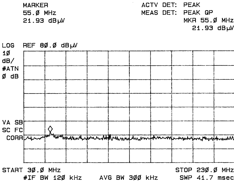
Figure three Radiated Emissions Plot
