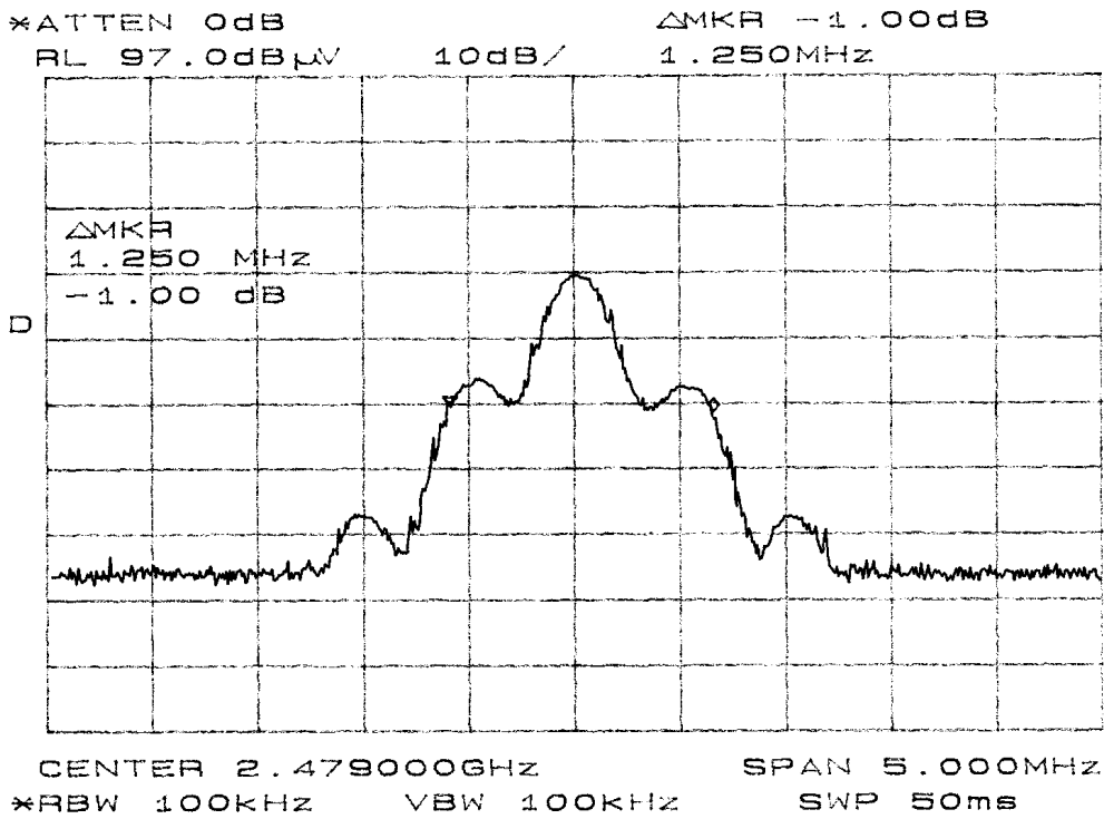
Figure thirteen Occupied Bandwidth
