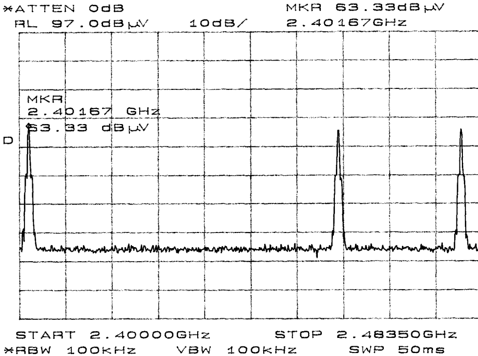
Figure ten Operation in Frequency Band
