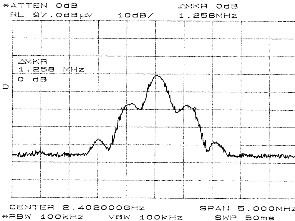
Figure eleven Occupied Bandwidth
