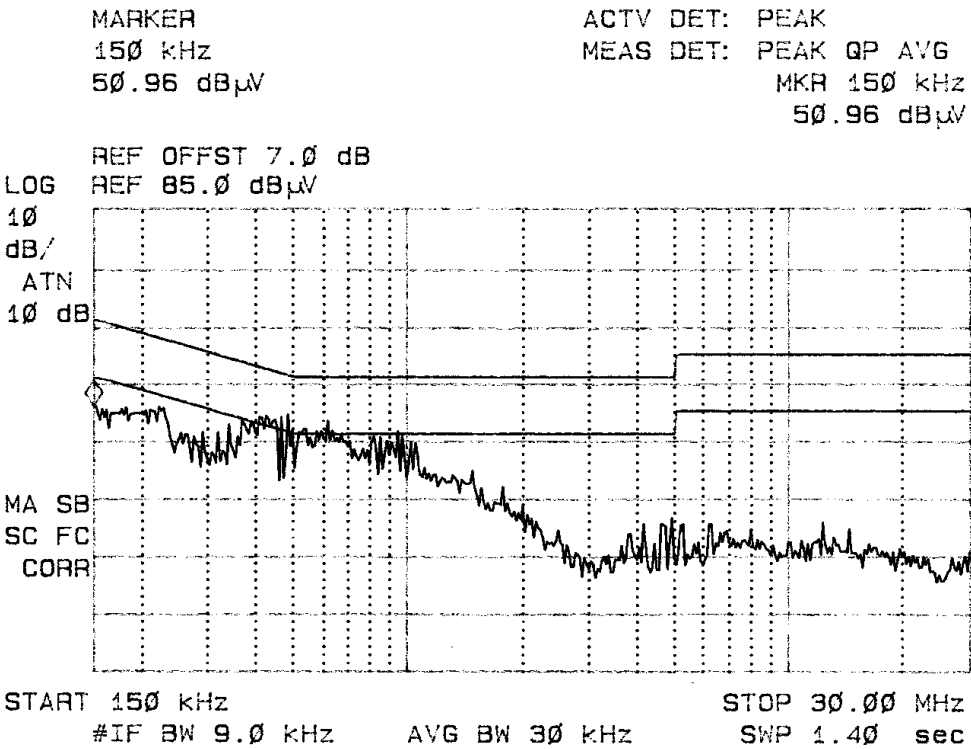
Figure Four AC Line Conducted emissions of EUT line 2 (CPU)
