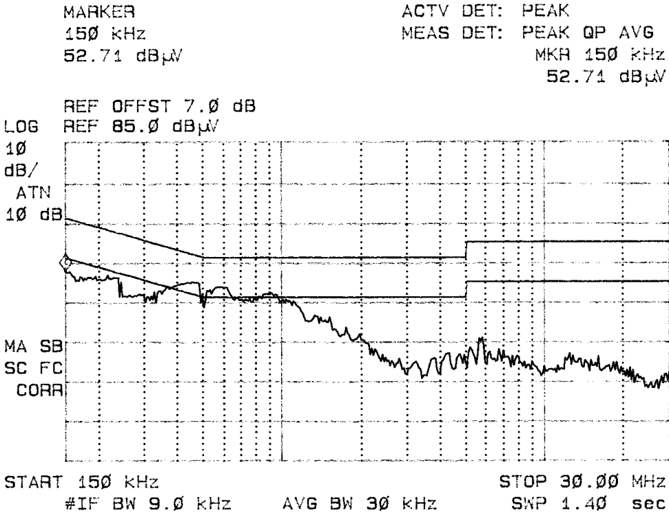
Figure Three AC Line Conducted emissions of EUT line 1 (CPU)
