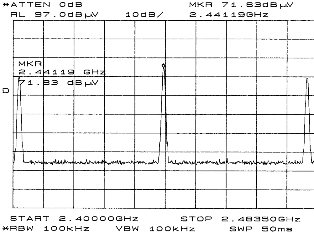
Figure twelve Output Across Operational Band
