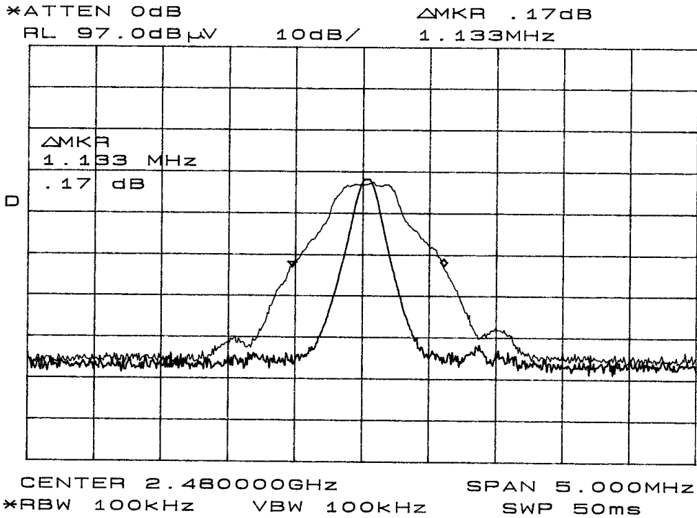
Figure fifteen Occupied Bandwidth
