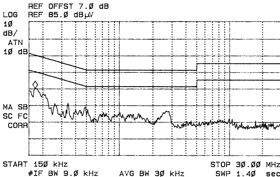
Figure Two AC Line Conducted emissions of EUT line 2 (362-00043-04)
