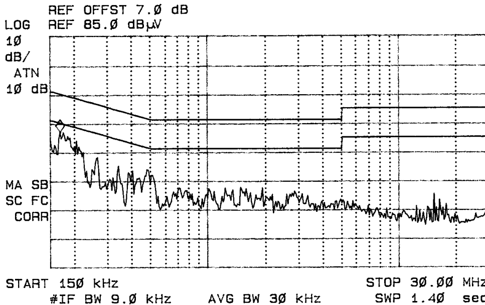
Figure One AC Line Conducted emissions of EUT line 1 (362-00043-04)
