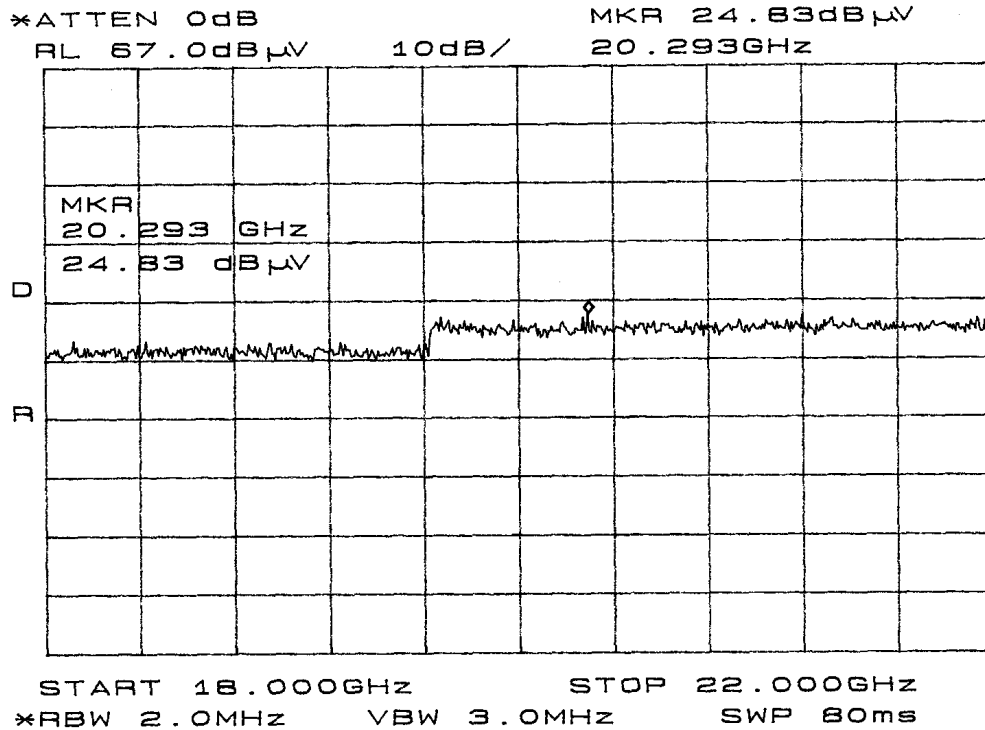
Figure seven Radiated Emissions Plot
