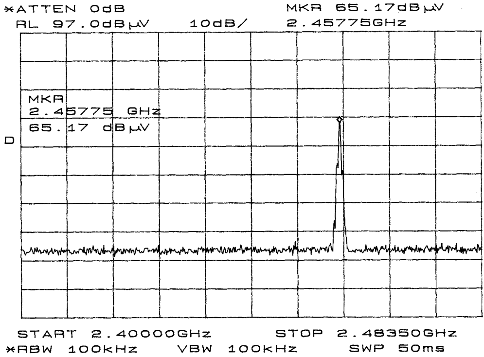
Figure eight Operation in Frequency Band
