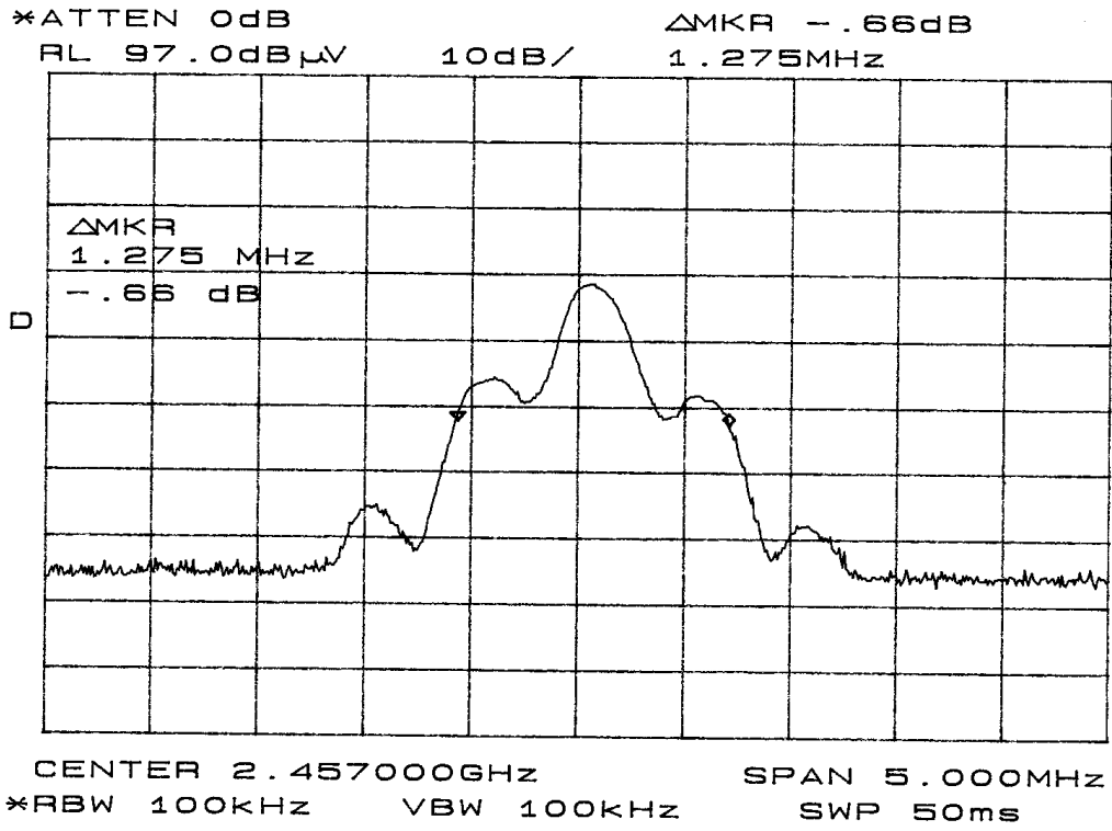
Figure nine Occupied Bandwidth
