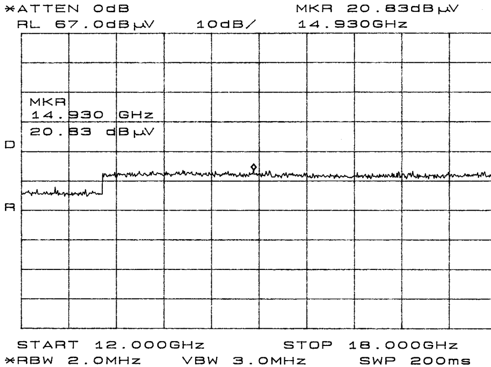
Figure six Radiated Emissions Plot
