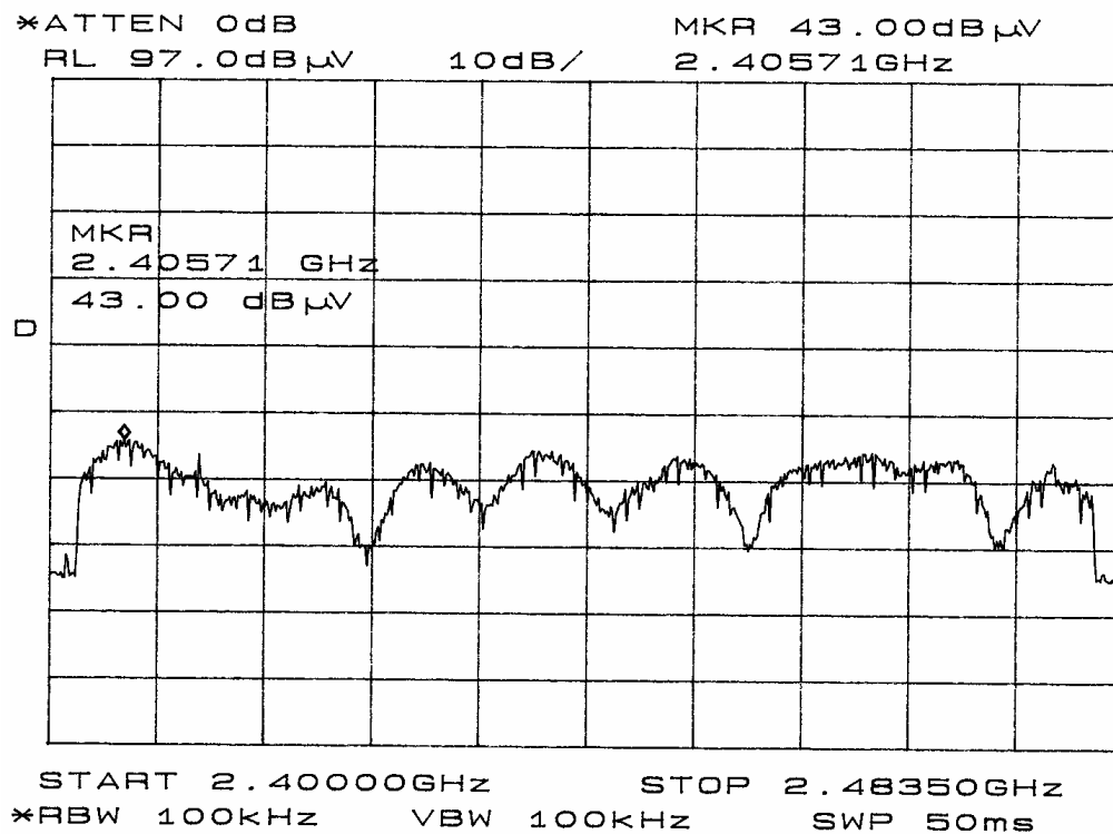
Figure Ten Operation across Frequency Band
