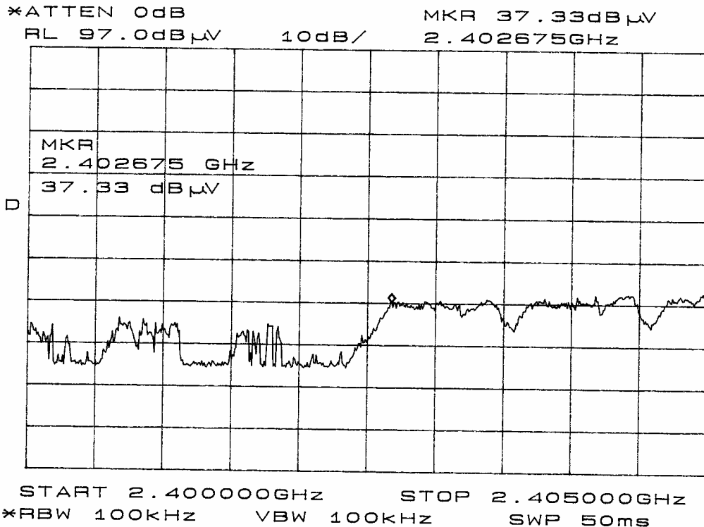
Figure Eleven Operation at Frequency Band Edge
