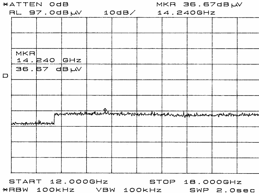
Figure Eight Radiated Emissions Plot
