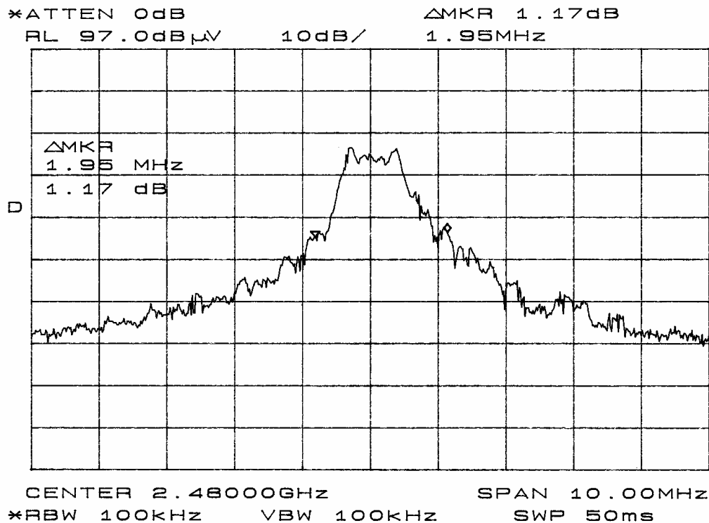
Figure Nine Occupied Bandwidth
