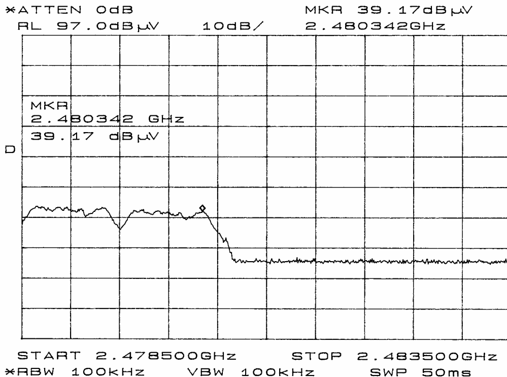
Figure Twelve Operation at Frequency Band Edge
