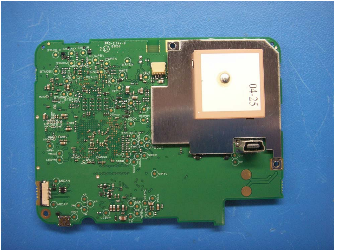
Figure 2: Bottom View with Shields
