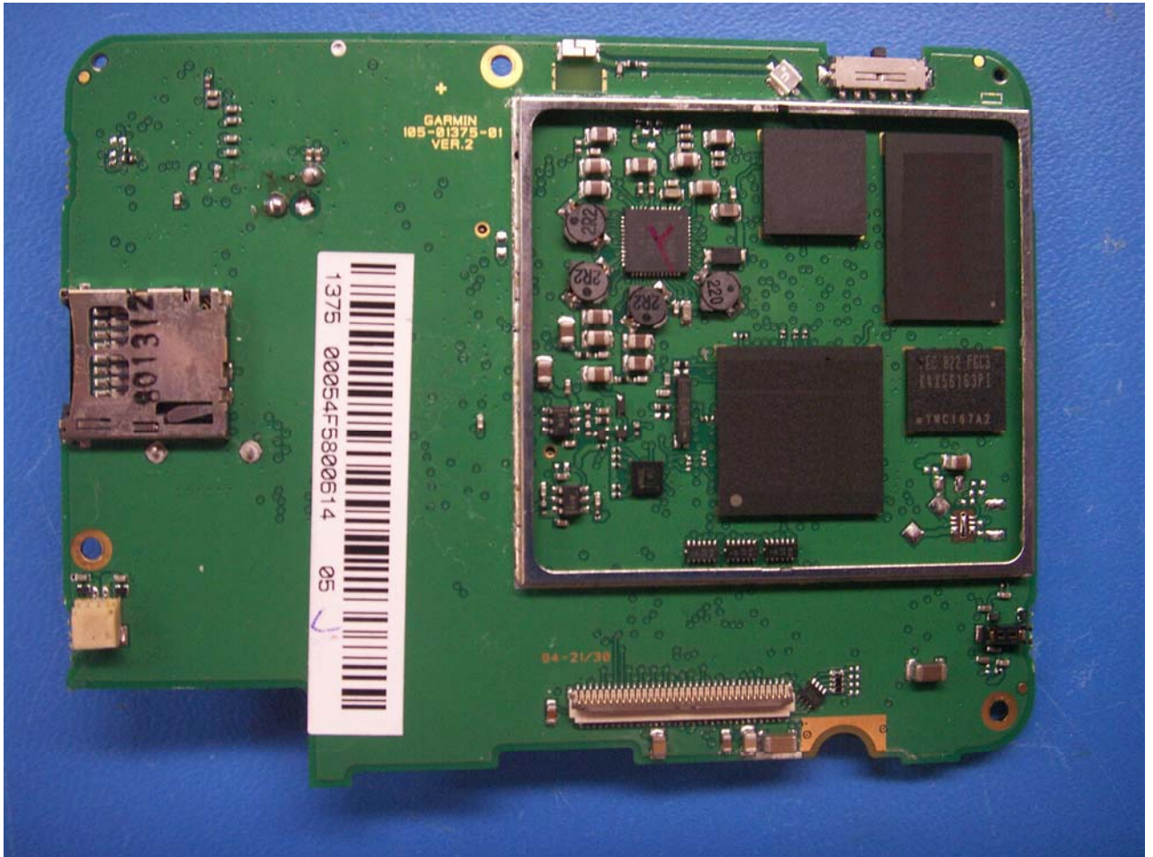
Figure 3: Top View without Shields
