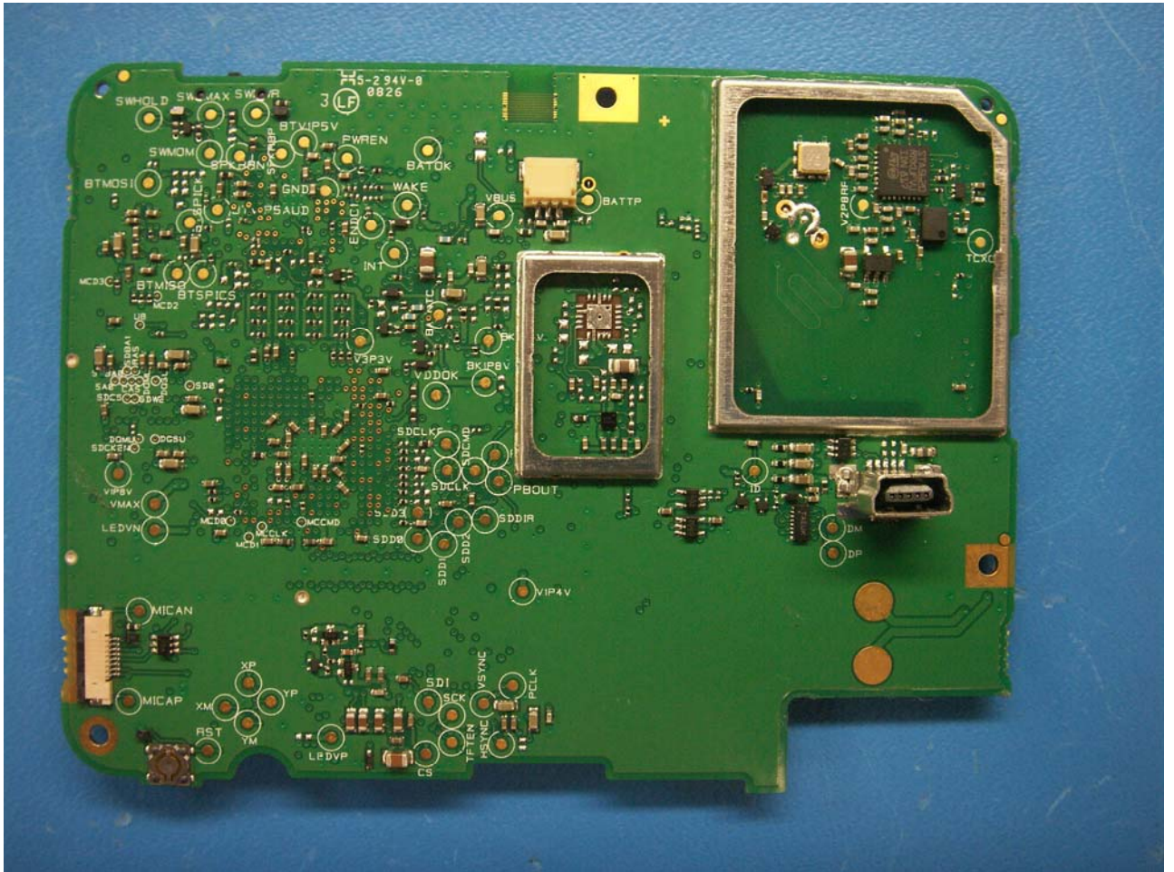
Figure 4: Bottom View without Shields
