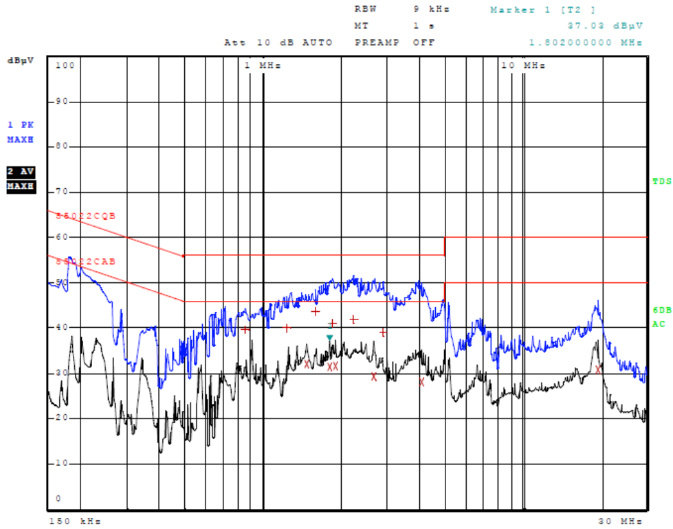
Figure Three AC Line Conducted emissions of EUT line 1 (EUT USB to CPU)
