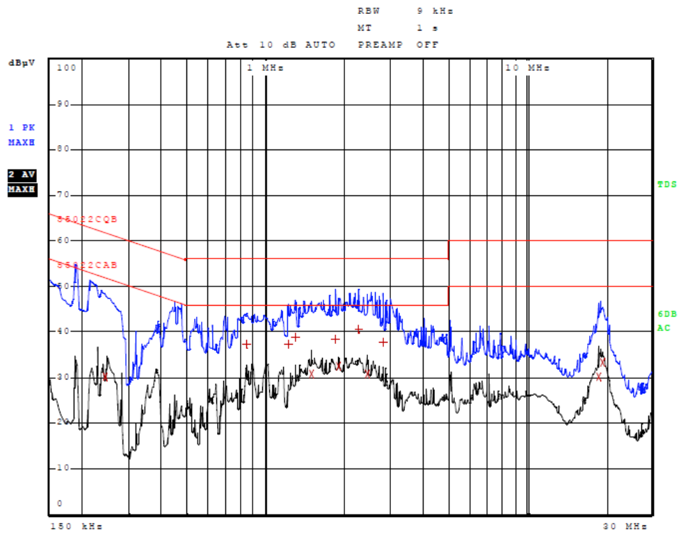
Figure Four AC Line Conducted emissions of EUT line 2 (EUT USB to CPU)
